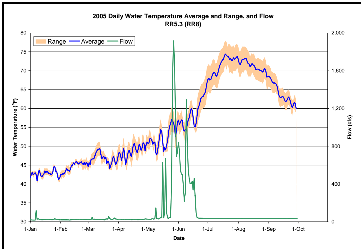
Figure A-71. The daily water temperature average and range measured at RR5.3 and the sum of flow measured at USGS # 11428800 (Rubicon below Hell Hole) and # 11430000 (SF Rubicon below Gerle Cr) during 2005
