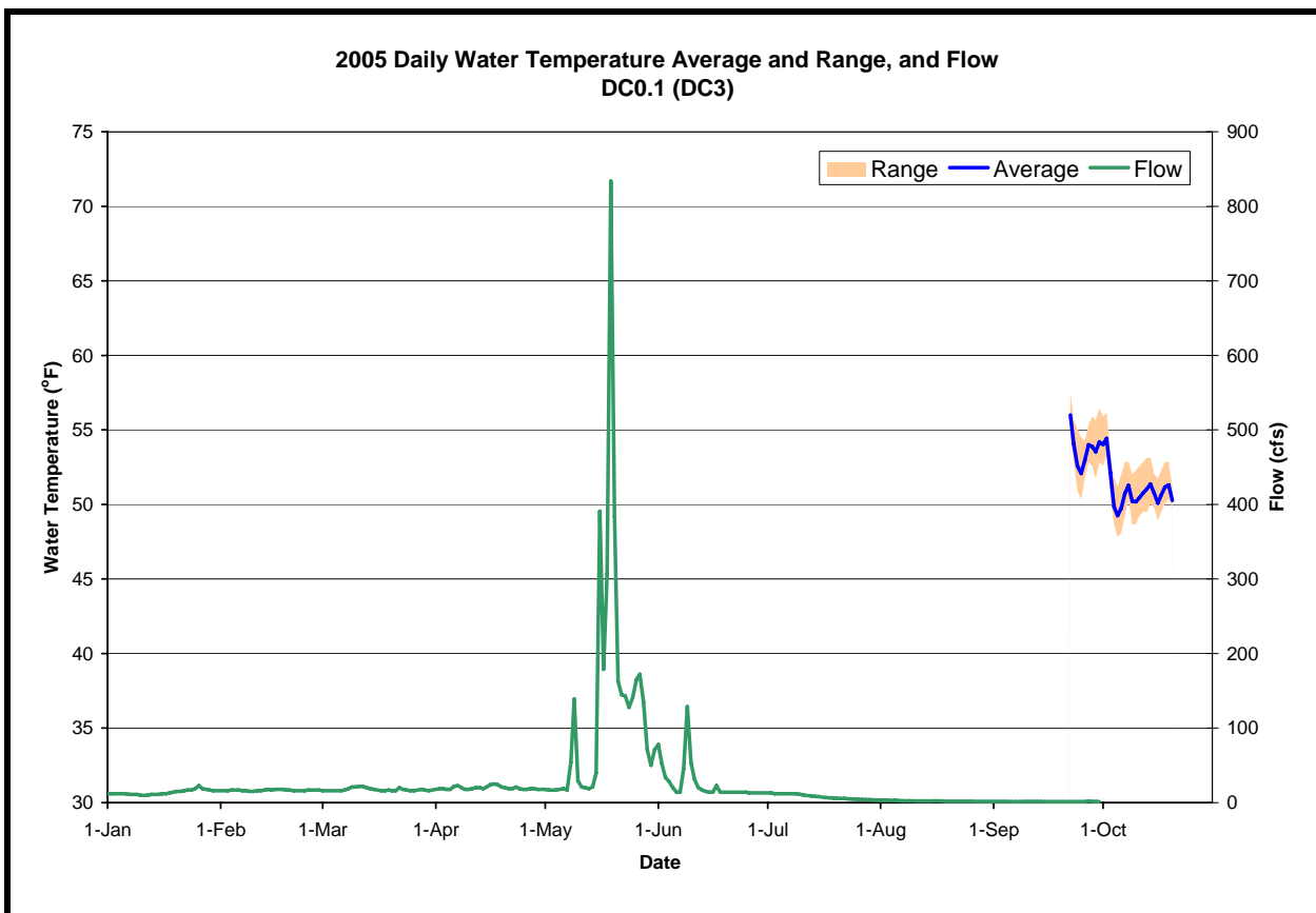
Figure A-5. The daily water temperature average and range measured at DC0.1 and flow measured at USGS # 11427750 (Duncan Cr below diversion) during 2005.
