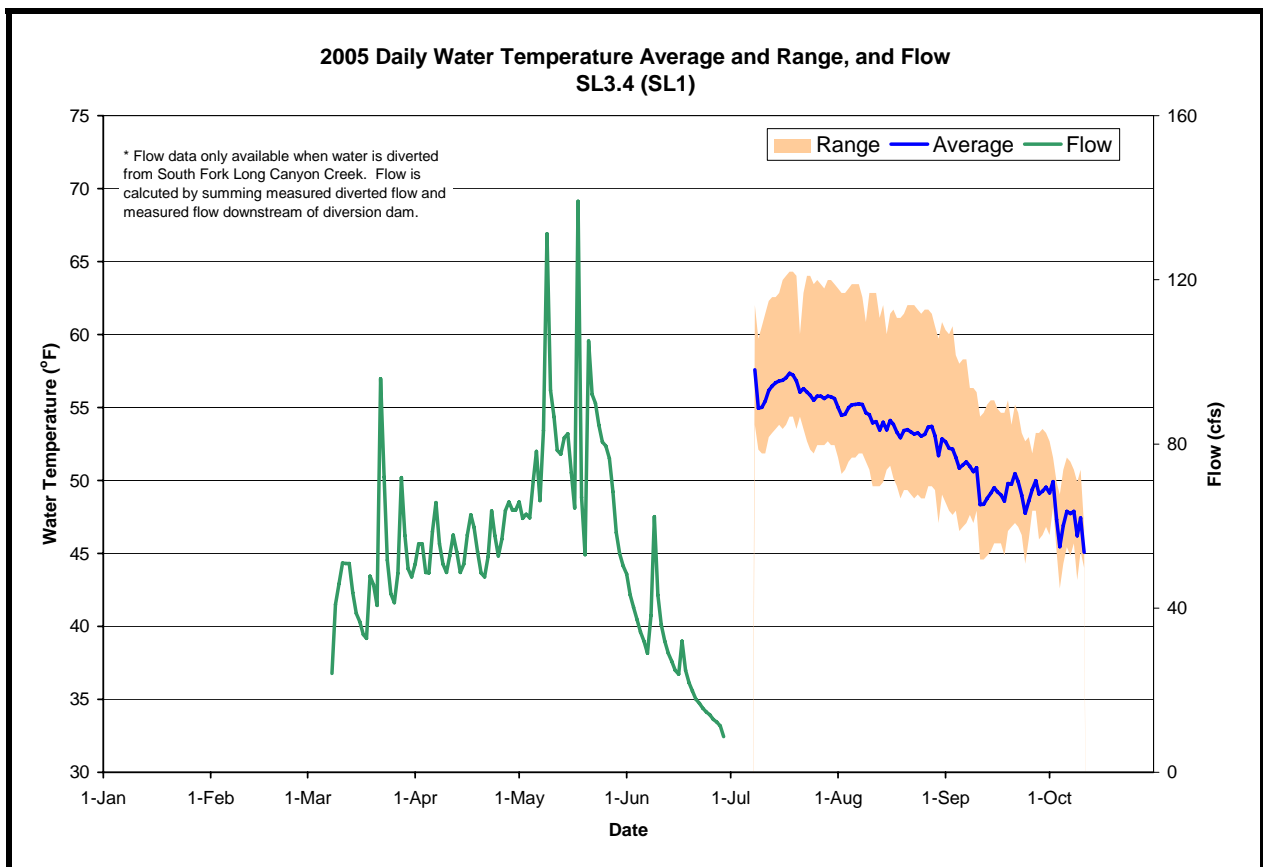
Figure A-81. The daily water temperature average and range measured at SL3.4 and the sum of flow measured at USGS # 11433060 (SF Long Canyon Diversion Tunnel) and # 11433065 (SF Long Canyon below diversion) during 2005. [Note: flows are only measured in South Fork Long Canyon Creek when flows are diverted, which typically occurs between late winter and spring. Consequently, flow data are not available during the summer]
