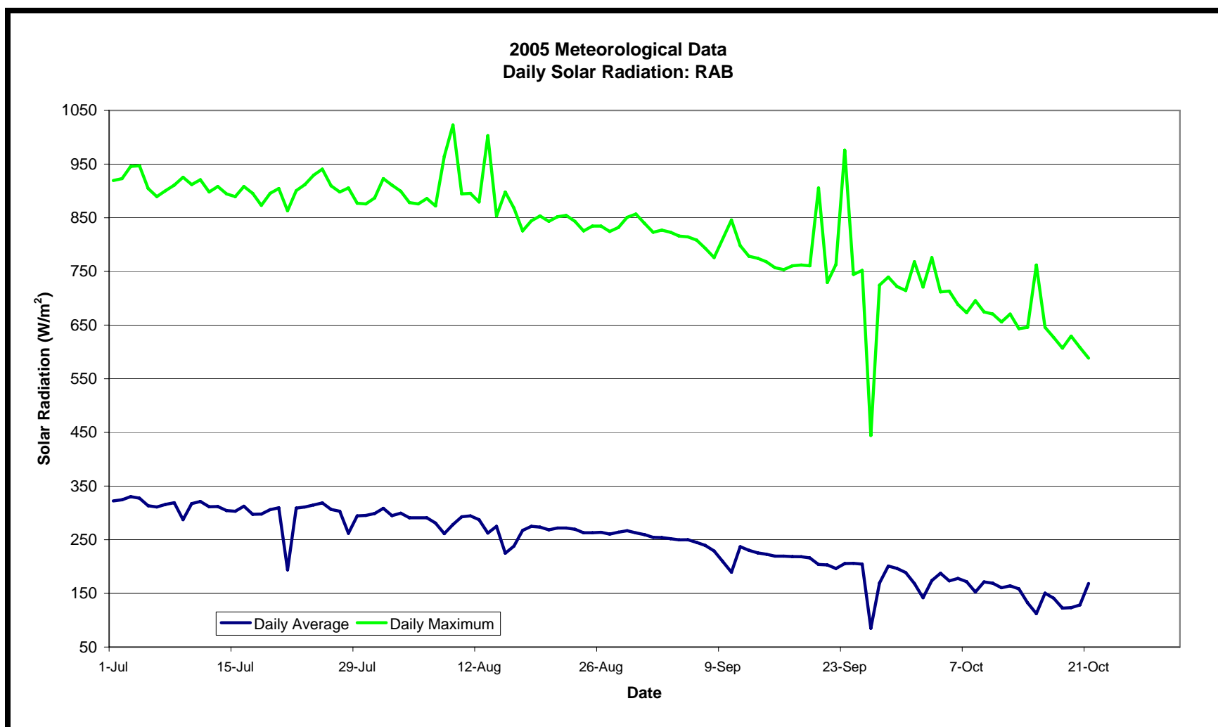
Figure 48. The daily Average and Maximum Solar Radiation (watts/meter squared (W/m 2 )) at Ralston Afterbay Dam Collected During the Summer and Fall of 2005.
