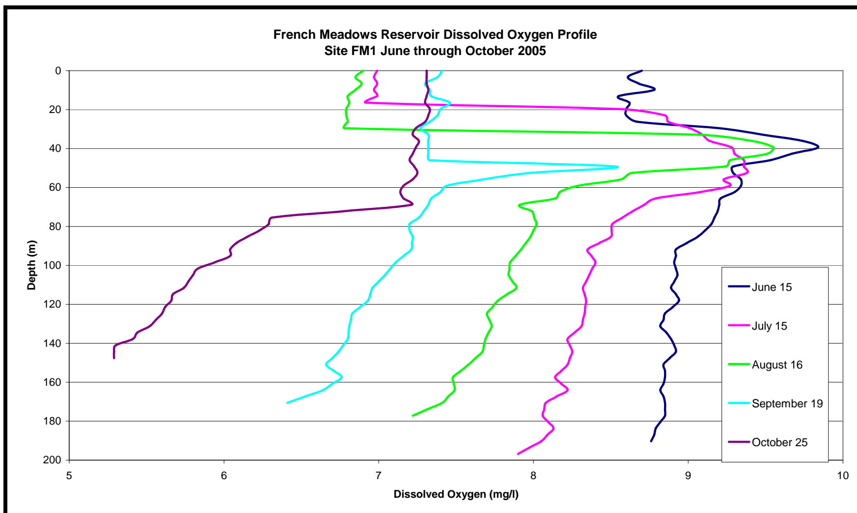
Figure 26. The French Meadows Reservoir Dissolved Oxygen Profiles at Site FM1 (Nearest French Meadows Dam) on June 15, July 15, August 16, September 19, and October 25, 2005.
