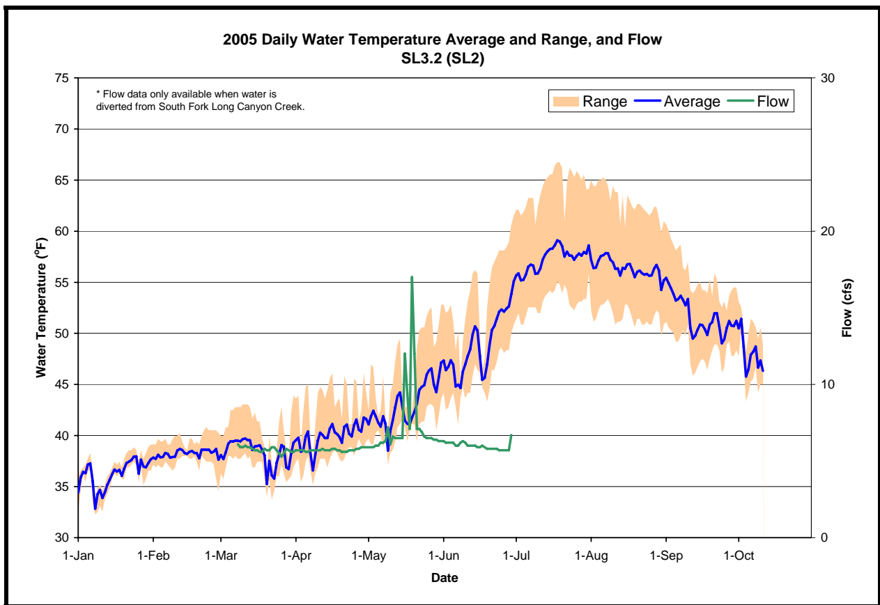
Figure A-83. The daily water temperature average and range measured at SL3.2 and flow measured at USGS # 11433065 (SF Long Canyon below diversion) during 2005. [Note: flows are only measured in South Fork Long Canyon Creek when flows are diverted, which typically occurs between late winter and spring. Consequently, flow data are not available during the summer]
