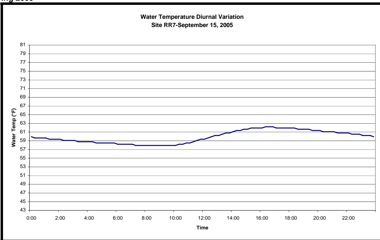
Figure A-70. The 15-minute interval water temperature data observed at RR7 during a particularly warm day in September to illustrate diurnal variation
