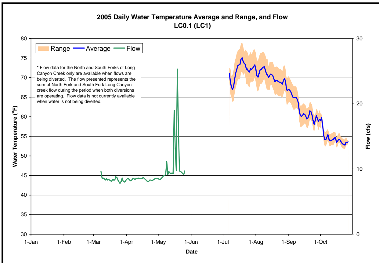
Figure A-11. The daily water temperature average and range measured at LC0.1 and the sum of flow measured at USGS # 11433065 (SF Long Canyon below diversion) and # 11433085 (NF Long Canyon below diversion) during 2005. [Note: flows are only measured in North Fork and South Fork Long Canyon creeks when flows are diverted, which typically occurs between late winter and spring. Consequently, flow data are not available during the summer]
