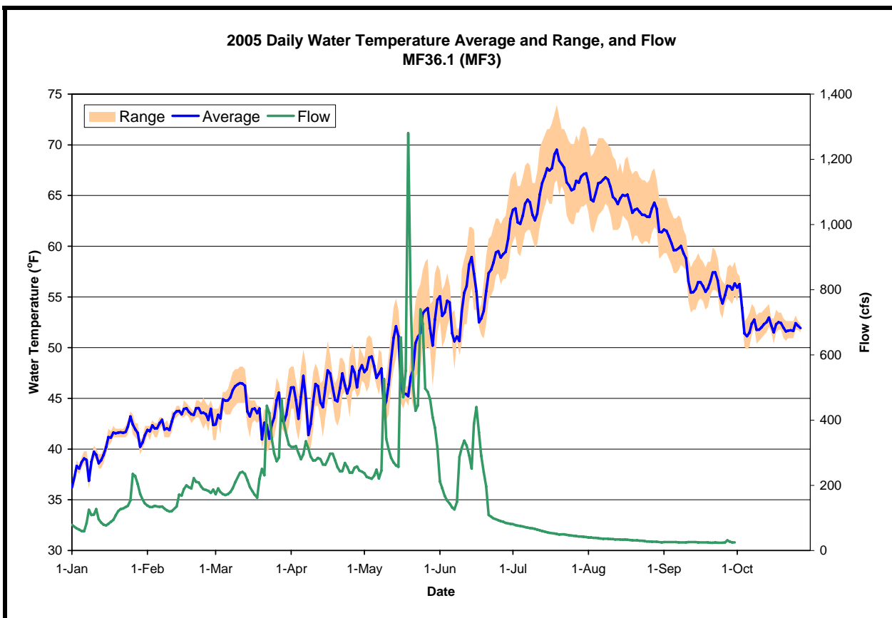
Figure A-21. The daily water temperature average and range measured at MF36.1 and flow measured at USGS # 11427760 (MF American above MF Powerhouse) during 2005
