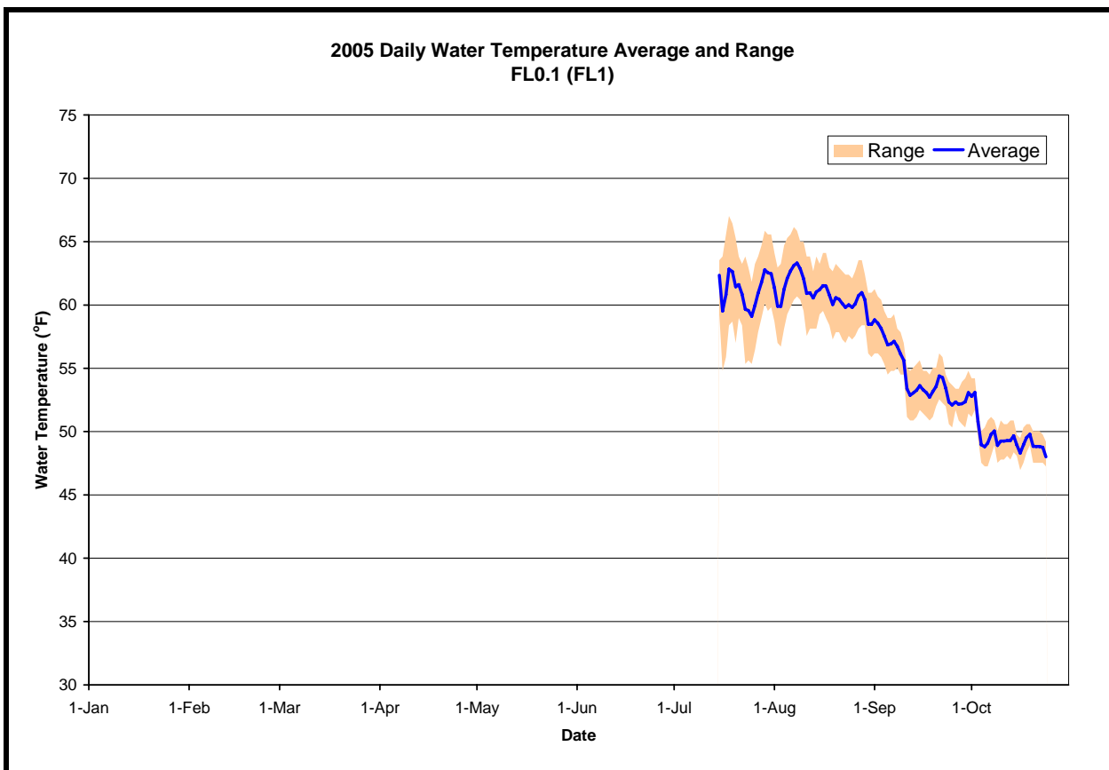
Figure A-7. The daily water temperature average and range measured at FL0.1 during 2005. USGS flow data are not available near this site.
