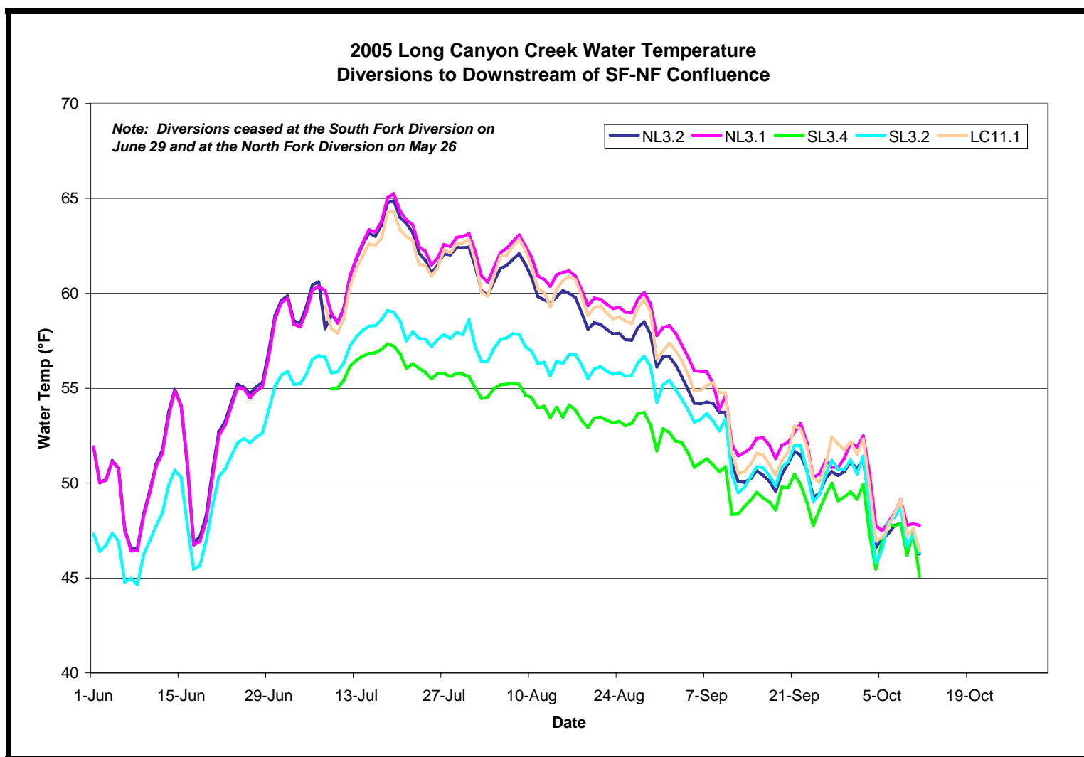
Figure 16. Summer and Fall Daily Average Water Temperature Data Collected in Long Canyon Creek at Sites NL3.2, NL3.1, SL3.4, SL3.2, and LC11.1. Refer to Figures 3-5 for the Relative Site Locations. [Note: The differences in the durations of the water temperature observations are due to differences in site installation and final download dates].
