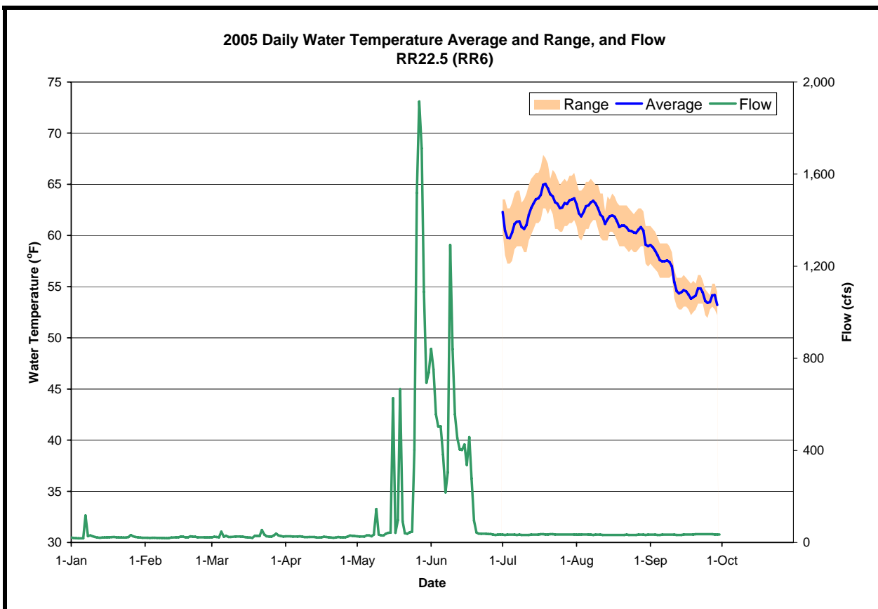
Figure A-67. The daily water temperature average and range measured at RR22.5 and the sum of flow measured at USGS # 11428800 (Rubicon below Hell Hole) and # 11430000 (SF Rubicon below Gerle Cr) during 2005
