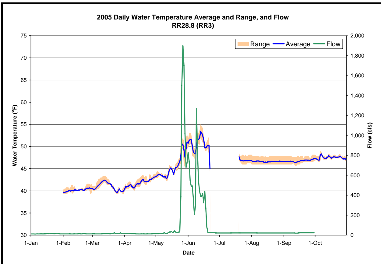
Figure A-61. The daily water temperature average and range measured at RR28.8 and flow measured at USGS # 11428800 (Rubicon below Hell Hole) during 2005
