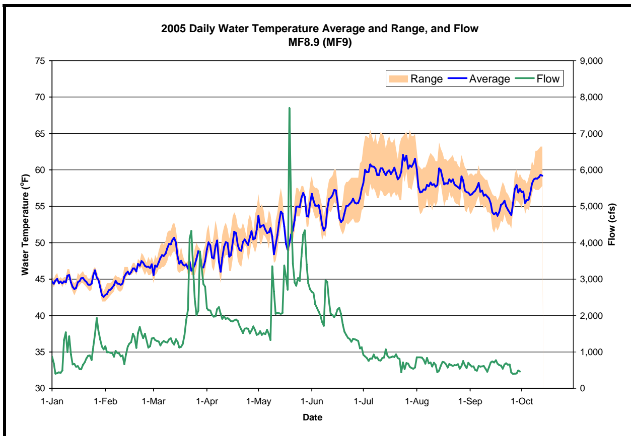
Figure A-33. The daily water temperature average and range measured at MF8.9 and flow measured at USGS # 11433300 (MF American near Foresthill) during 2005.
