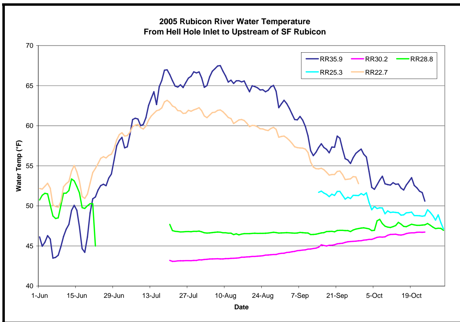
Figure 13. Summer and Fall Daily Average Water Temperature Data Collected in the Rubicon River at Sites RR35.9, RR30.2, RR28.8, RR25.3, and RR22.7. Refer to Figures 3-5 for the Relative Site Locations. [Note: The differences in the durations of the water temperature observations are due to differences in site installation and final download dates].
