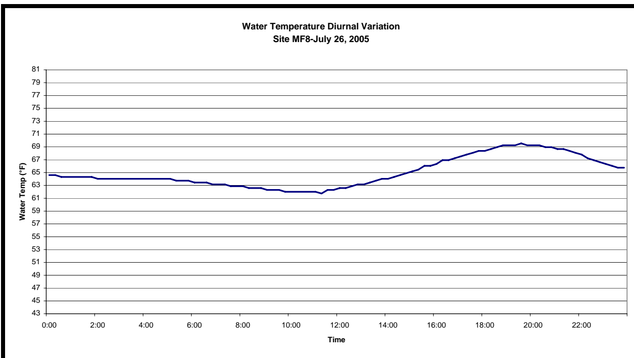
Figure A-32. The 15-minute interval water temperature data observed at MF8 during a particularly warm day in July to illustrate diurnal variation
