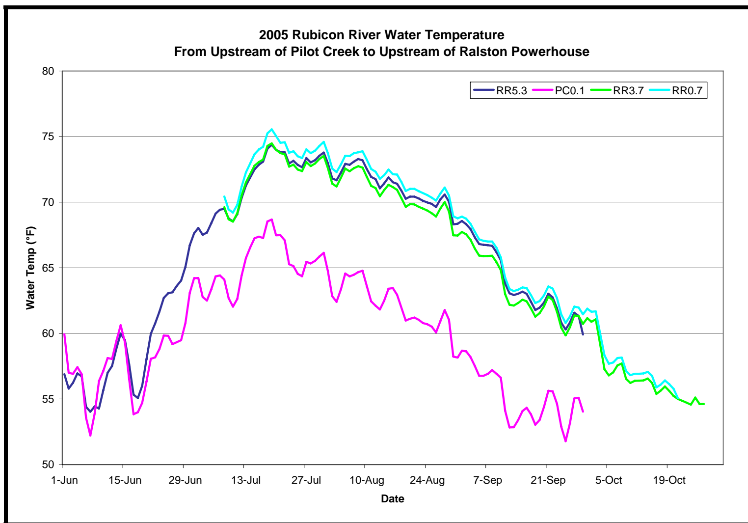
Figure 15. Summer and Fall Daily Average Water Temperature Data Collected in the Rubicon River at Sites RR5.3, PC0.1, RR3.7, and RR0.7. Refer to Figures 3-5 for the Relative Site Locations. [Note: The differences in the durations of the water temperature observations are due to differences in site installation and final download dates].
