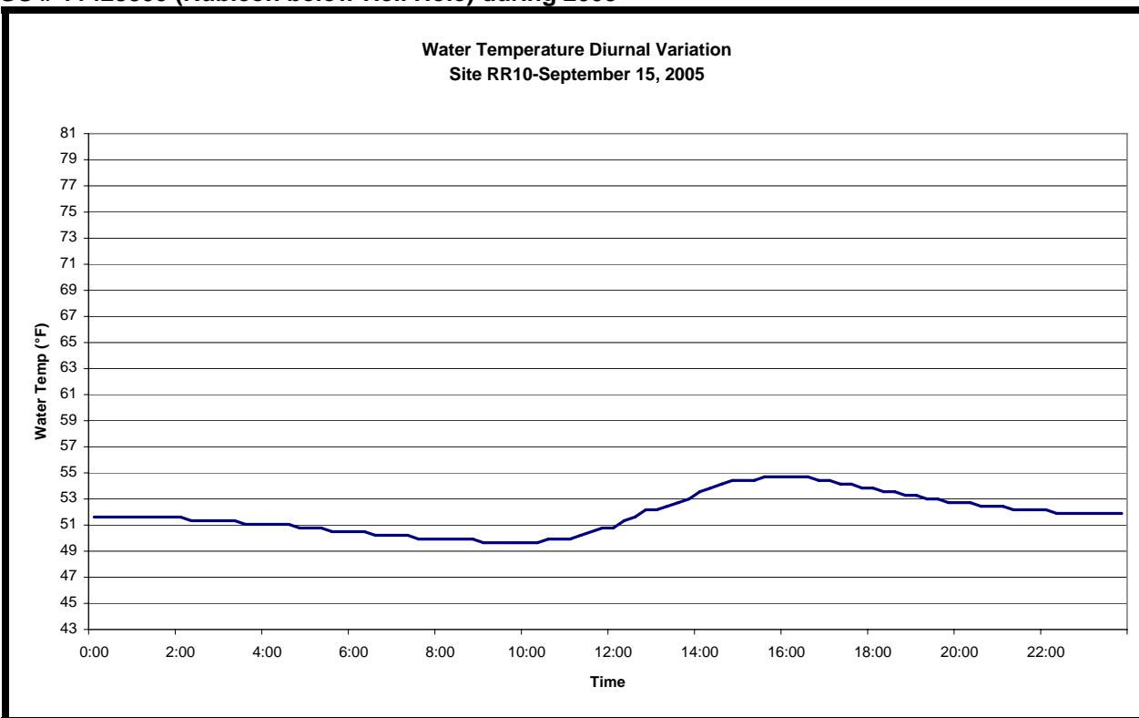
Figure A-76. The 15-minute interval water temperature data observed at RR10 during a particularly warm day in September to illustrate diurnal variation
