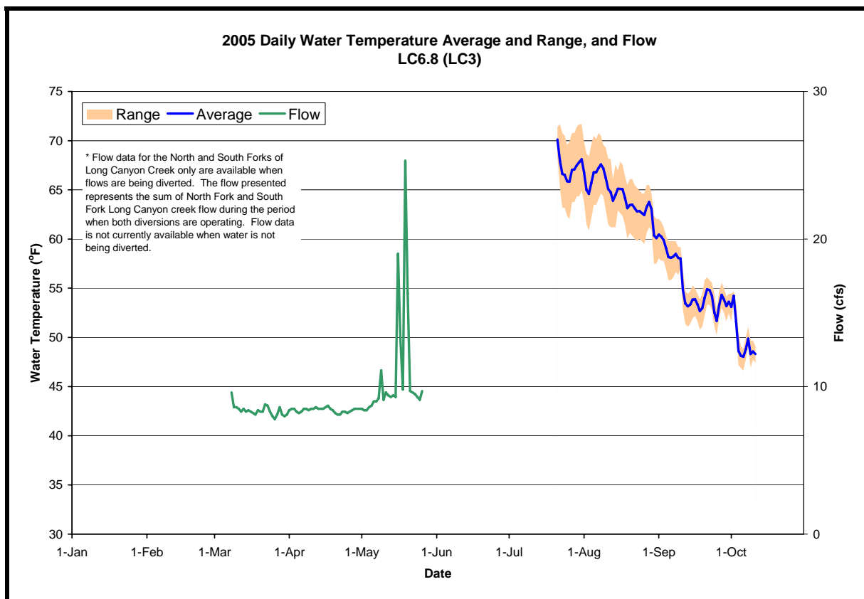
Figure A-15. The daily water temperature average and range measured at LC6.8 and the sum of flow measured at USGS # 11433065 (SF Long Canyon below diversion) and # 11433085 (NF Long Canyon below diversion) during 2005. [Note: flows are only measured in North Fork and South Fork Long Canyon creeks when flows are diverted, which typically occurs between late winter and spring. Consequently, flow data are not available during the summer]
