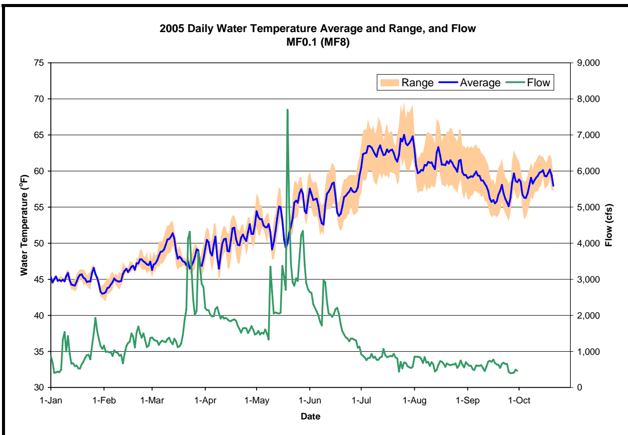
Figure A-31. The daily water temperature average and range measured at MF0.1 and flow measured at USGS # 11433300 (MF American near Foresthill) during 2005
