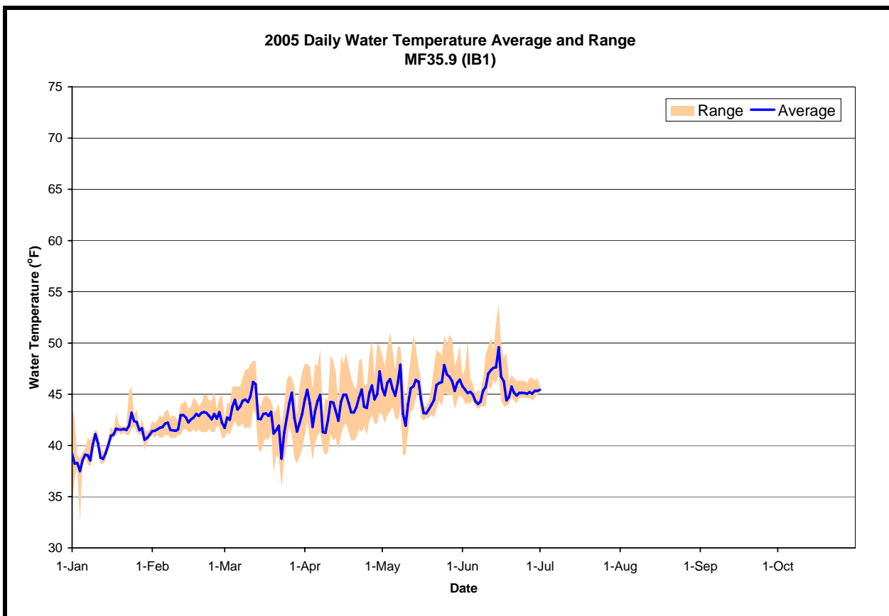
Figure A-9. The daily water temperature average and range measured at MF35.9 during 2005. USGS flow data are not available near this site
