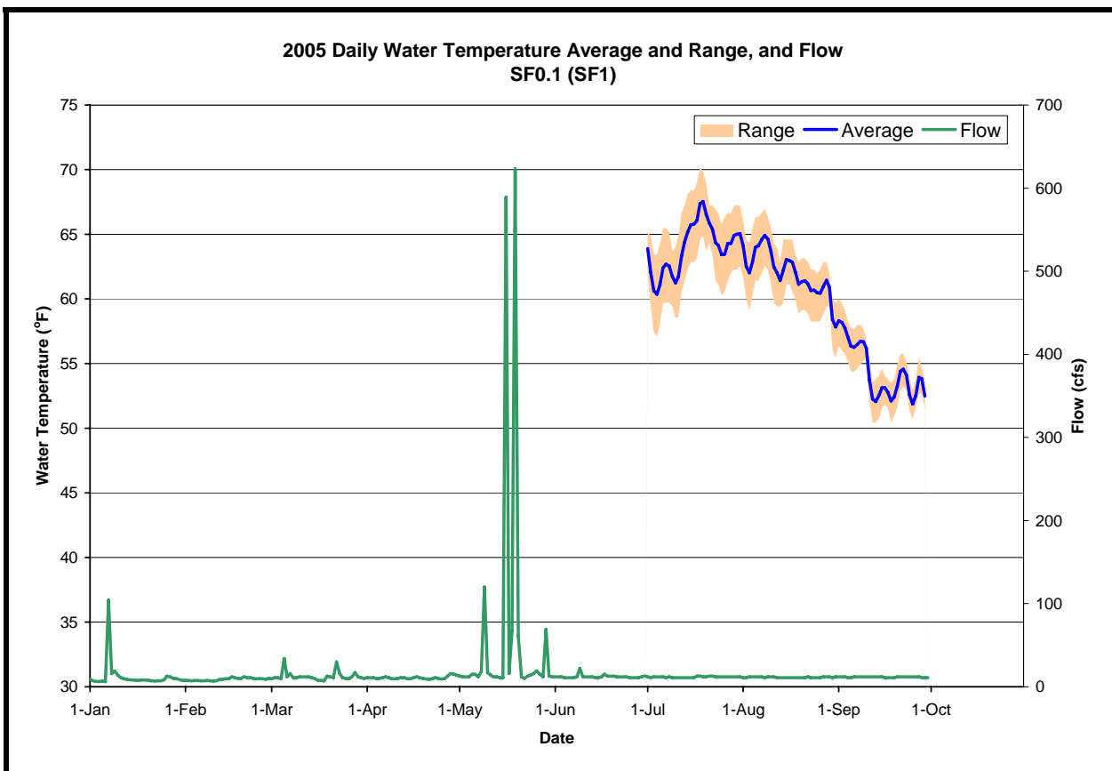
Figure A-79. The daily water temperature average and range measured at SF0.1 and flow measured at USGS # 11430000 (SF Rubicon below Gerle Cr) during 2005
