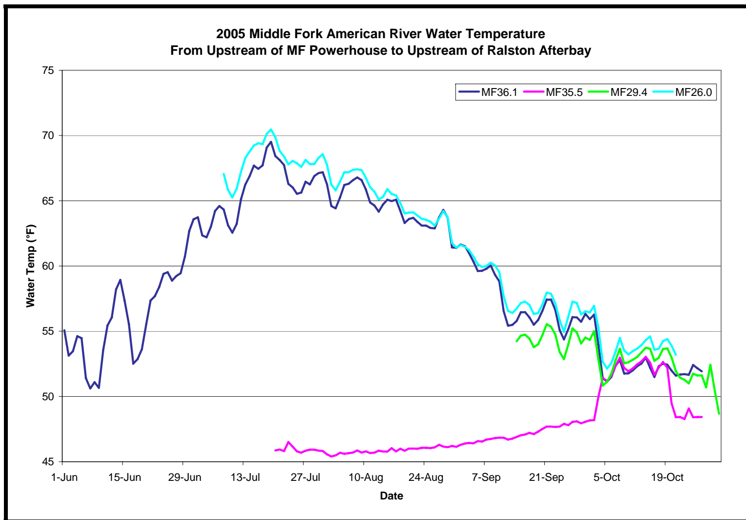
Figure 10. Summer and Fall Daily Average Water Temperature Data Collected in the Middle Fork American River at Sites MF36.1, MF35.5, MF29.4, and MF26.0. Refer to Figures 3-5 for the Relative Site Locations. [Note: The differences in the durations of the water temperature observations are due to differences in site installation and final download dates].
