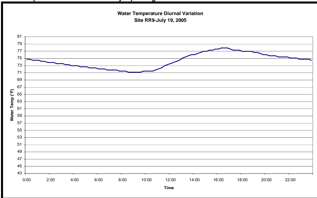
Figure A-74. The 15-minute interval water temperature data observed at RR9 during a particularly warm day in July to illustrate diurnal variation
