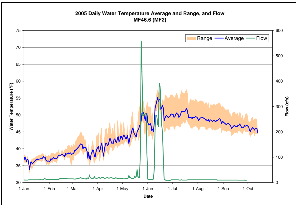
Figure A-19. The daily water temperature average and range measured at MF46.6 and flow measured at USGS # 11427500 (MF American below French Meadows) during 2005.
