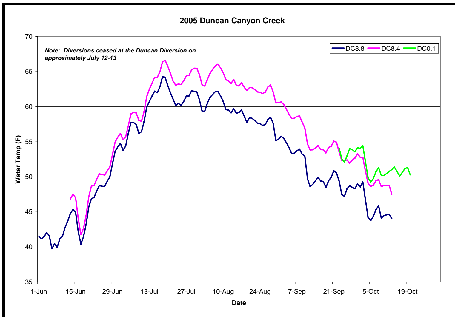
Figure 12. Summer and Fall Daily Average Water Temperature Data collected in Duncan Canyon Creek at Sites DC8.8, DC8.4, and DC0.1. Refer to Figures 3-5 for the Relative Site Locations. [Note: The differences in the durations of the water temperature observations are due to differences in site installation and final download dates].
