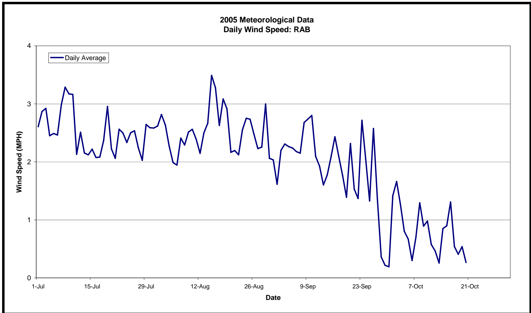
Figure 50. The Daily Average Wind Speed (miles per hour (mph)) at Ralston Afterbay Dam Collected During the Summer and Fall of 2005.
