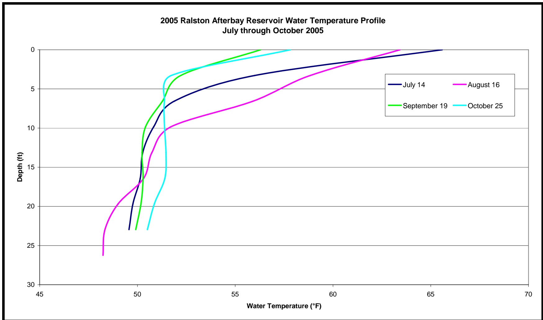
Figure 39. The Ralston Afterbay Reservoir Water Temperature Profiles on July 14, August 16, September 19, and October 25, 2005.
