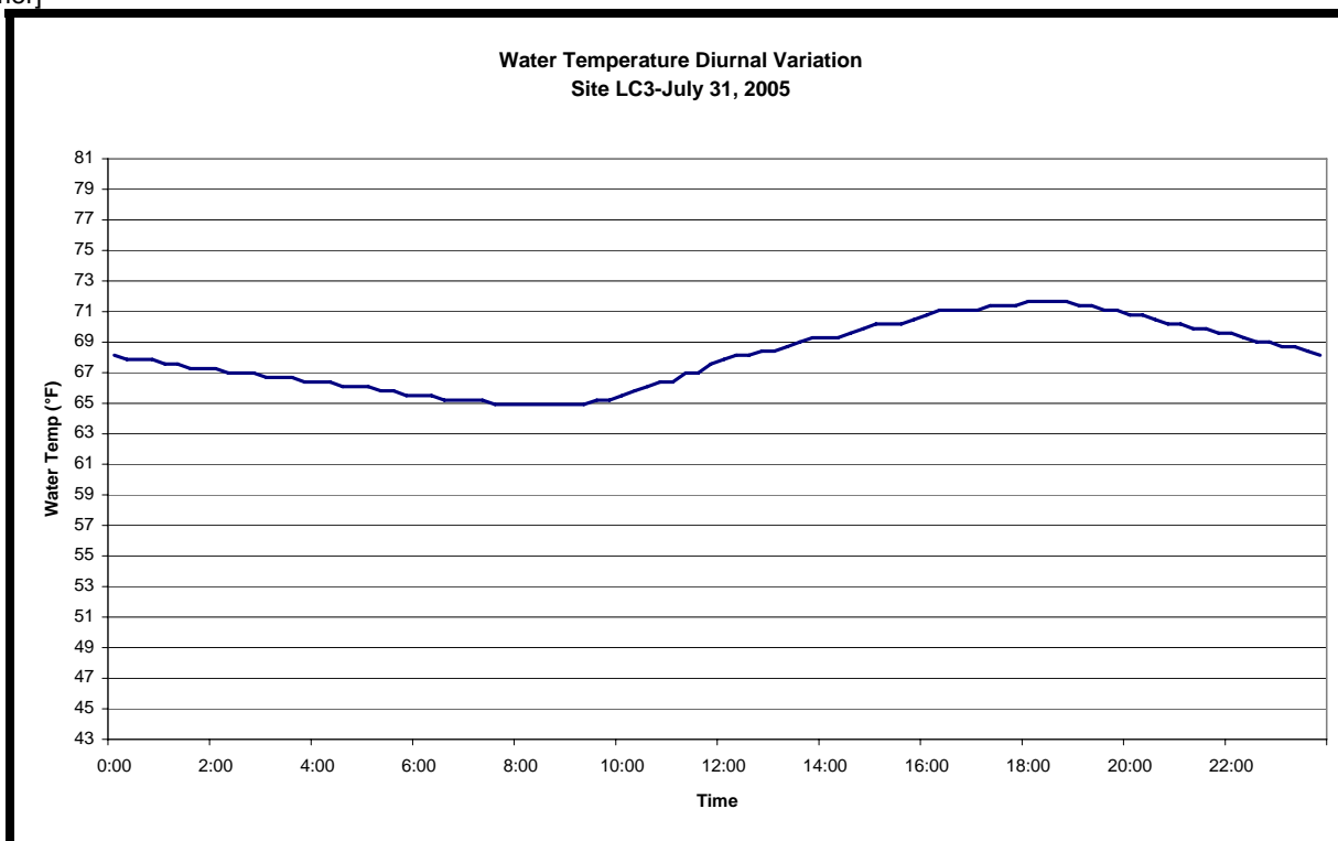
Figure A-16. The 15-minute interval water temperature data observed at LC3 during a particularly warm day in July to illustrate diurnal
