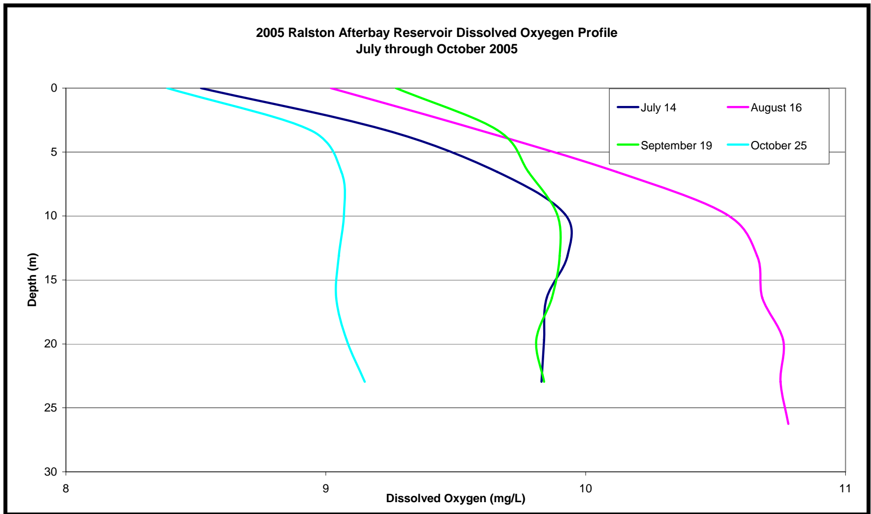
Figure 40. The Ralston Afterbay Reservoir Dissolved Oxygen Profiles from July 14, August 16, September 19, and October 25, 2005.
