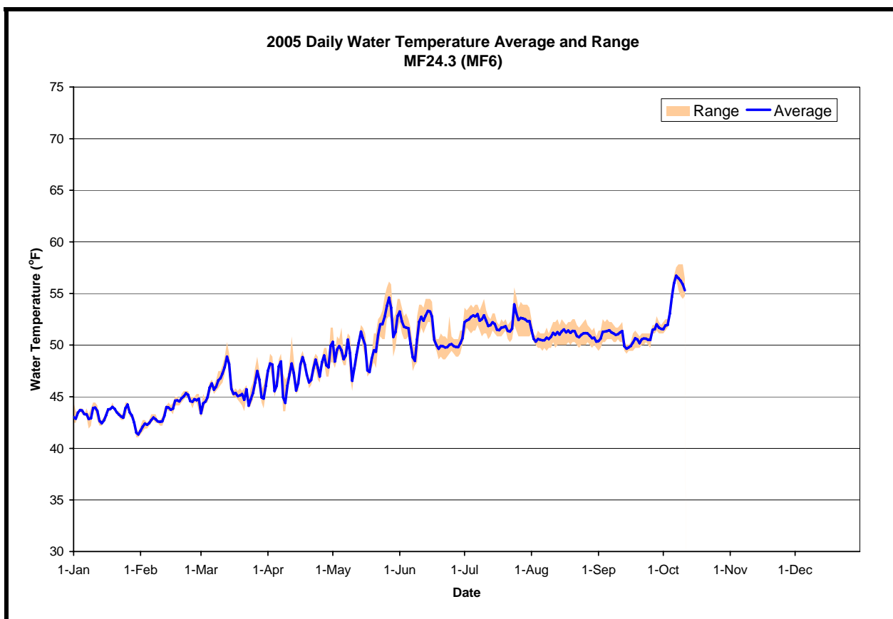
Figure A-27. The daily water temperature average and range measured at MF24.3 during 2005. USGS flow data are not available near this site
