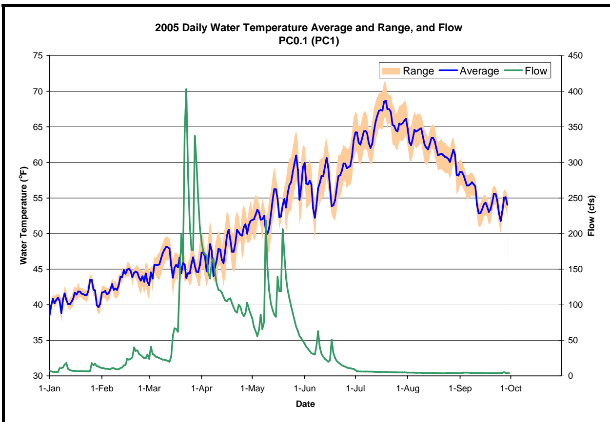
Figure A-55. The daily water temperature average and range measured at PC0.1 and flow measured at USGS # 11433040 (Pilot Cr below Mutton Canyon) during 2005
