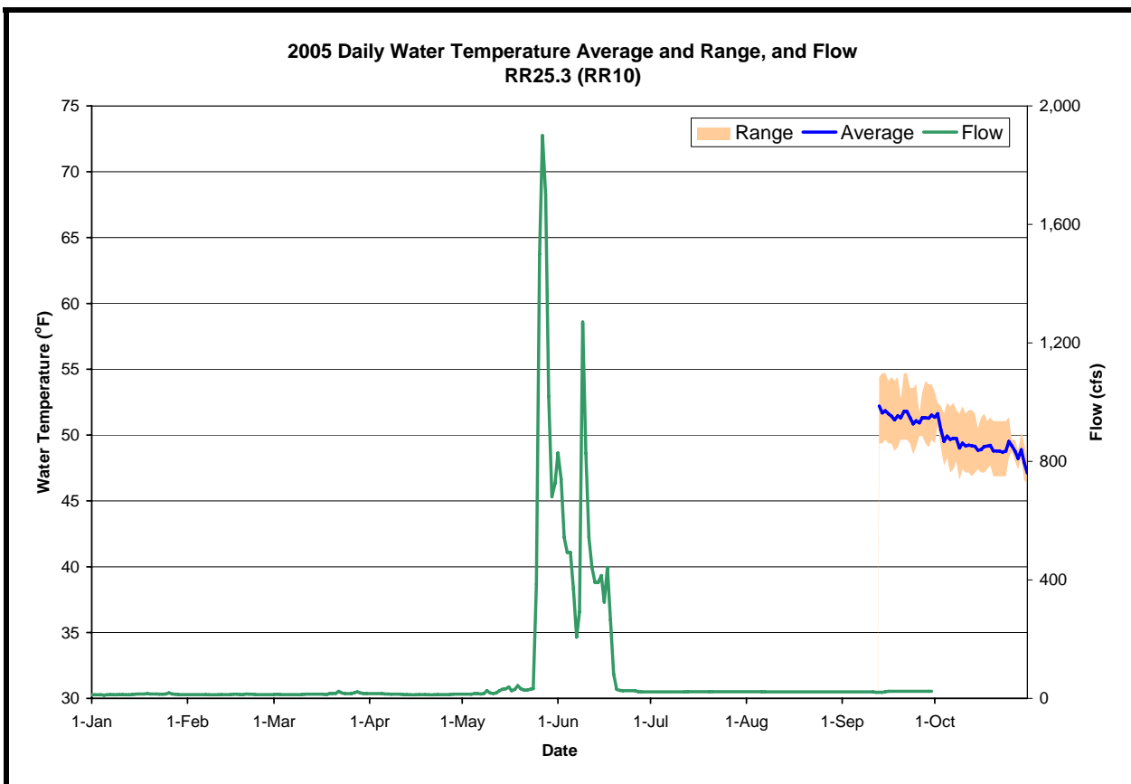
Figure A-75. The daily water temperature average and range measured at RR25.3 and flow measured at USGS # 11428800 (Rubicon below Hell Hole) during 2005
