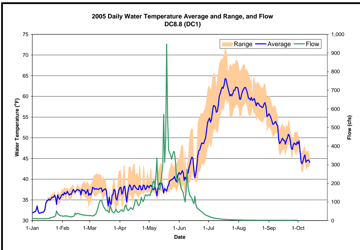
Figure A-1. The daily water temperature average and range measured at DC1 during 2005.
