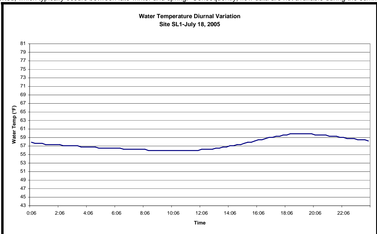
Figure A-82. The 15-minute interval water temperature data observed at SL1 during a particularly warm day in July to illustrate diurnal variation
