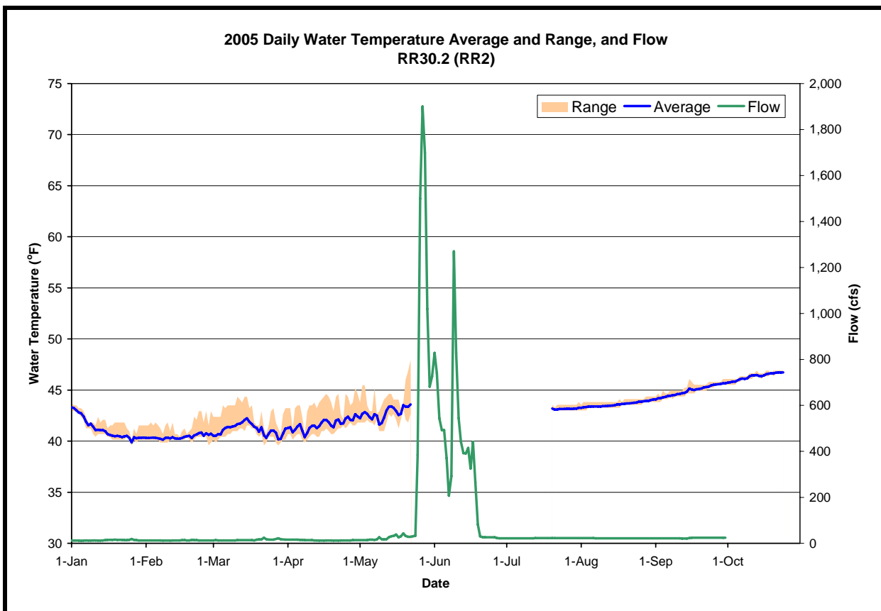
Figure A-59. The daily water temperature average and range measured at RR30.2 and flow measured at USGS # 11428800 (Rubicon below Hell Hole) during 2005
