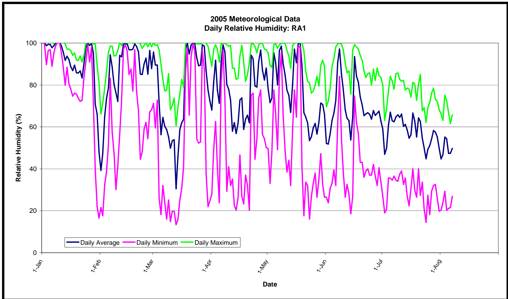
Figure 56. The Daily Average, Maximum, and Minimum Relative Humidity (%) at the Rubicon River Near Ellicott Bridge Collected During January through Early August 2005.
