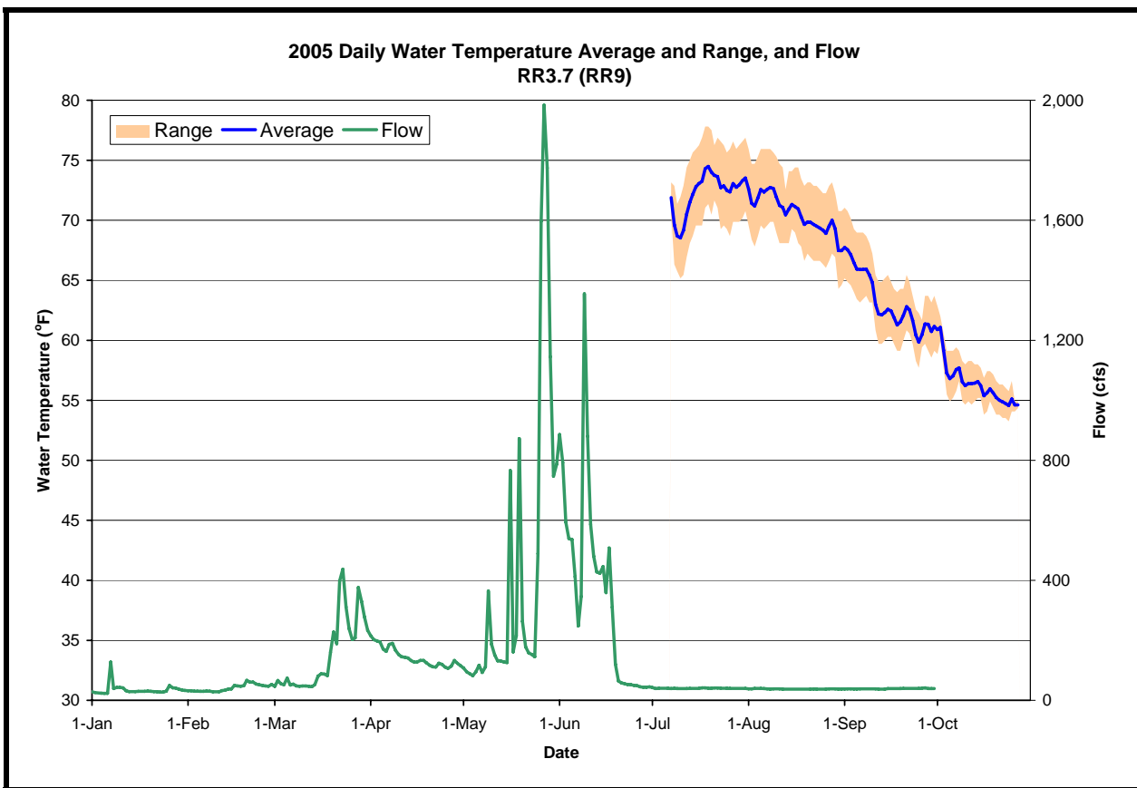
Figure A-73. The daily water temperature average and range measured at RR3.7 and the sum of flow measured at USGS # 11428800 (Rubicon below Hell Hole), 11430000 (SF Rubicon below Gerle Cr), and 11433040 (Pilot Cr below Mutton Canyon) during 2005
