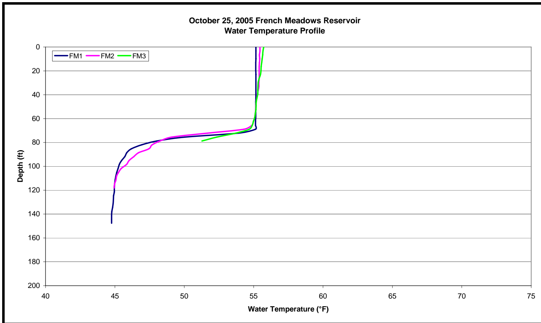
Figure 24. The French Meadows Reservoir Water Temperature Profiles at Sites FM1, FM2, and FM3 on October 25, 2005.
