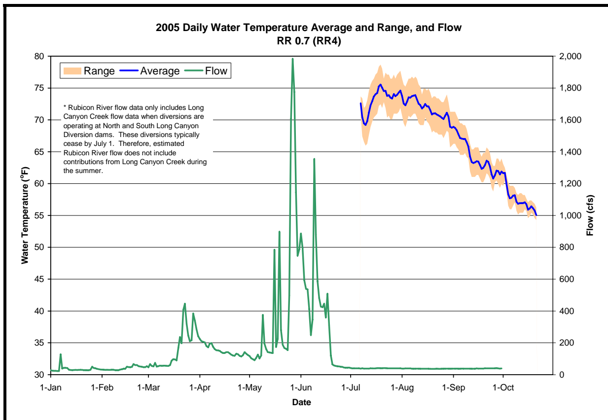
Figure A-63. The daily water temperature average and range measured at RR0.7 and the sum of flow measured at USGS # 11428800 (Rubicon below Hell Hole), 11430000 (SF Rubicon below Gerle Cr), 11433040 (Pilot Cr below Mutton Canyon), 11433065 (SF Long Canyon below diversion, when applicable), and 11433085 (NF Long Canyon below diversion, when applicable) during 2005
