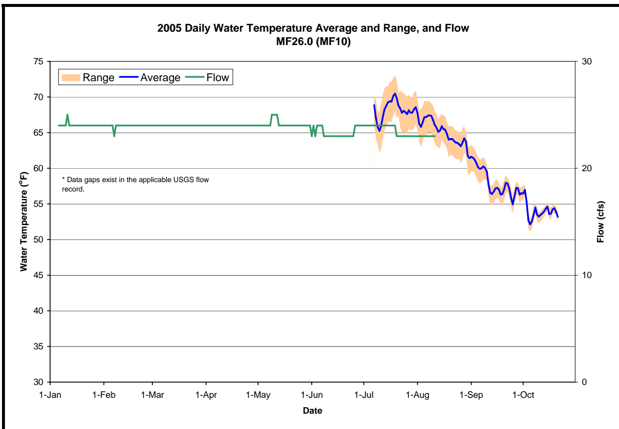
Figure A-35. The daily water temperature average and range measured at MF26.0 and flow measured at USGS # 11427770 (MF American below Interbay) during 2005.
