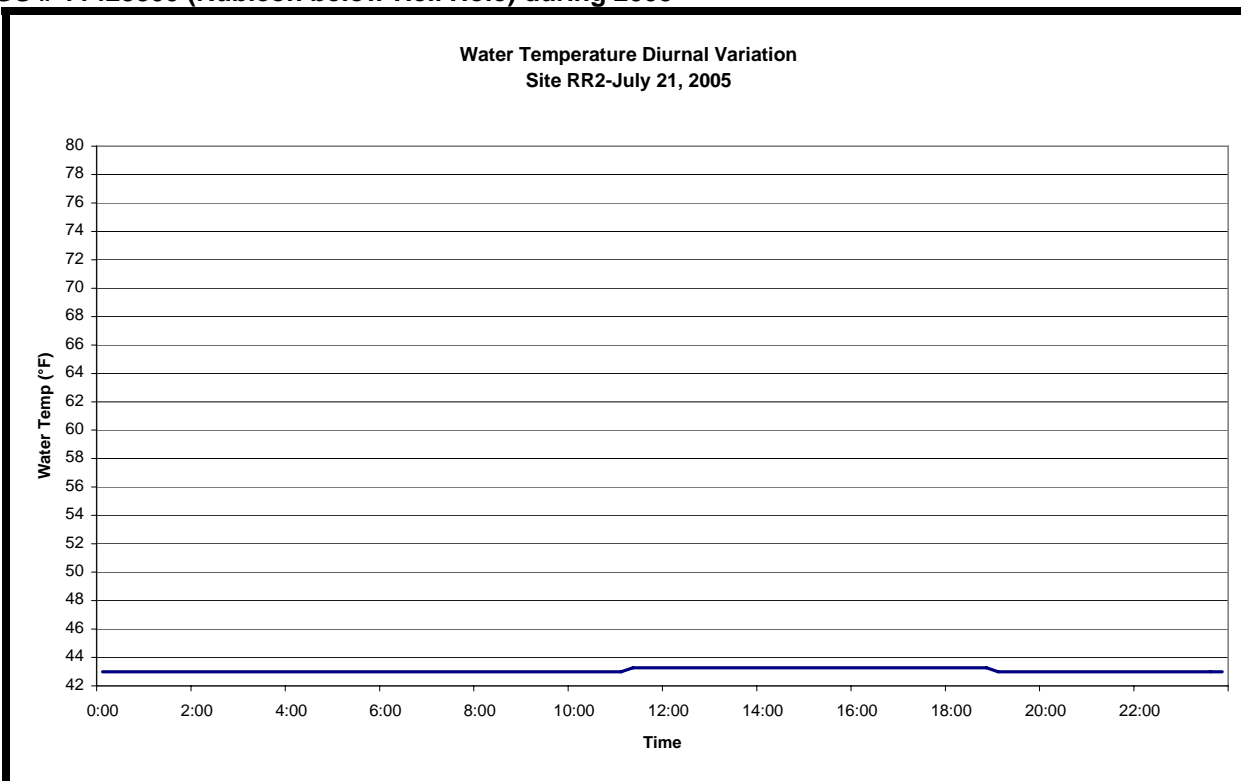
Figure A-60. The 15-minute interval water temperature data observed at RR2 during a particularly warm day in July to illustrate diurnal variation
