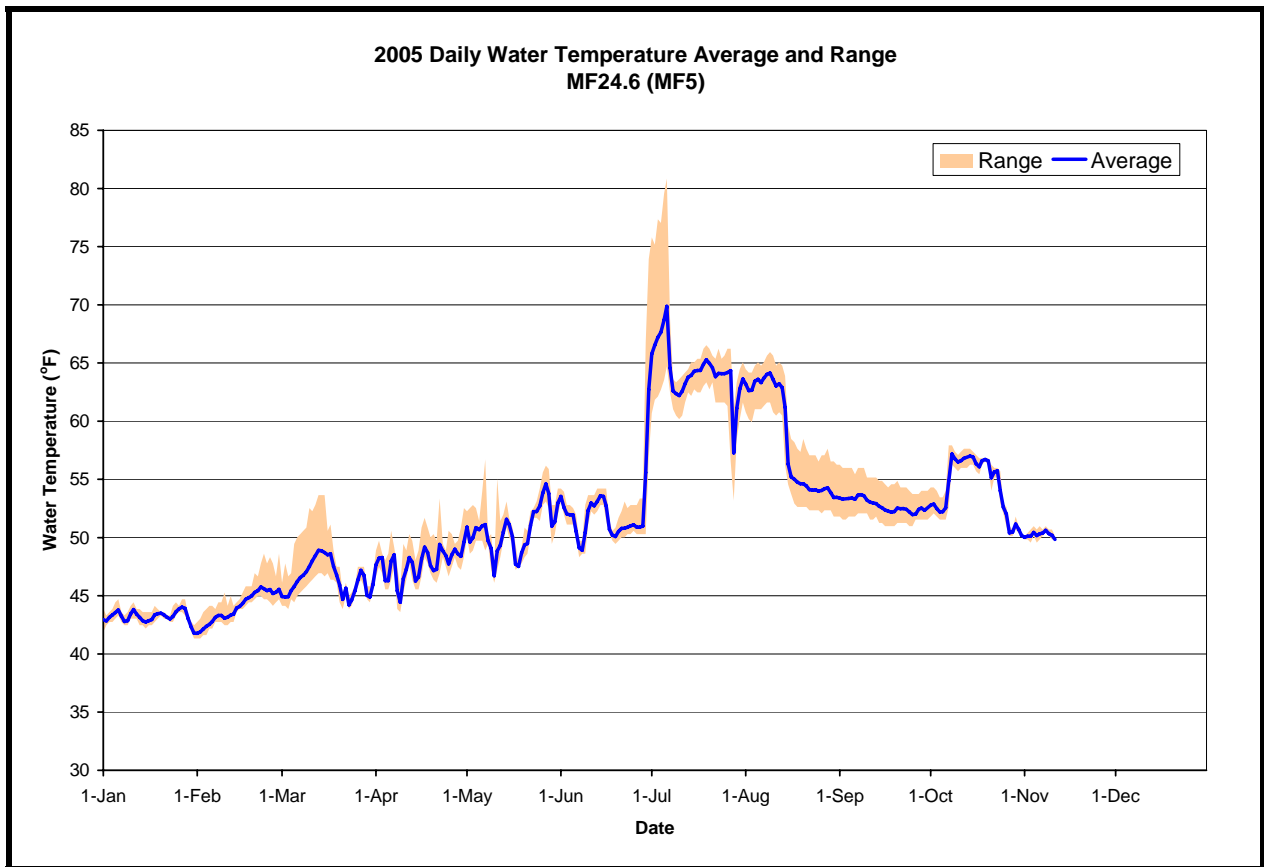
Figure A-25. The daily water temperature average and range measured at MF24.6 during 2005. USGS flow data are not available near this site
