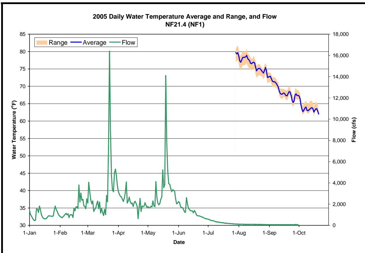
Figure A-43. The daily water temperature average and range measured at NF21.4 and flow measured at USGS # 11427000 (NF American below Clementine) during 2005
