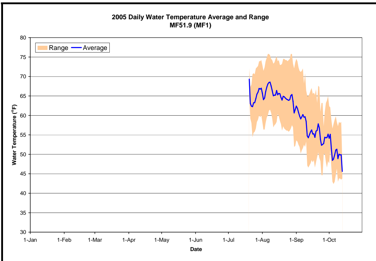
Figure A-17. The daily water temperature average and range measured at MF51.9 during 2005. USGS flow data are not available near this site
