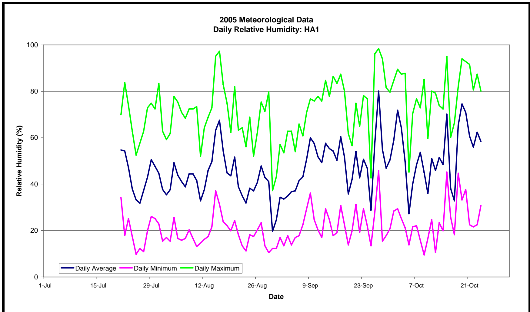
Figure 54. The Daily Average, Maximum, and Minimum Relative Humidity (%) at the Rubicon River Near Hell Hole Dam Collected During the Summer and Fall of 2005.
