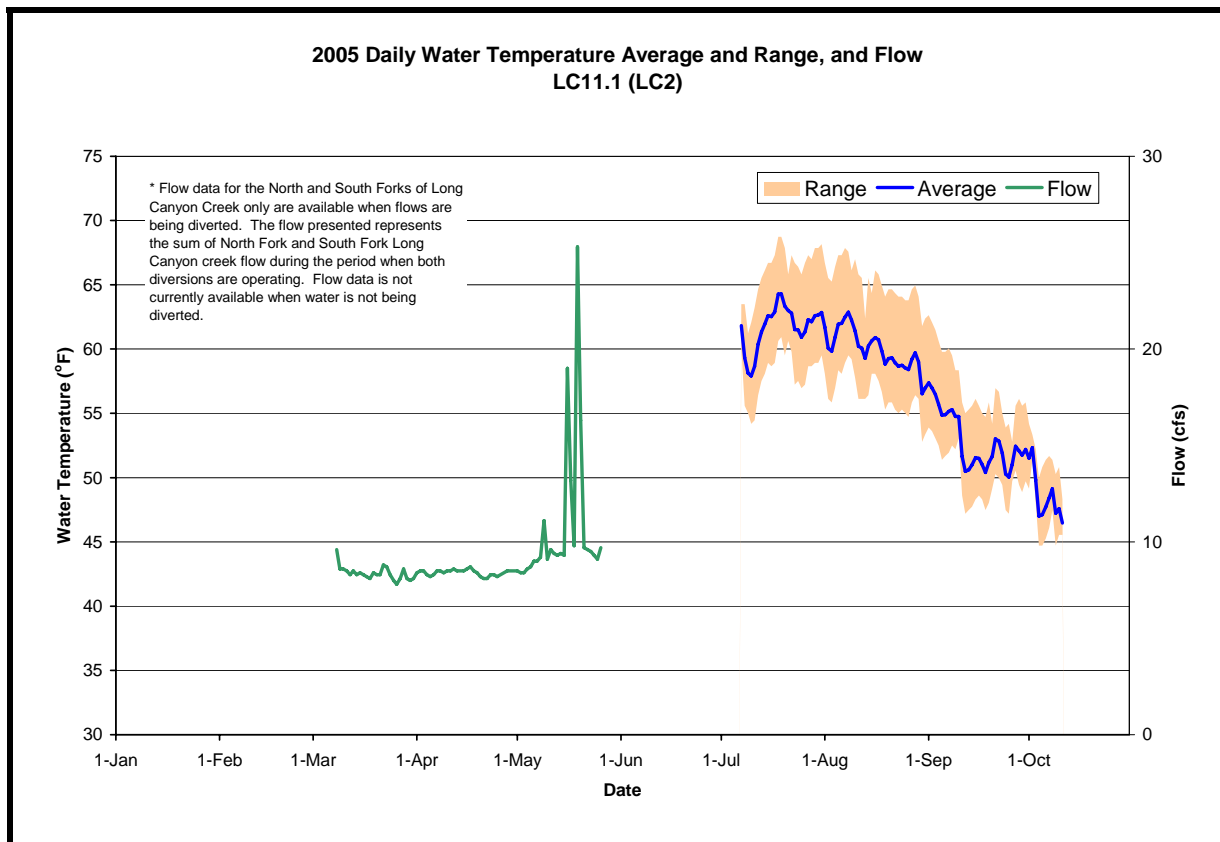
Figure A-13. The daily water temperature average and range measured at LC11.1 and the sum of flow measured at USGS # 11433065 (SF Long Canyon below diversion) and # 11433085 (NF Long Canyon below diversion) during 2005. [Note: flows are only measured in North Fork and South Fork Long Canyon creeks when flows are diverted, which typically occurs between late winter and spring. Consequently, flow data are not available during the summer]
