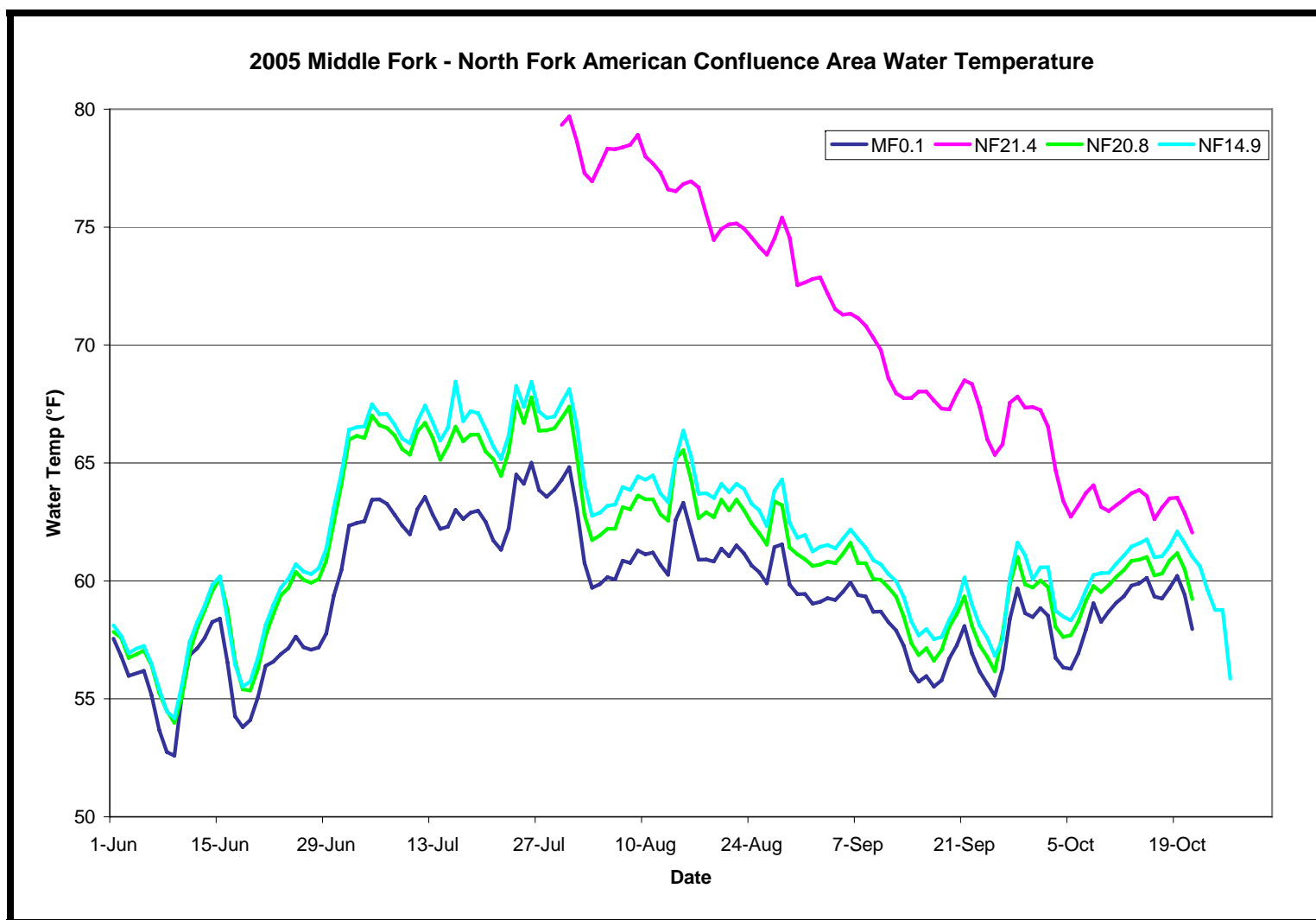
Figure 18. Summer and Fall Daily Average Water Temperature Data Collected in the North Fork American River (NF21.4, NF20.8, NF14.9) and in the Middle Fork American River Immediately Upstream of the North Fork American River Confluence (MF0.1). Refer to Figures 3-5 for the Relative Site Locations. [Note: The differences in the durations of the water temperature observations are due to differences in site installation and final download dates].
