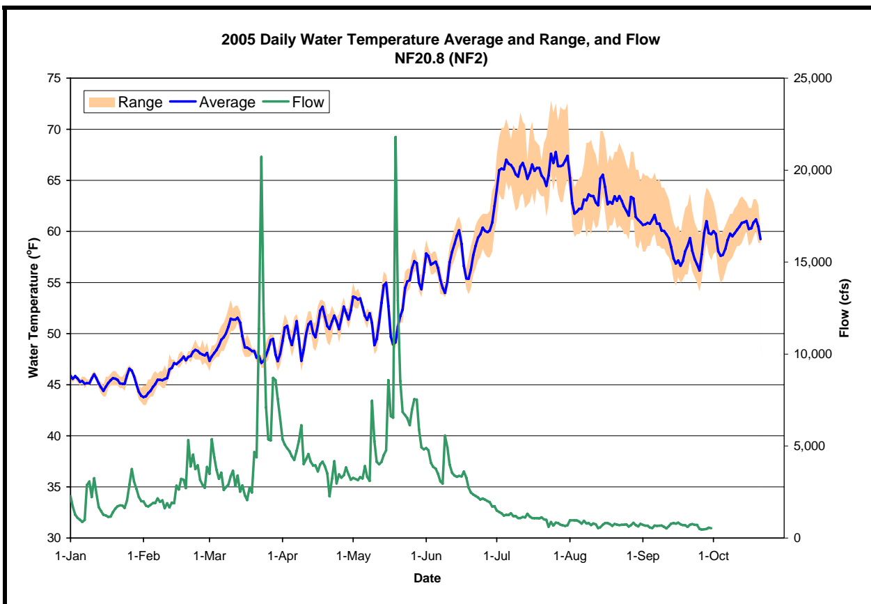
Figure A-45. The daily water temperature average and range measured at NF20.8 and the sum of flow measured at USGS # 11427000 (NF American below Clementine) and # 11433300 (MF American near Foresthill) during 2005
