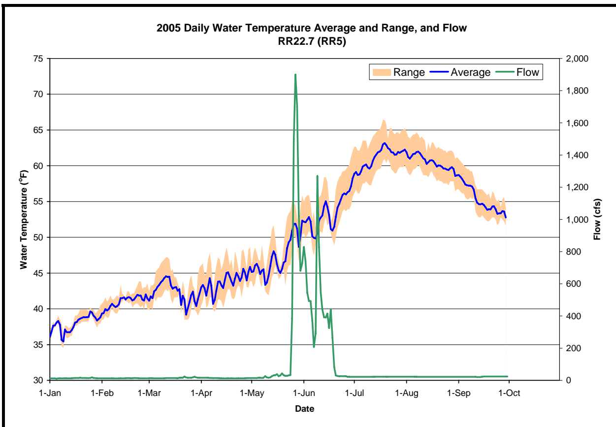
Figure A-65. The daily water temperature average and range measured at RR22.7 and flow measured at USGS # 11428800 (Rubicon below Hell Hole) during 2005
