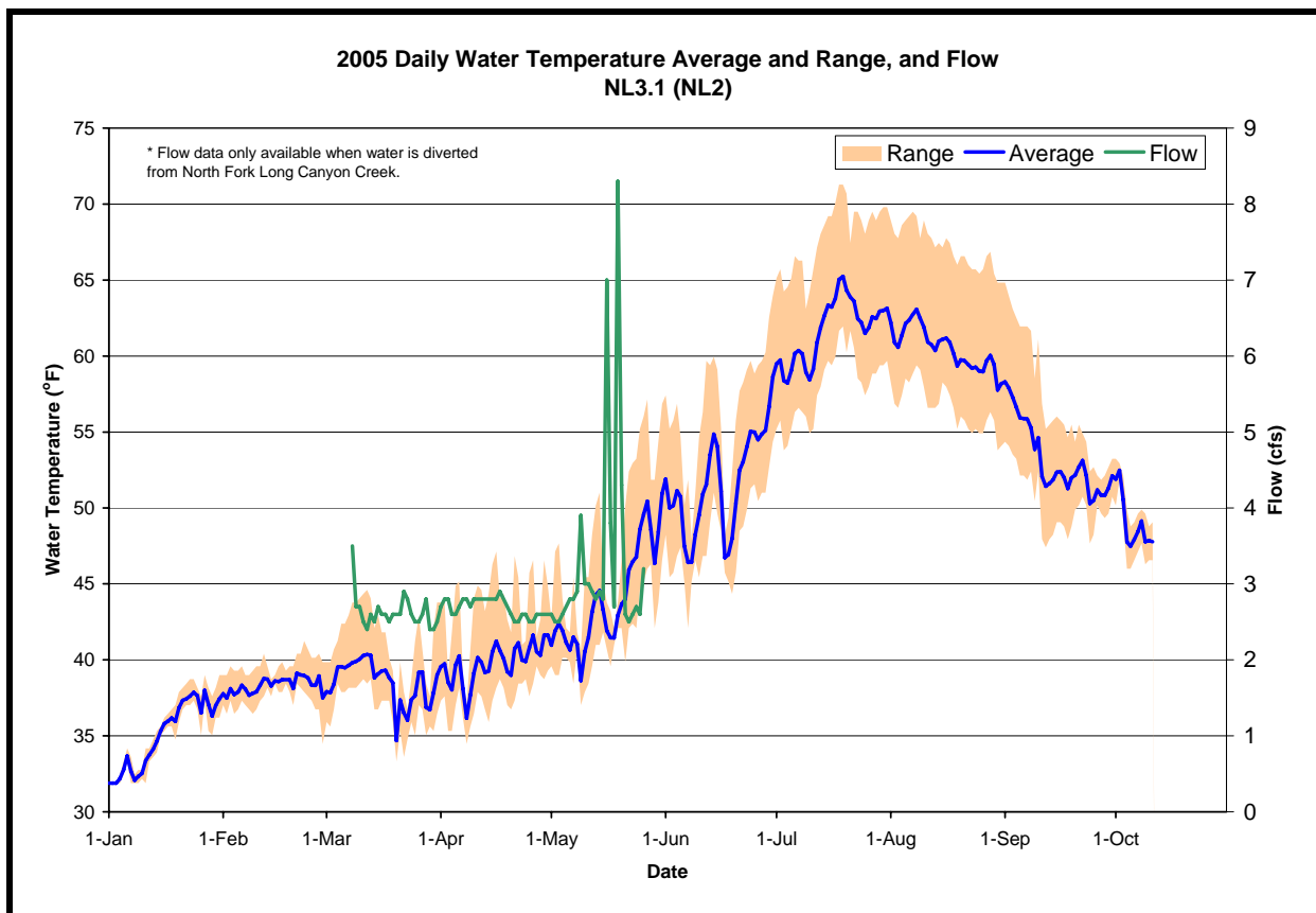
Figure A-51. The daily water temperature average and range measured at NL3.1 and flow measured at USGS # 11433085 (NF Long Canyon below diversion) during 2005. [Note: flows are only measured in North Fork Long Canyon Creek when flows are diverted, which typically occurs between late winter and spring. Consequently, flow data are not available during the summer]
