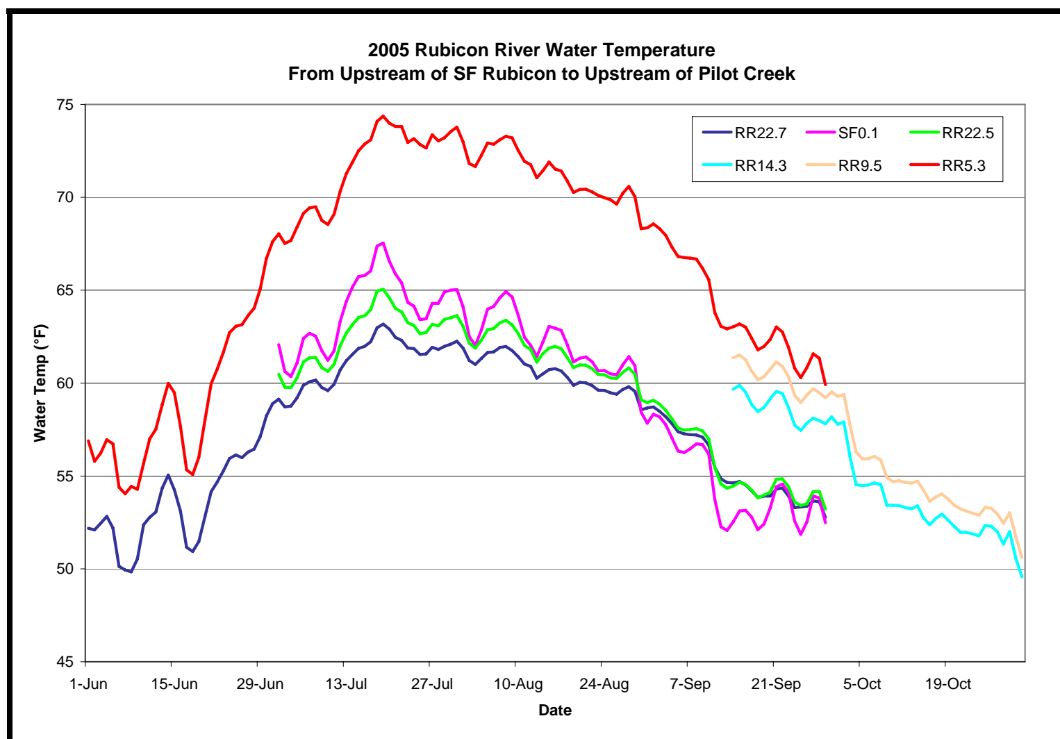
Figure 14. Summer and Fall Daily Average Water Temperature Data Collected in the Rubicon River at Sites RR22.7, SF0.1, RR22.5, RR14.3, RR9.5, and RR5.3. Refer to Figures 3-5 for the Relative Site Locations. [Note: The differences in the durations of the water temperature observations are due to differences in site installation and final download dates].
