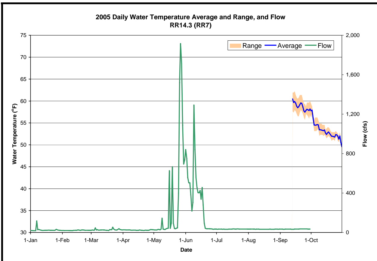
Figure A-69. The daily water temperature average and range measured at RR14.3 and the sum of flow measured at USGS # 11428800 (Rubicon below Hell Hole) and # 11430000 (SF Rubicon below Gerle Cr) during 2005
