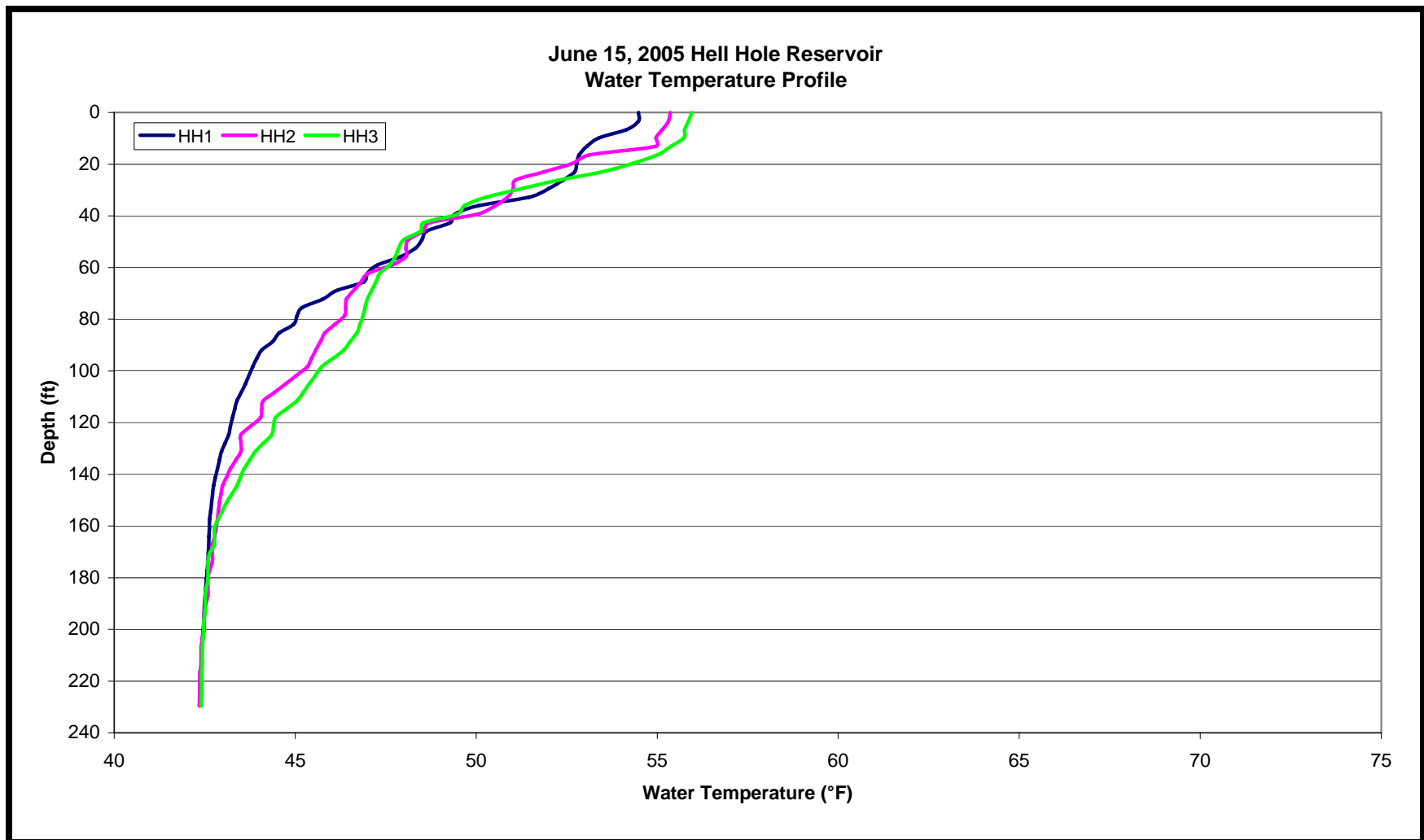
Figure 29. The Hell Hole Reservoir Water Temperature Profiles at Sites HH1, HH2, and HH3 on June 15, 2005.
