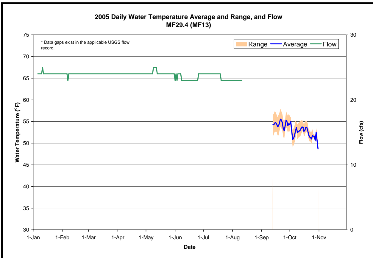
Figure A-41. The daily water temperature average and range measured at MF29.4 and flow measured at USGS # 11427770 (MF American below Interbay) during 2005
