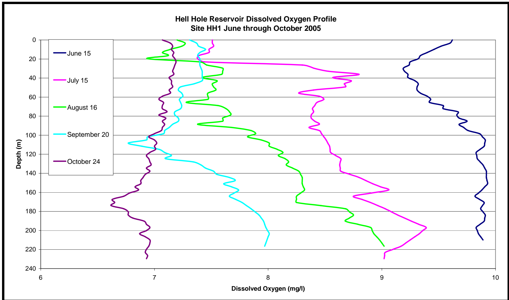
Figure 35. The Hell Hole Reservoir Dissolved Oxygen Profiles at Site HH1 (Nearest Hell Hole Dam) on June 15, July 15, August 16, September 20, and October 24, 2005.
