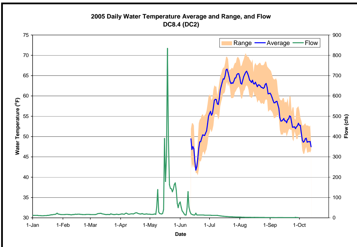
Figure A-3. The daily water temperature average and range measured at DC8.4 and flow measured at USGS # 11427750 (Duncan Cr below diversion) during 2005.
