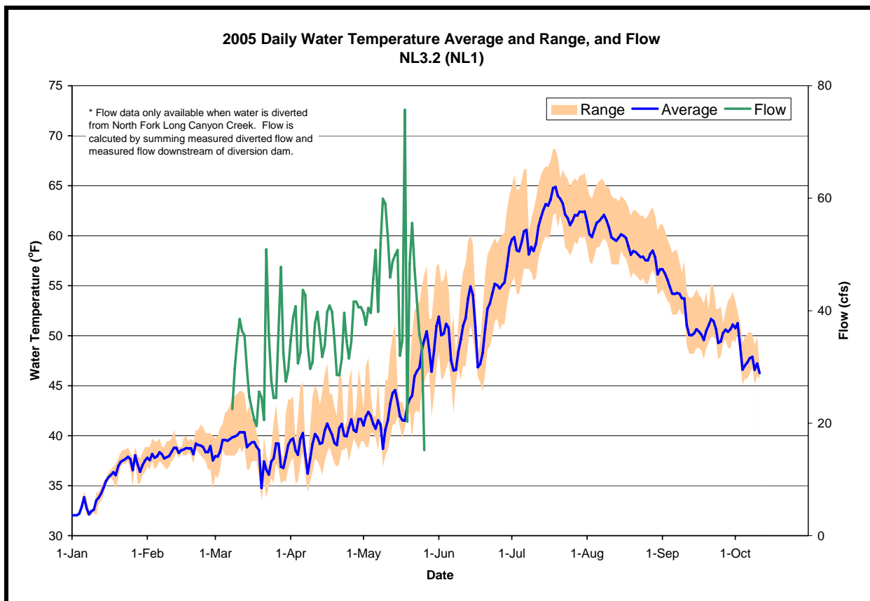
Figure A-49. The daily water temperature average and range measured at NL3.2 and the sum of flow measured at USGS # 11433080 (NF Long Canyon Diversion Tunnel) and # 11433085 (NF Long Canyon below diversion) during 2005. [Note: flows are only measured in North Fork Long Canyon Creek when flows are diverted, which typically occurs between late winter and spring. Consequently, flow data are not available during the summer]
