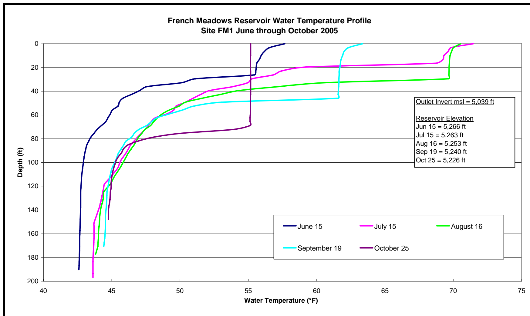
Figure 25. The French Meadows Reservoir Water Temperature Profiles at Site FM1 (Nearest French Meadows Dam) on June 15, July 15, August 16, September 19, and October 25, 2005, Including the River Outlet Invert Elevation and the Approximate Reservoir Elevation (msl) for Each Sample Date.
