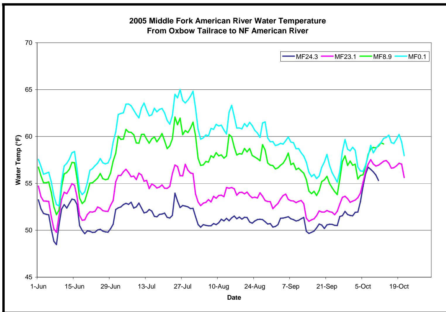
Figure 11. Summer and Fall Daily Average Water Temperature Data Collected in the Middle Fork American River at Sites MF24.3, MF23.1, MF8.9, and MF0.1. Refer to Figures 3-5 for the Relative Site Locations. [Note: The differences in the durations of the water temperature observations are due to differences in site installation and final download dates].
