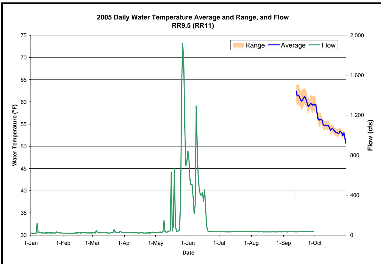
Figure A-77. The daily water temperature average and range measured at RR9.5 and the sum of flow measured at USGS # 11428800 (Rubicon below Hell Hole) and # 11430000 (SF Rubicon below Gerle Cr) during 2005
