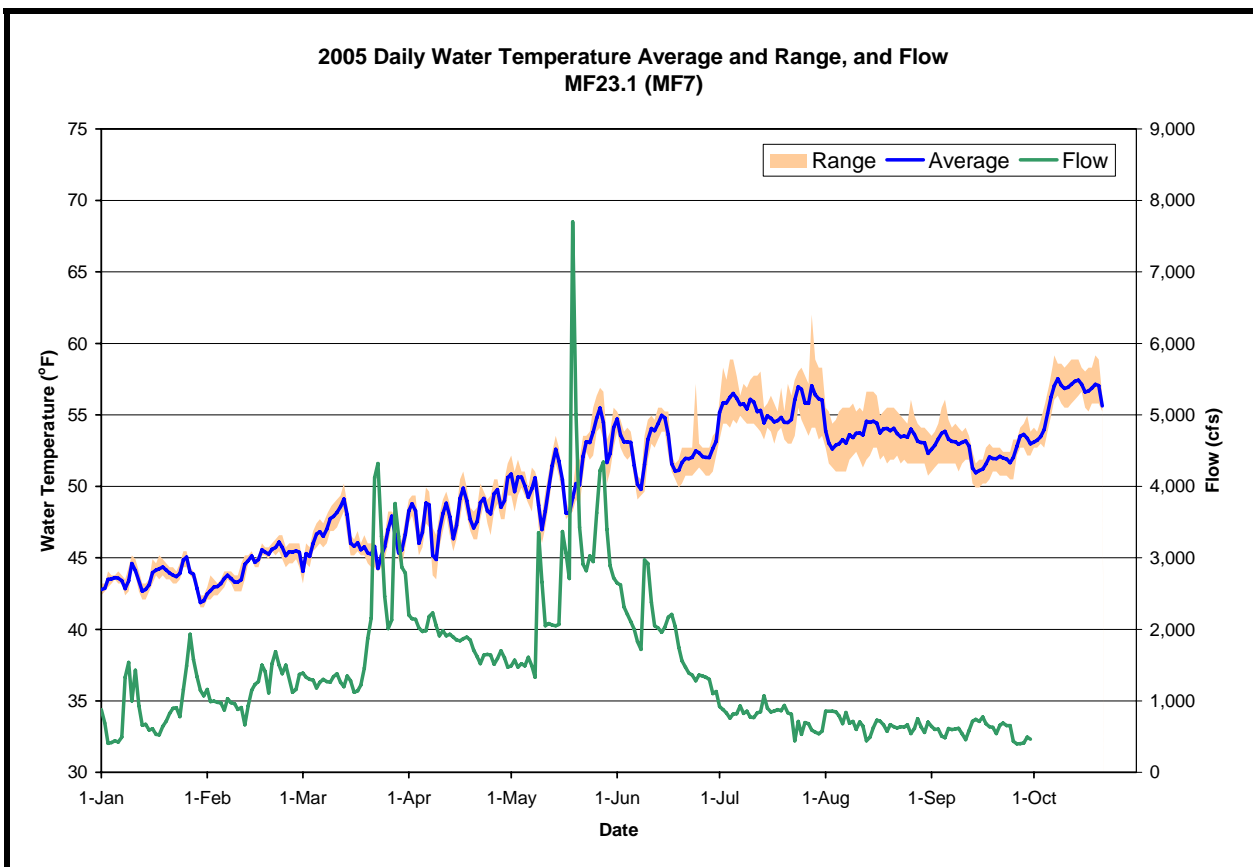
Figure A-29. The daily water temperature average and range measured at MF23.1 and flow measured at USGS # 11433300 (MF American near Foresthill) during 2005
