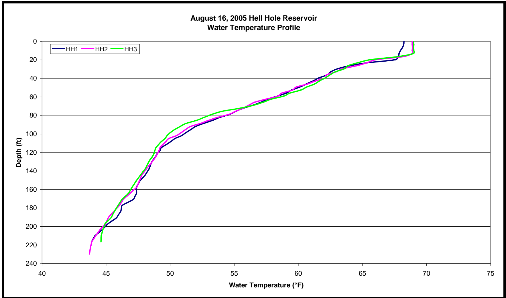
Figure 31. The Hell Hole Reservoir Water Temperature Profiles at Sites HH1, HH2, and HH3 on August 16, 2005.
