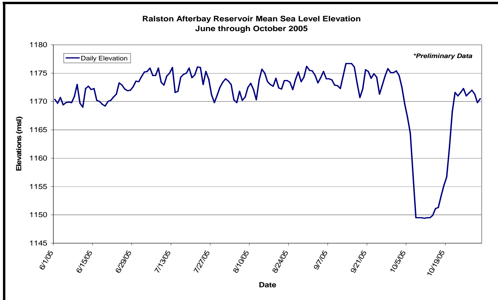
Figure 38. The Daily Reservoir Elevation at Ralston Afterbay Reservoir During June through October 2005. [Note the decrease in reservoir elevation during the MFP powerhouse maintenance outage period during October]. [Note: Preliminary data].
