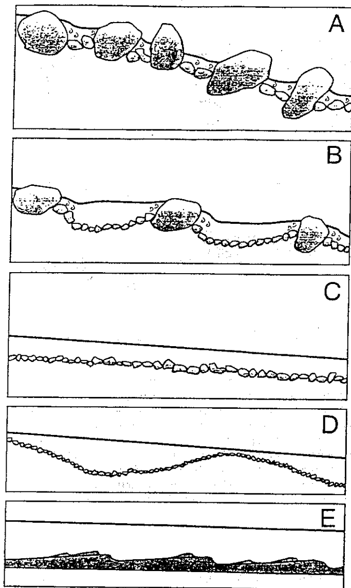
Figure 3. Schematic longitudinal profiles of alluvial channel morphologies at low flow: (A) cascade; (B) step pool; (C) plane bed; (D) pool riffle; and (E) dune ripple.
