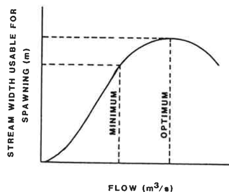
FIGURE 4.5.—Usable-width technique for determining spawning flow. (From Thompson 1972.)
