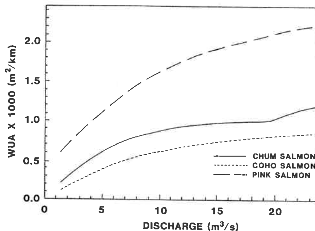
FIGURE 4.6.—Relation of available chum, coho, and pink salmon spawning habitat (weighted usable area, WUA) to streamflow, Upper Tunnel Creek. (From Reiser and Ramey 1984.)
