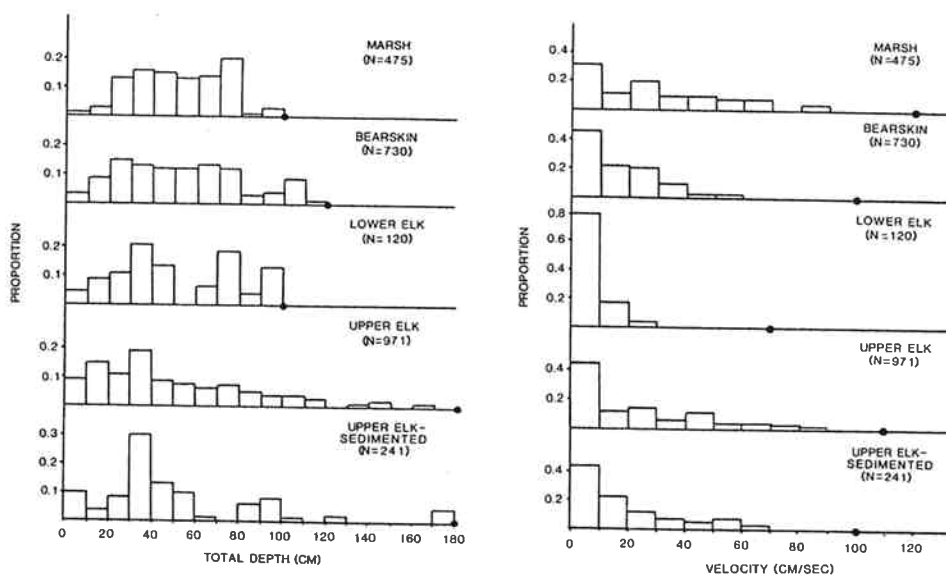
FIGURE 4.32.—Distribution of age-0 chinook salmon (77–89 mm mean total length) relative to water depth and velocity in pools of Idaho streams in August 1979. Dots indicate maximum water depth or velocity observed in the pools surveyed. (From Konopacky 1984.)
