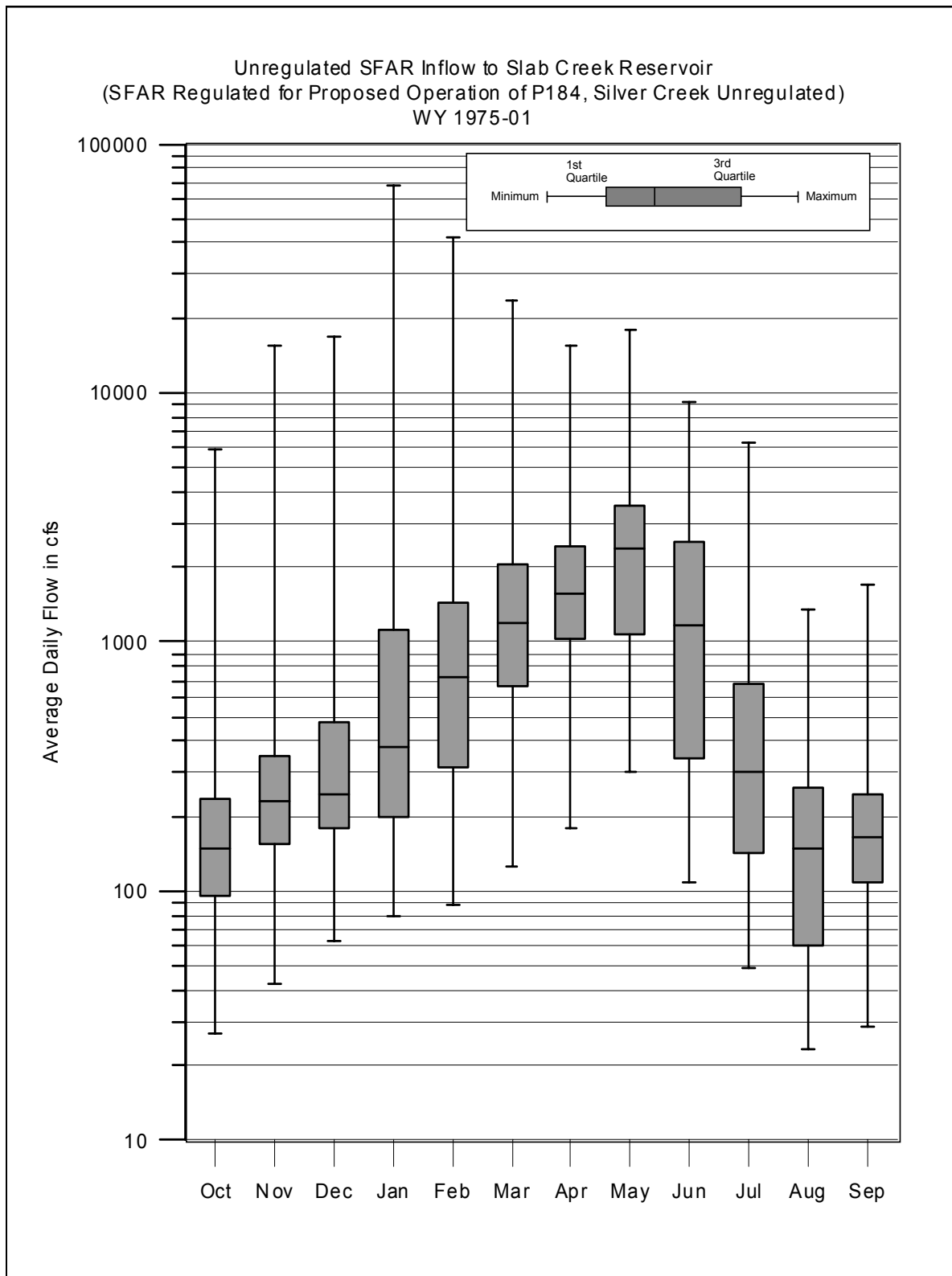
Figure 3.2.7-1. Unregulated SFAR Inflow to Slab Creek Reservoir (SFAR Regulated for P184, Silver Creek Unregulated) WY 1975-01, Monthly Box-whisker Diagram
