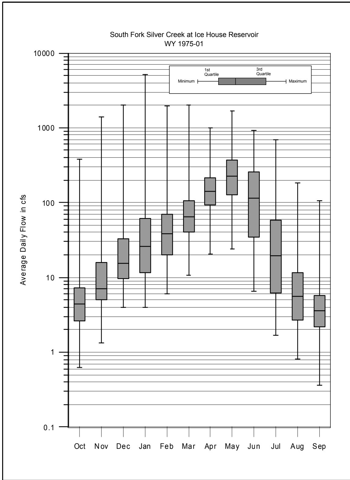
Figure 3.2.1-13. SF Silver Creek at Ice House Reservoir, Monthly Box-whisker Diagram
