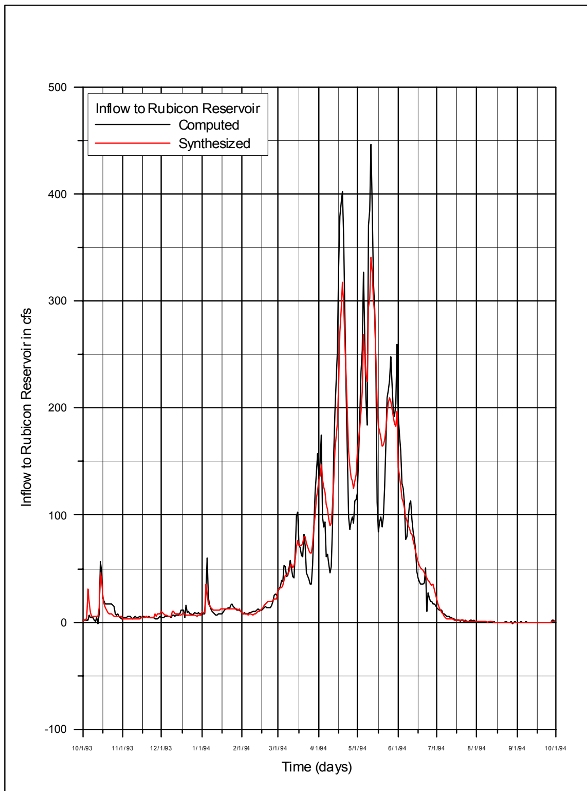
Figure 3.2.2-2. Inflow to Rubicon Reservoir, WY 1994
