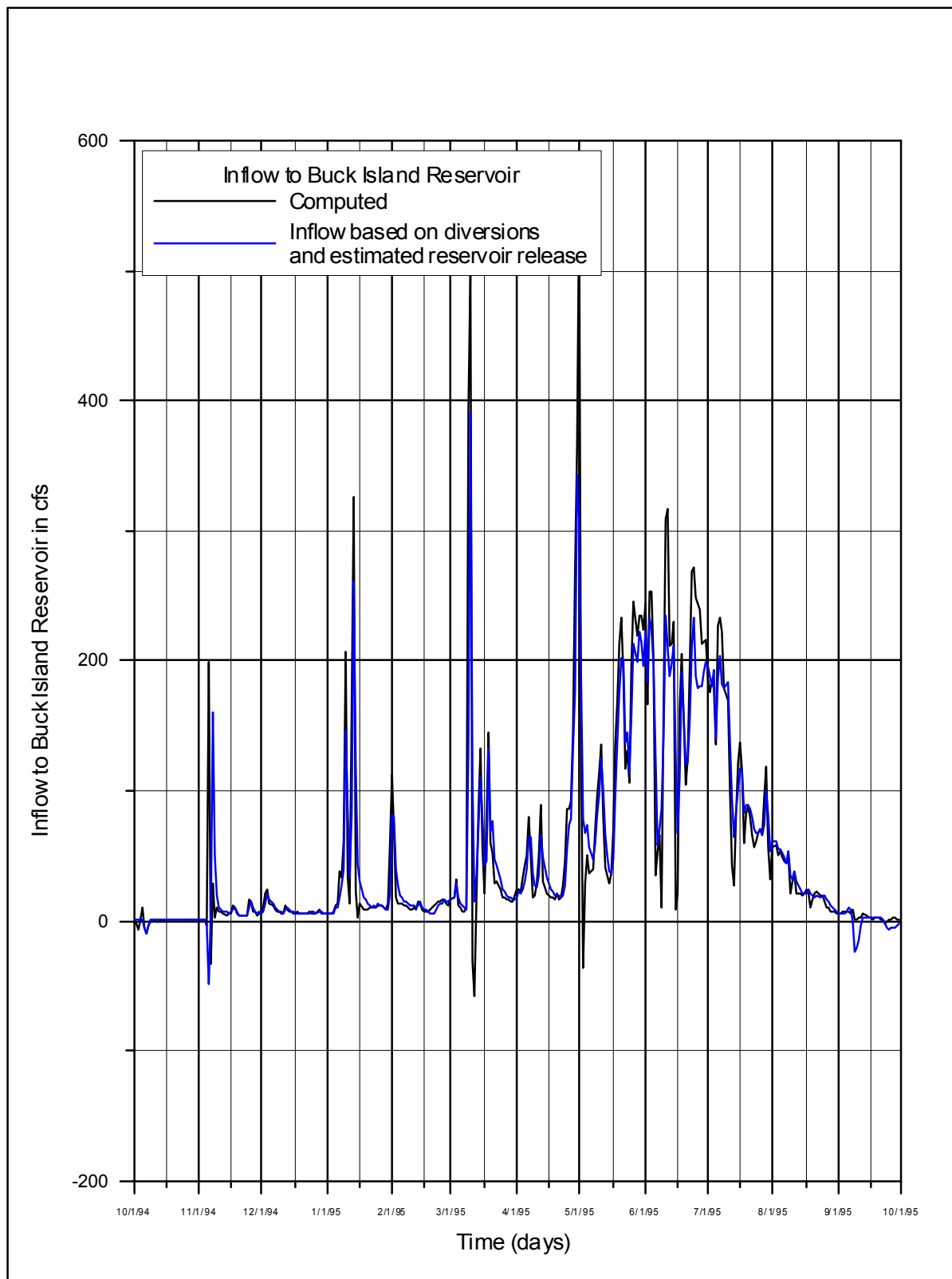
Figure 3.2.3-4. Inflow to Buck Island Reservoir, WY 1995 (on the x-axis, the plot runs from October 1, 1994 through October 1, 1995)
