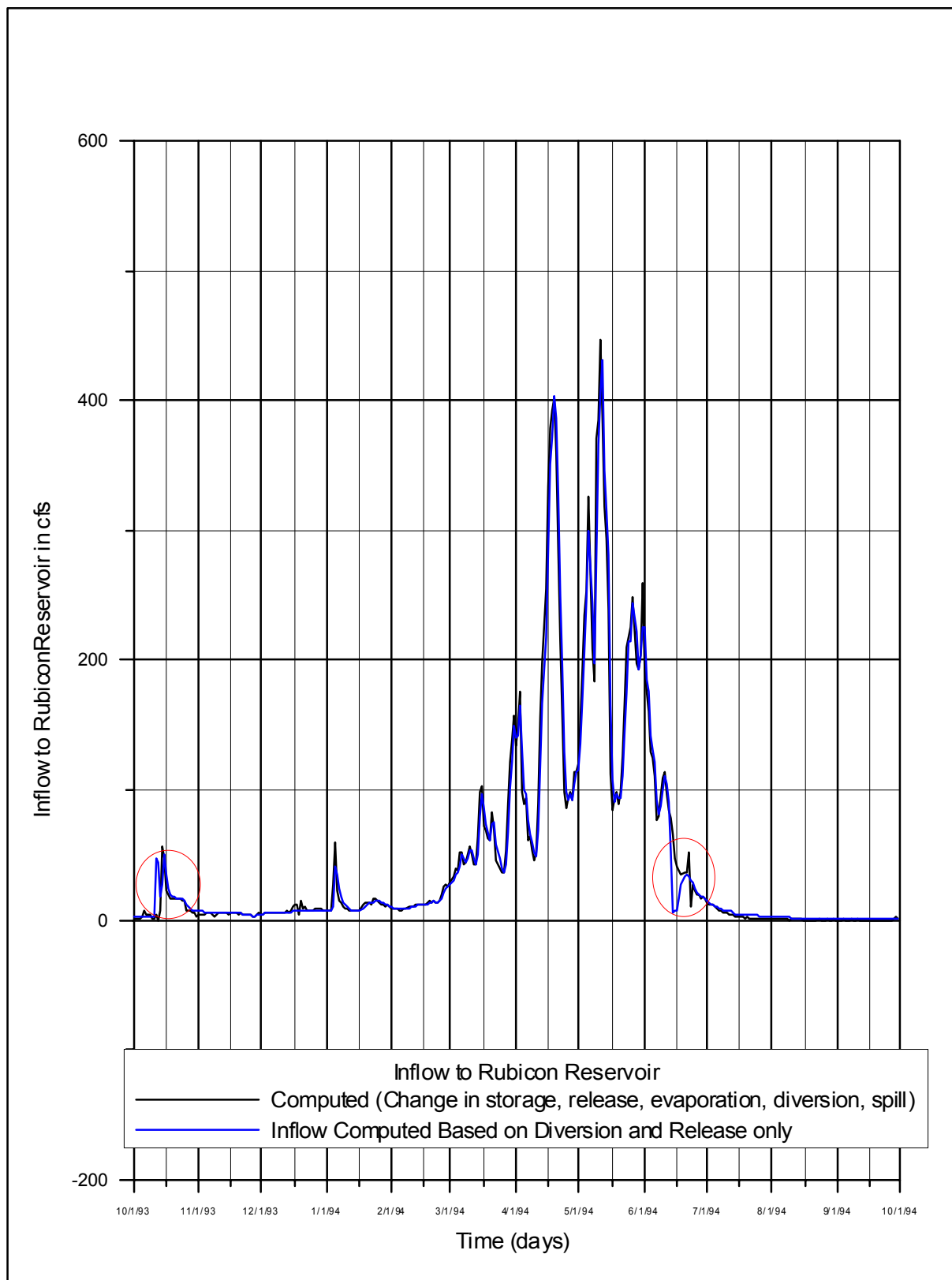
Figure 3.2.2-7. Inflow to Rubicon Reservoir, WY 1994
