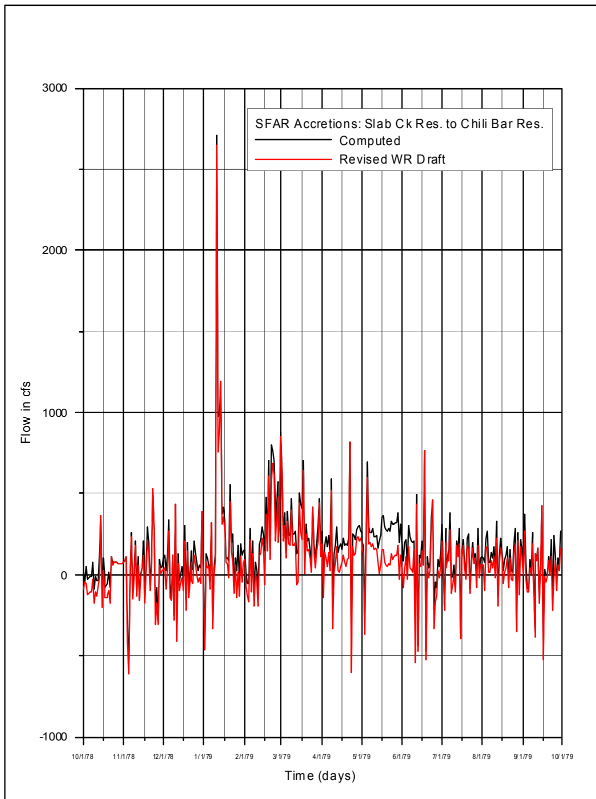
Figure 3.2.8-7. SFAR Accretions: Slab Creek Reservoir to Chili Bar Reservoir, WY 1979
