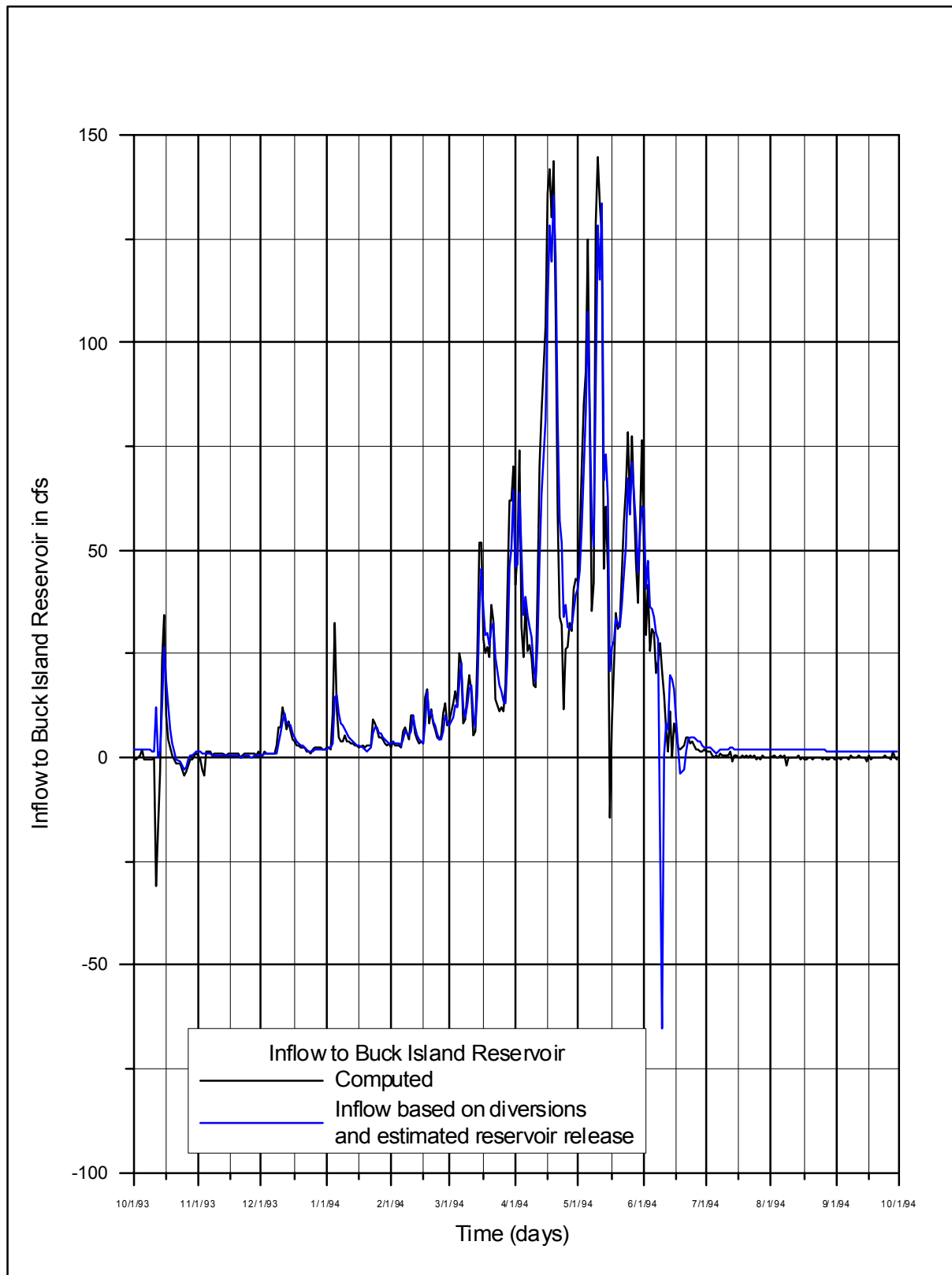
Figure 3.2.3-3. Inflow to Buck Island Reservoir, WY 1994
