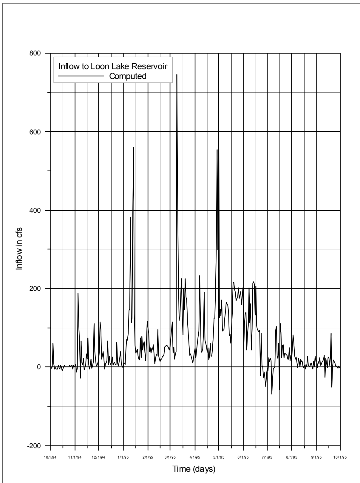
Figure 3.2.4-3. Inflow to Loon Lake Reservoir, WY 1995
