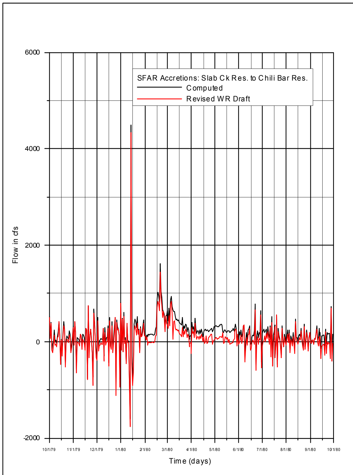
Figure 3.2.8-6. SFAR Accretions: Slab Creek Reservoir to Chili Bar Reservoir, WY 1980
