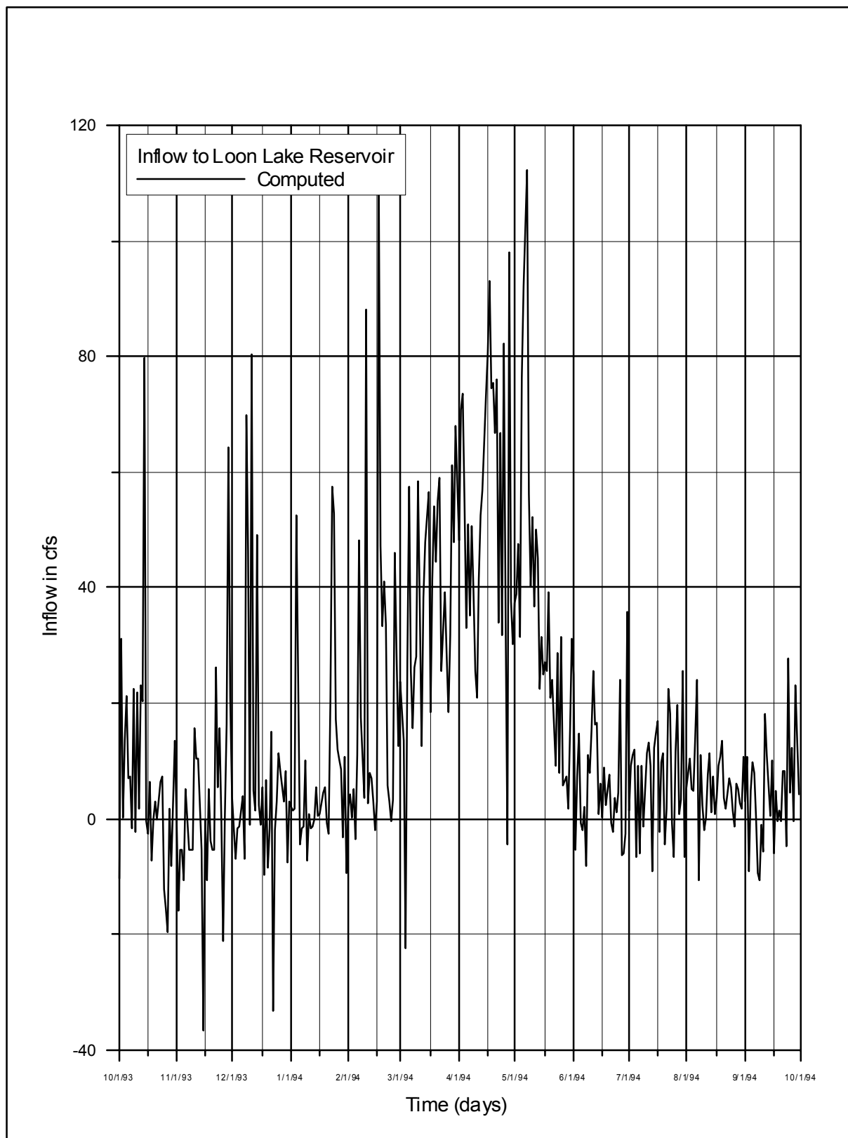
Figure 3.2.4-4. Inflow to Loon Lake Reservoir, WY 1994
