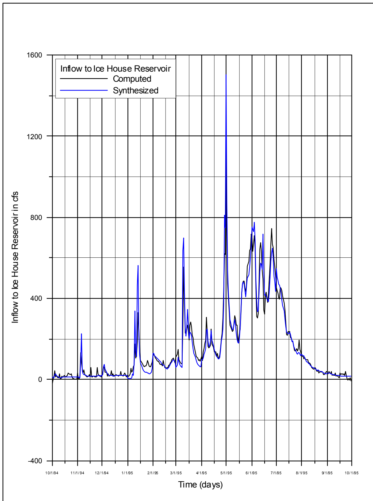
Figure 3.2.1-7. Inflow to Ice House Reservoir, WY 1995
