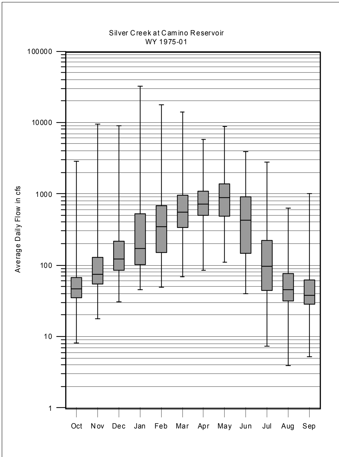
Figure 3.2.6-22. Silver Creek at Camino Reservoir, WY 1975-01, Monthly Box -Whisker Diagram
