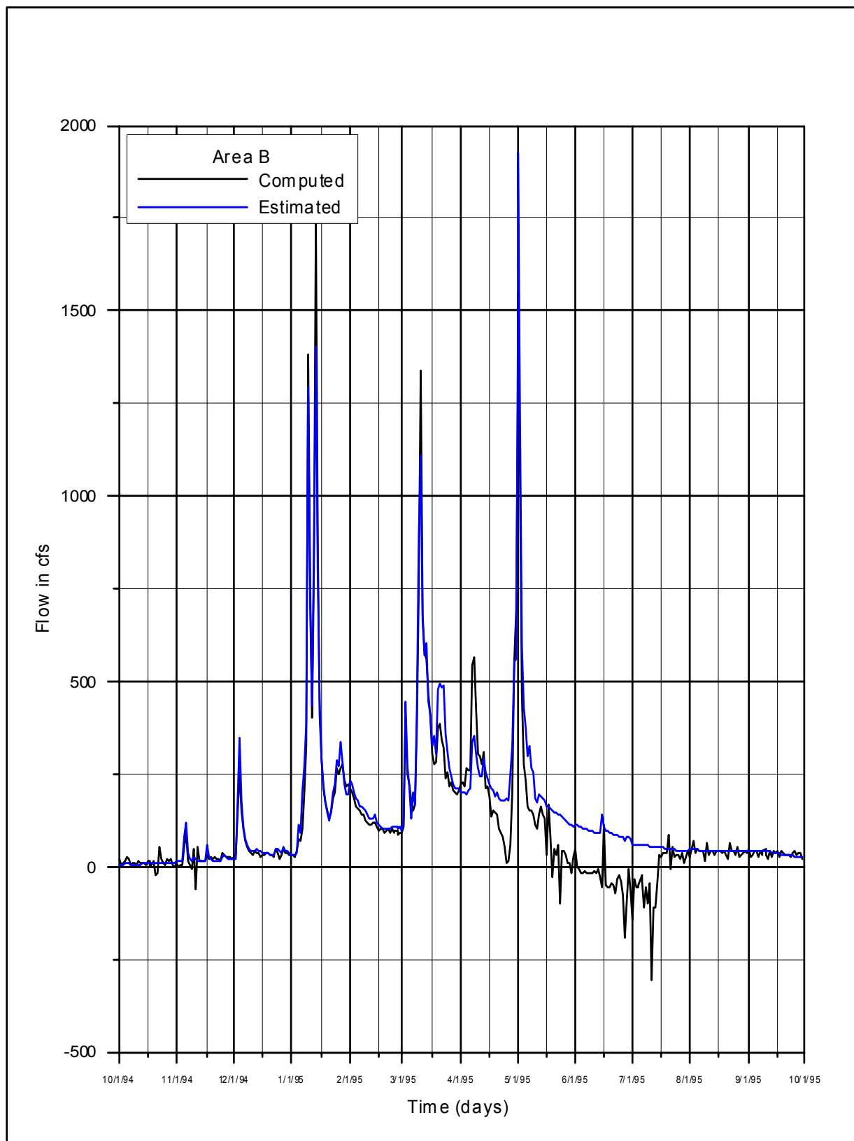
Figure 3.2.6-18 Area B, WY 1995
