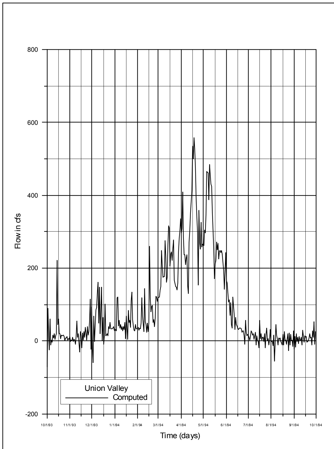
Figure 3.2.5-4. Union Valley, WY 1994
