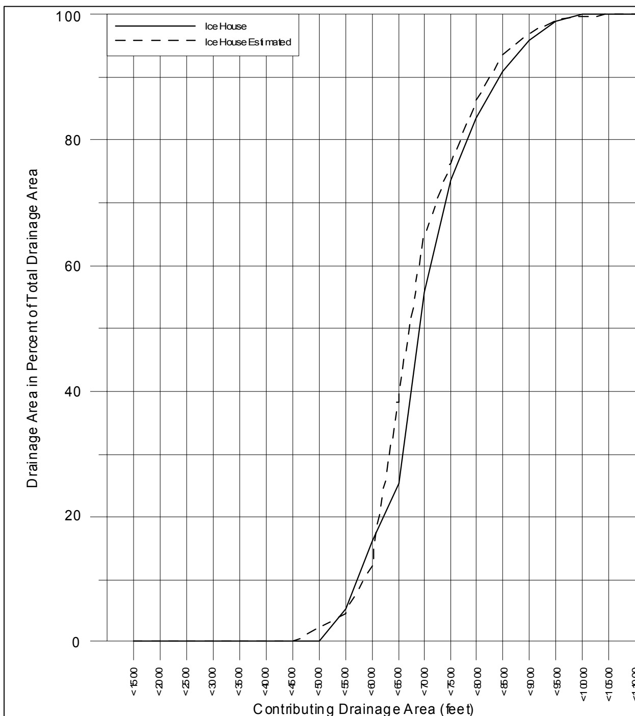
Figure 3.2.1-6. Ice House Reservoir Drainage Area Versus Elevation For Simulated Data
