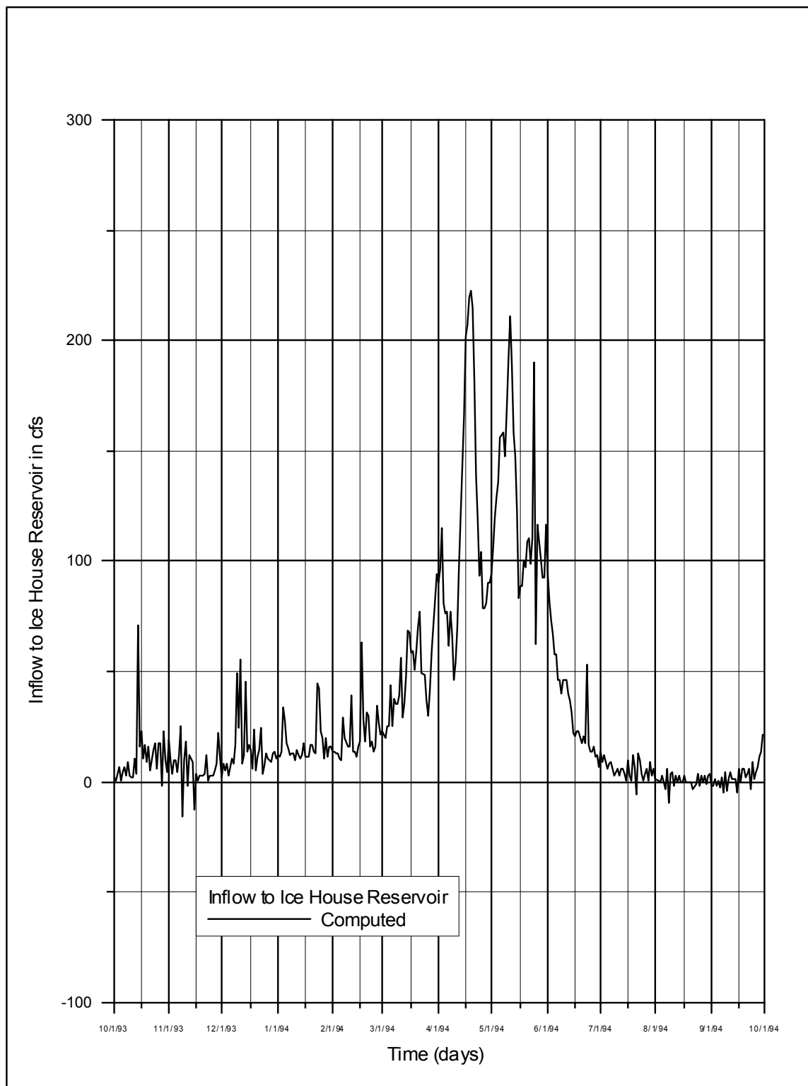
Figure 3.2.1-4. Inflow to Ice House Reservoir, WY 1994
