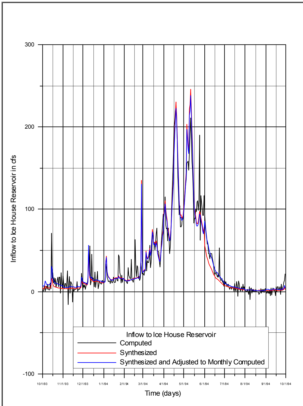
Figure 3.2.1-11. Inflow to Ice House Reservoir, WY 1994
