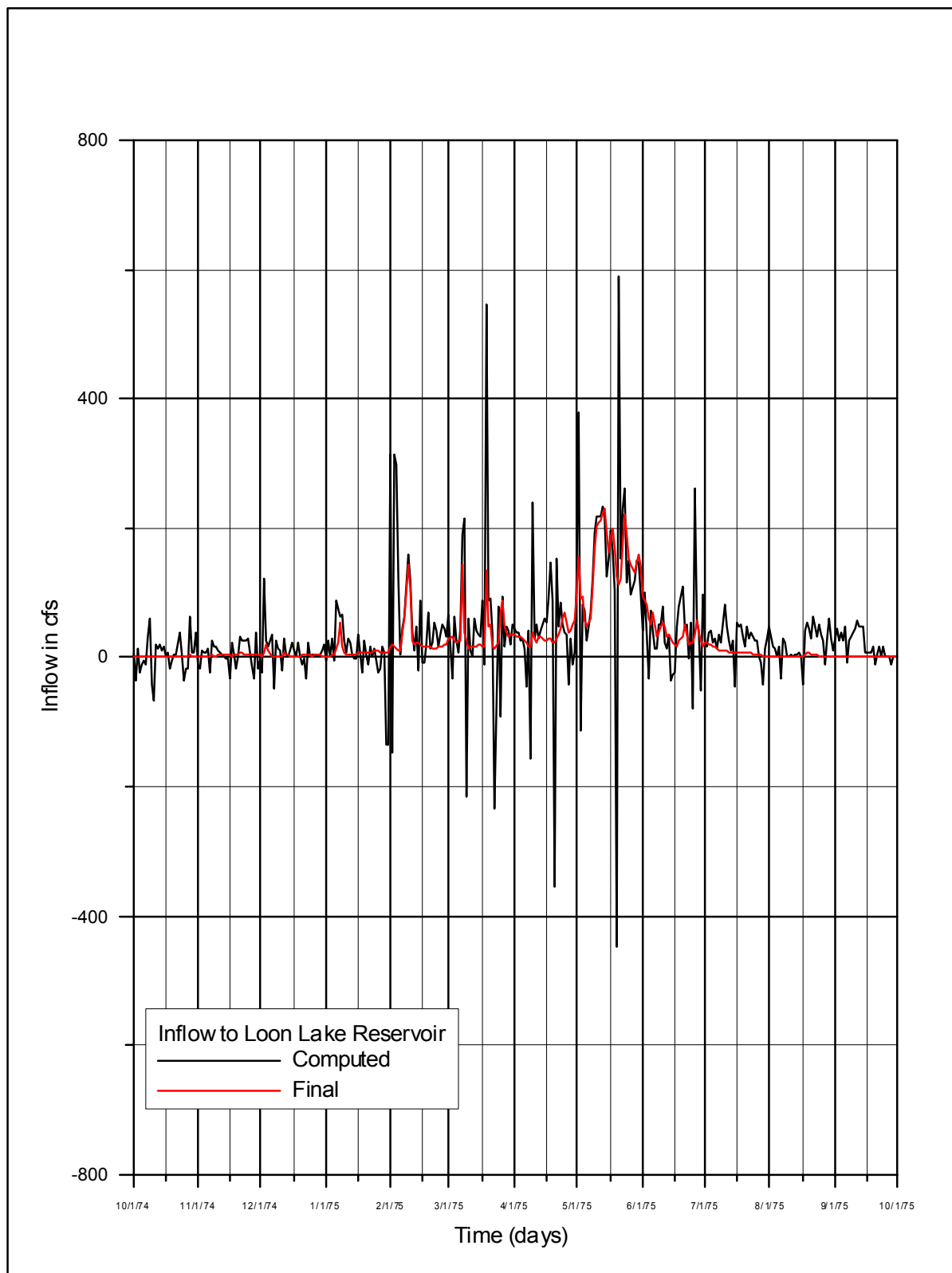
Figure 3.2.4-12. Inflow to Loon Lake Reservoir, WY 1975
