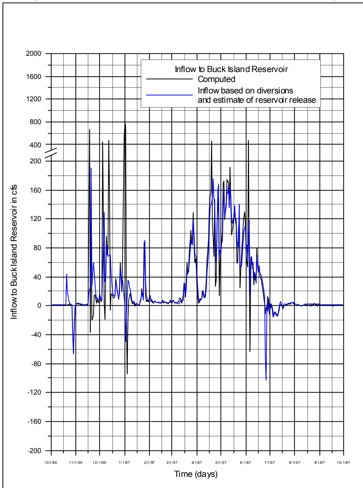
Figure 3.2.3-5. Inflow to Buck Island Reservoir, WY 1997 (on the x-axis, the plot runs from October 1, 1996 through October 1, 1997)
