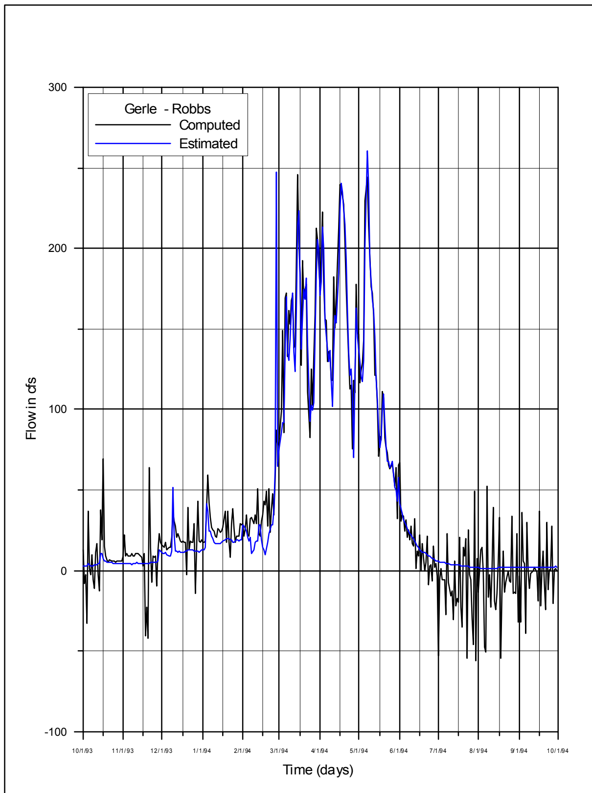
Figure 3.2.4-16. Gerle – Robbs, WY 1994
