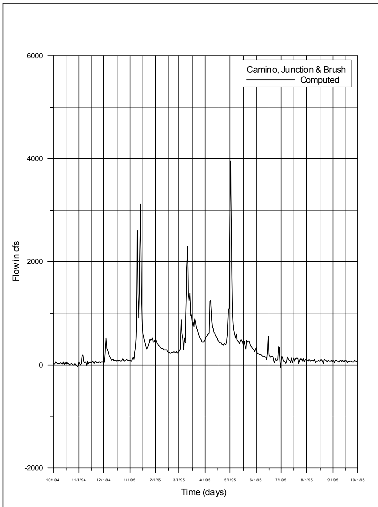
Figure 3.2.6-2. Camino, Junction and Brush, WY 1995
