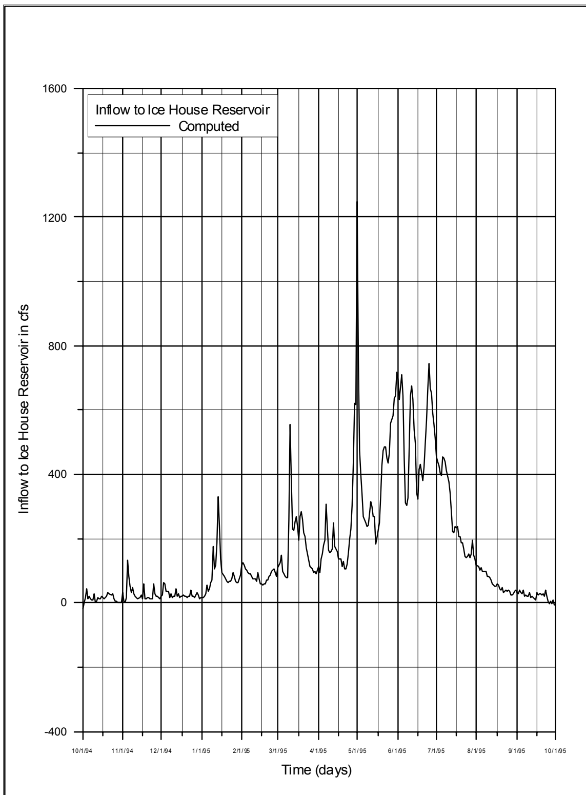
Figure 3.2.1-2. Inflow to Ice House Reservoir, WY 1995
