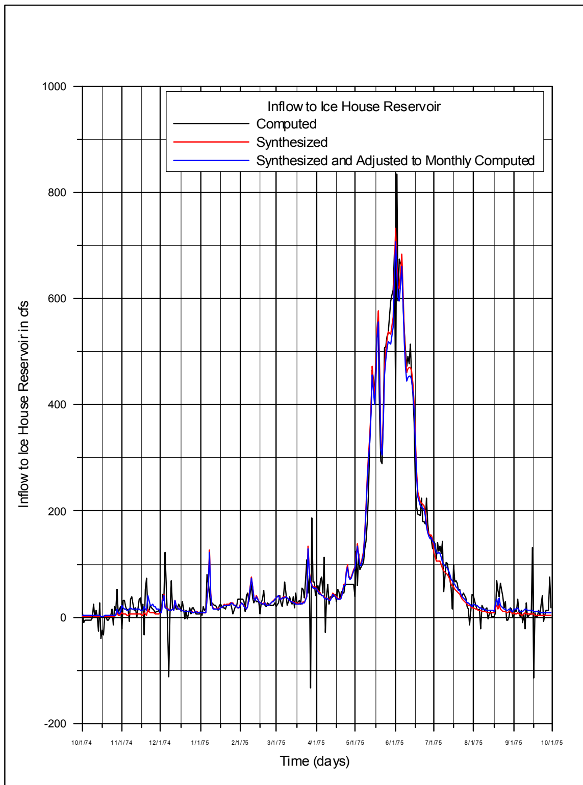
Figure 3.2.1-10. Inflow to Ice House Reservoir, WY 1975
