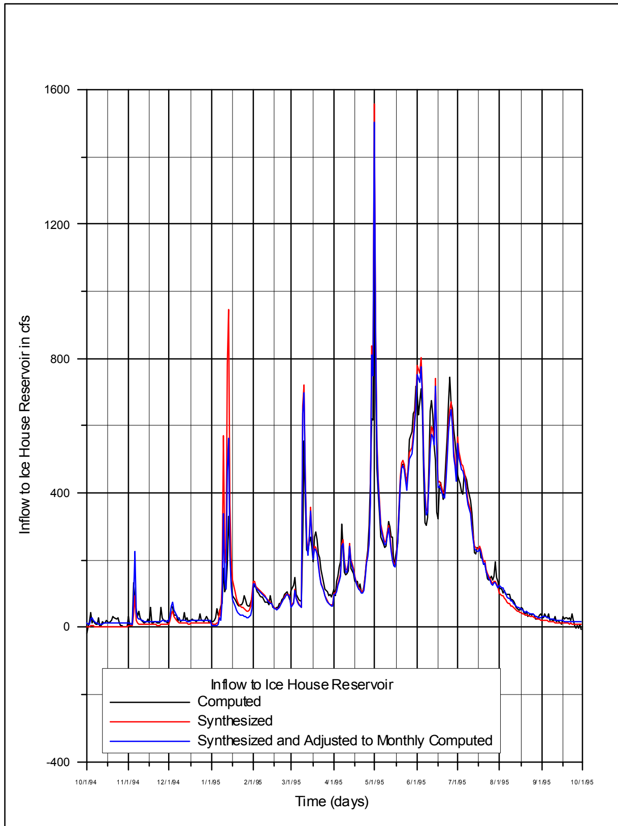
Figure 3.2.1-9. Inflow to Ice House Reservoir, WY 1995
