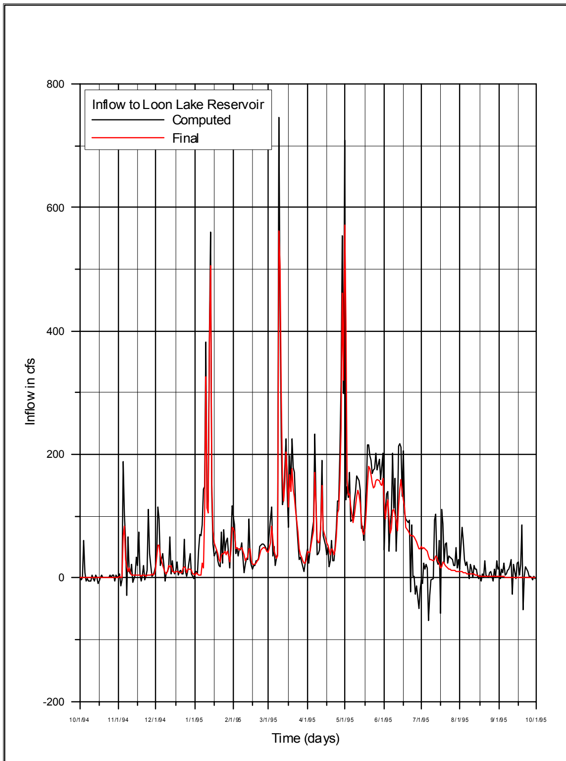
Figure 3.2.4-11. Inflow to Loon Lake Reservoir, WY 1995
