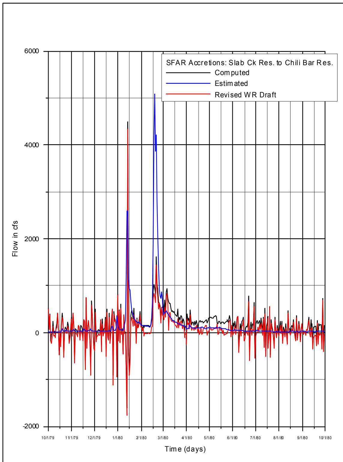
Figure 3.2.8-8. SFAR Accretions: Slab Creek Reservoir to Chili Bar Reservoir, WY 1980
