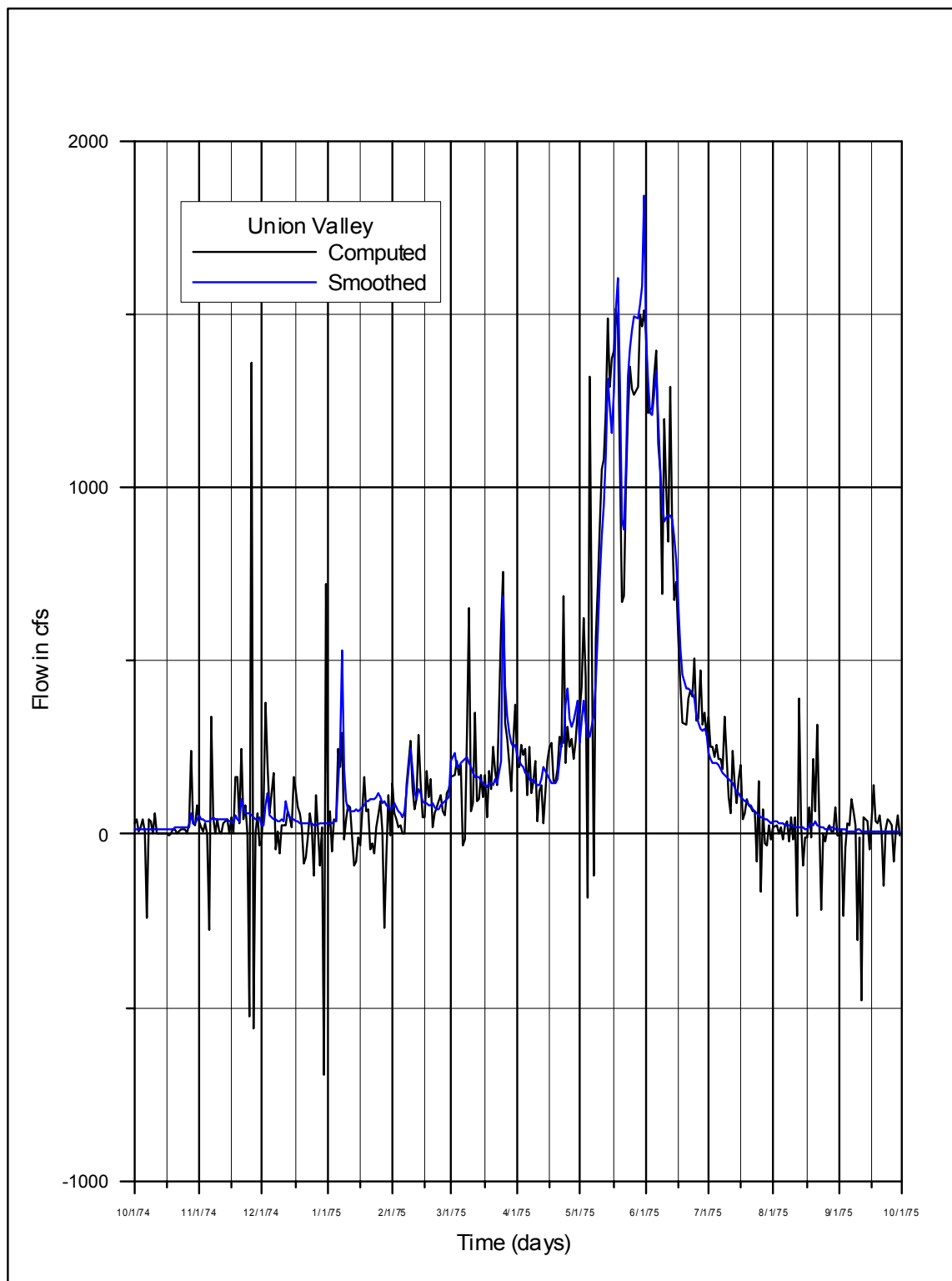
Figure 3.2.5-7. Union Valley, WY 1994
