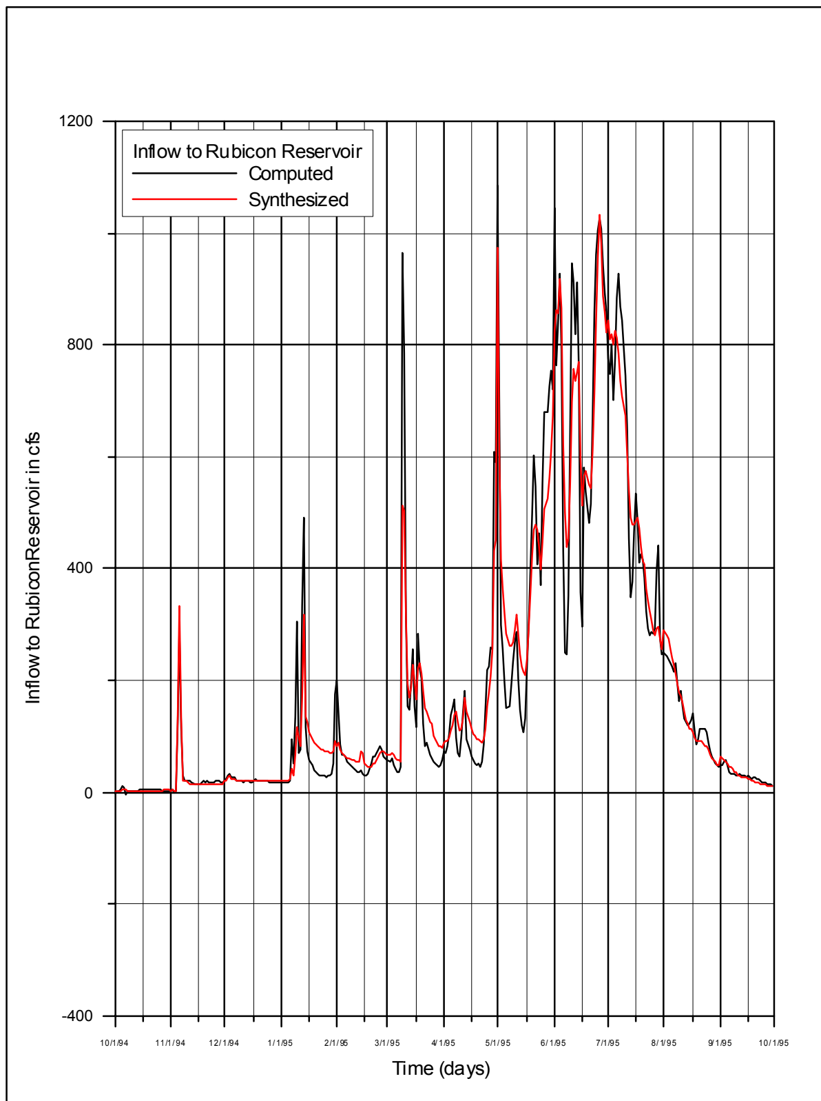
Figure 3.2.2-1. Inflow to Rubicon Reservoir, WY 1995
