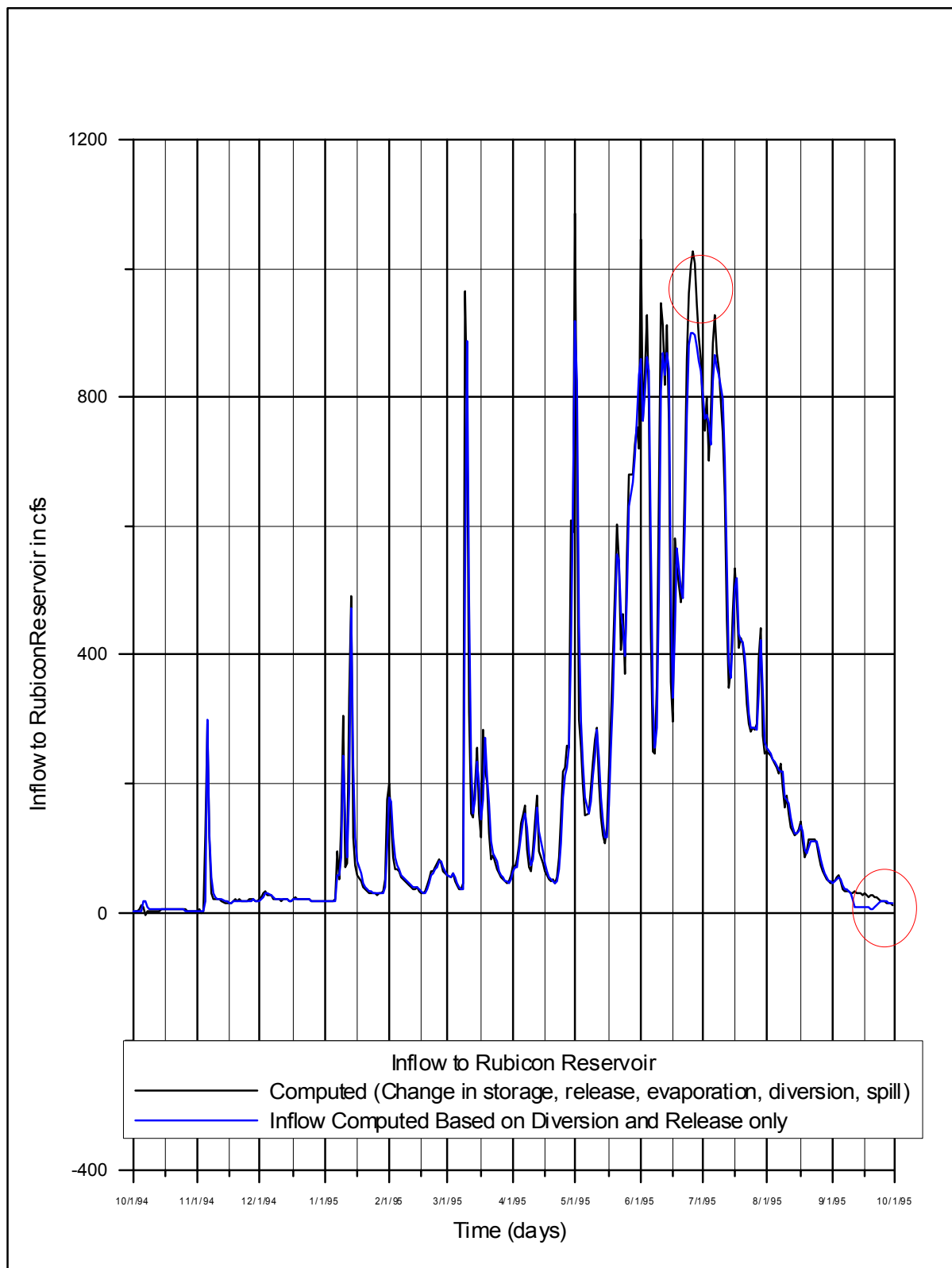
Figure 3.2.2-6. Inflow to Rubicon Reservoir, WY 1995
