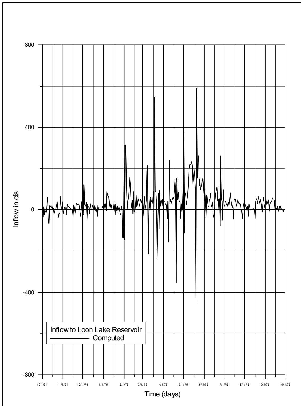
Figure 3.2.4-5. Inflow to Loon Lake Reservoir, WY 1975
