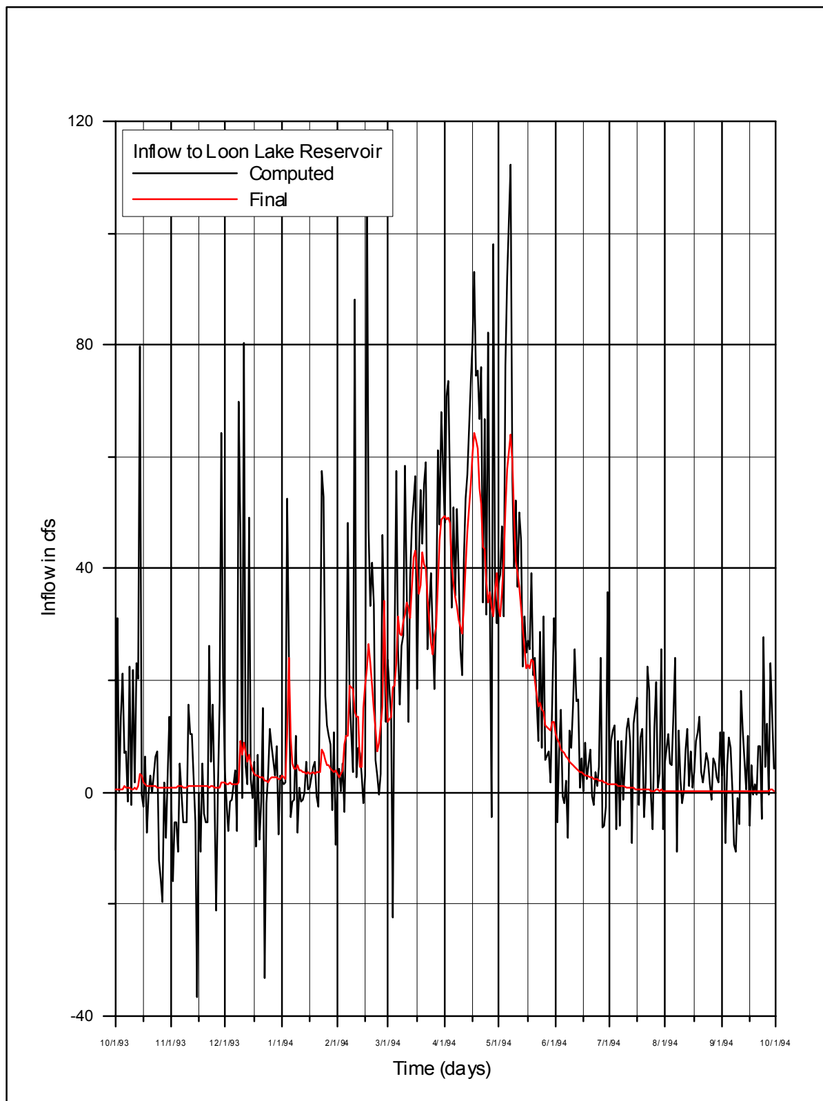
Figure 3.2.4-13. Inflow to Loon Lake Reservoir, WY 1994
