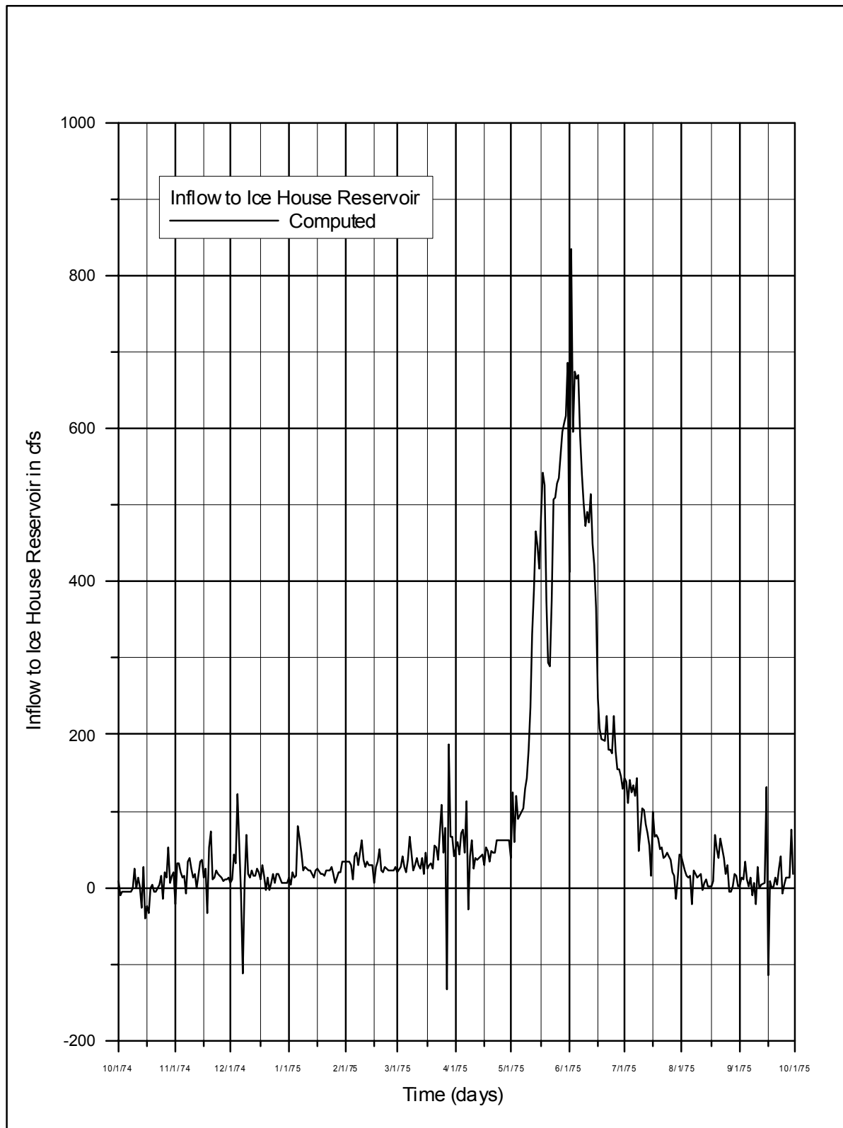
Figure 3.2.1-3. Inflow to Ice House Reservoir, WY 1975
