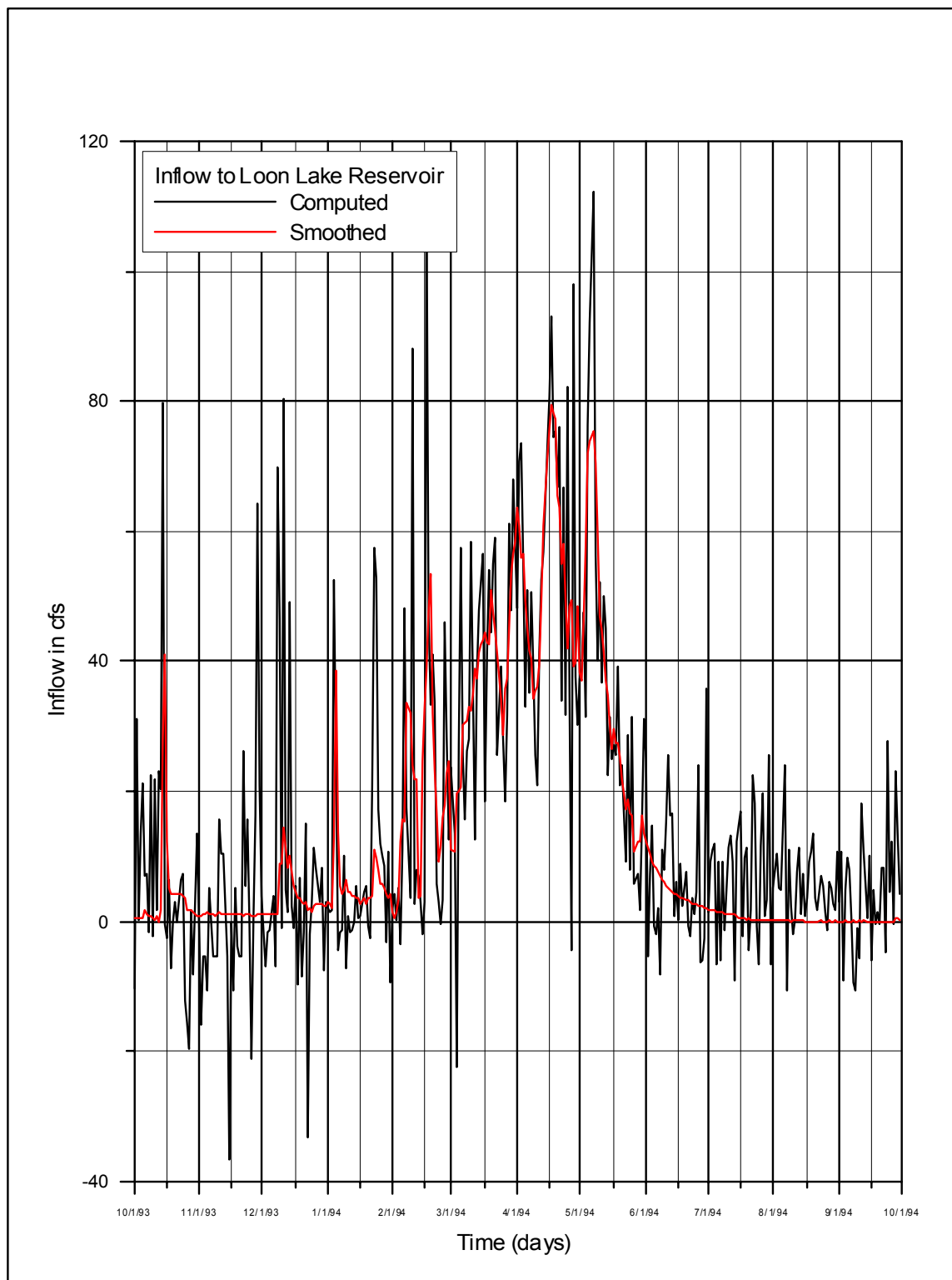
Figure 3.2.4-6. Inflow to Loon Lake Reservoir, WY 1994
