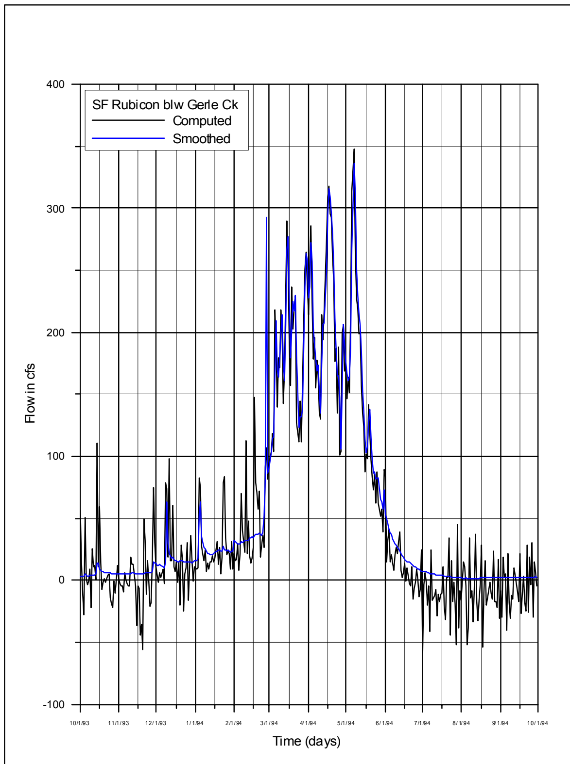
Figure 3.2.4-8. SF Rubicon below Gerle Creek, WY 1994
