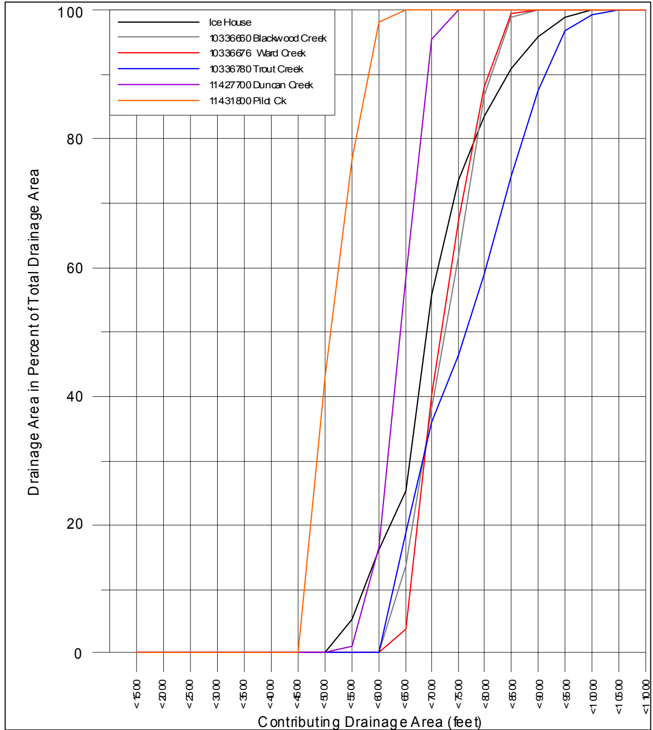
Figure 3.2.1-5. Ice House Reservoir Drainage Area Versus Elevation
