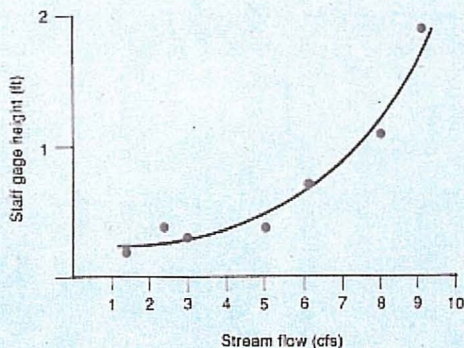
Forming a Stage-Discharge Curve
