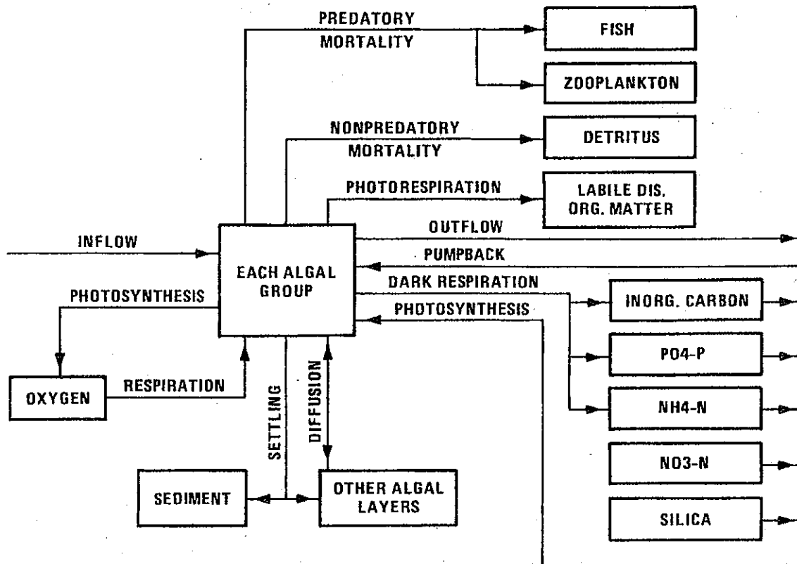
Figure 46. Fluxes for the algal compartments
