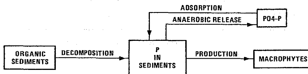
Figure 69. Fluxes among sediment phosphorus and other compartments
