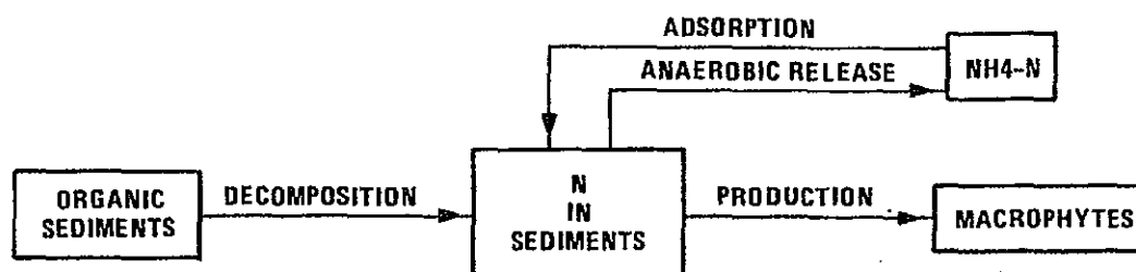
Figure 70. Fluxes among sediment nitrogen and other compartments
