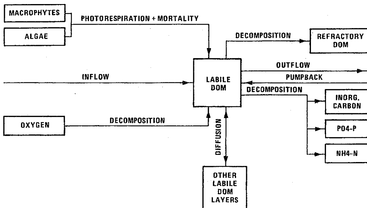
Figure 51. Fluxes for the labile DOM compartment
