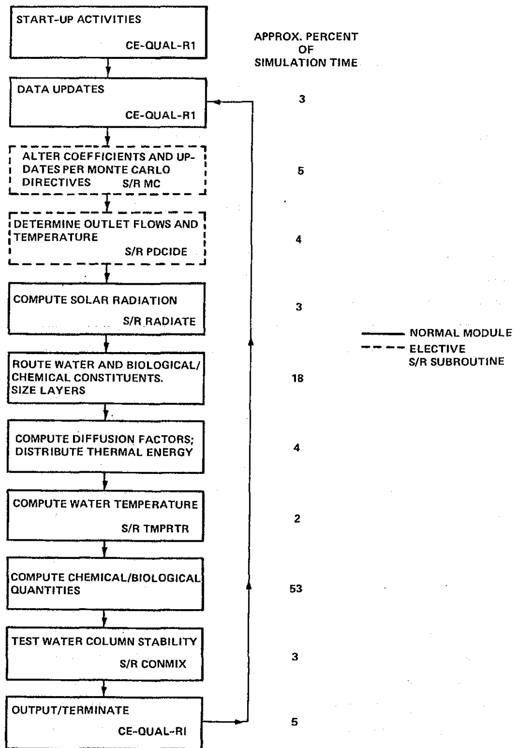
Figure 4. Sequence and timing of CE-QUAL-R1 elements
