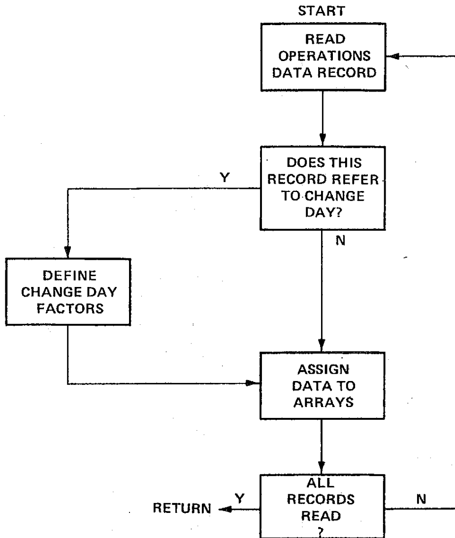
Figure 22. Flowchart representing subroutine OPREAD
