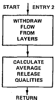
Figure 30. Flowchart for subroutine OUTVEL
