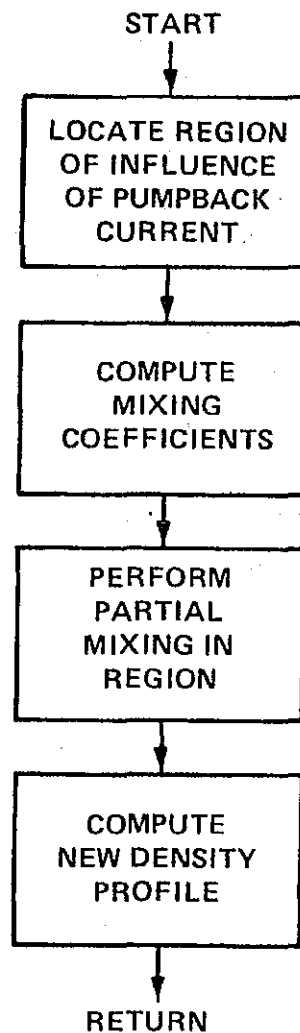
Figure 29. Flowchart for subroutine BUCKET
