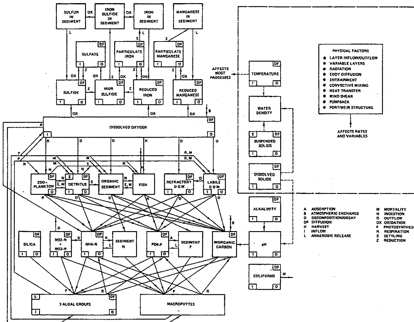
Figure 2. Overall organization of CE-QUAL-R1. CE-THERM-R1 is represented in the large dashed box. Solid lines represent processes and the transfer of mass. Short dashed lines represent information transfer
