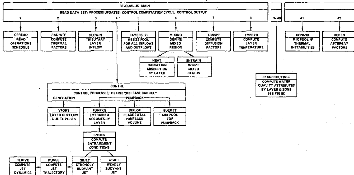
Figure 6. Relationships of water quality components for scheduled generation mode
