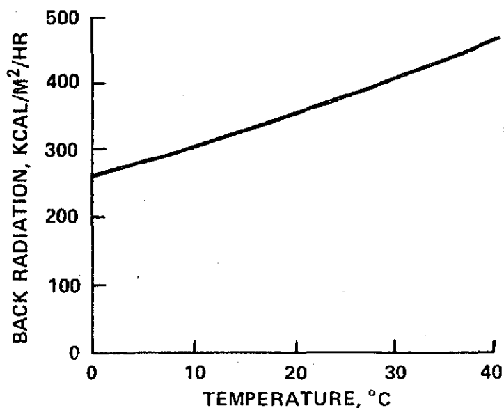
Figure 18. Back radiation
