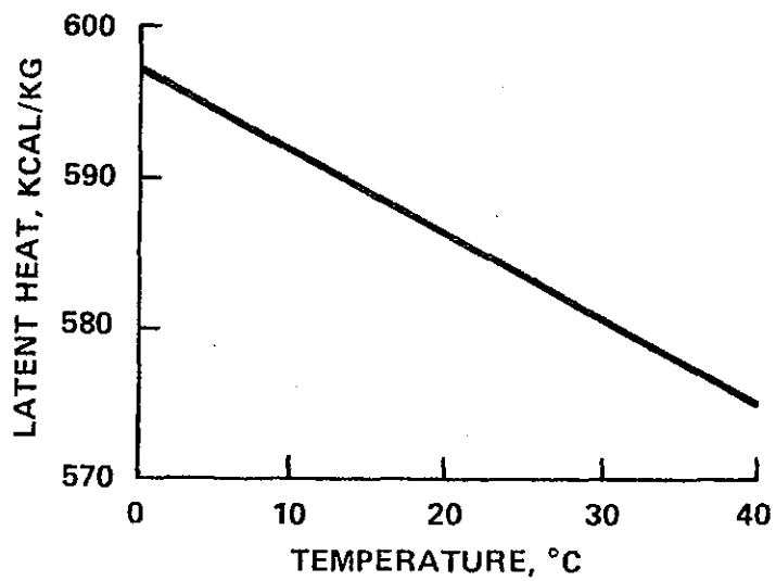
Figure 19. Latent heat,
