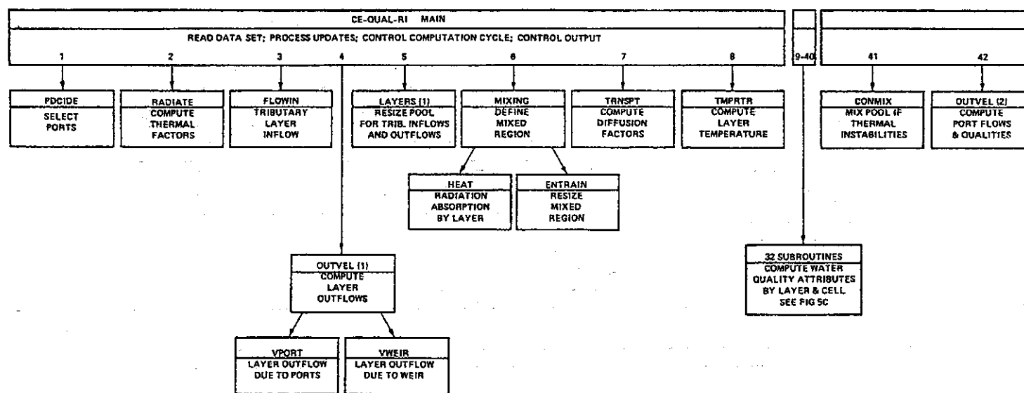
Figure 5. Relationships of water quality components for normal operations mode
