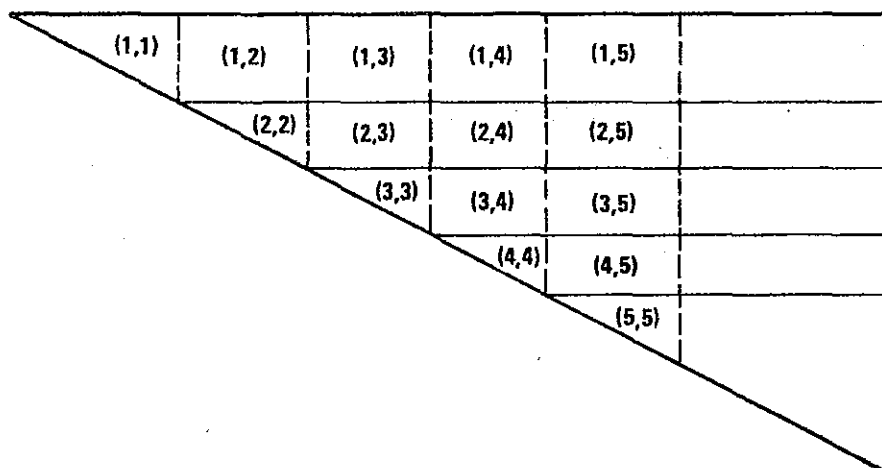
Figure 47. Representation of plant cells in CE-QUAL-R1
