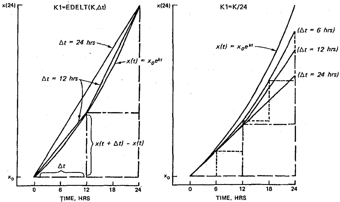
Figure 12. Rate transforms
