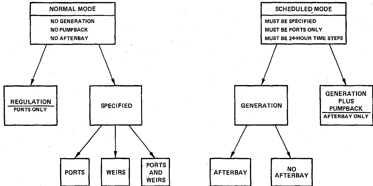
Figure 3. Options available in CE-QUAL-R1 to represent different reservoirs.
