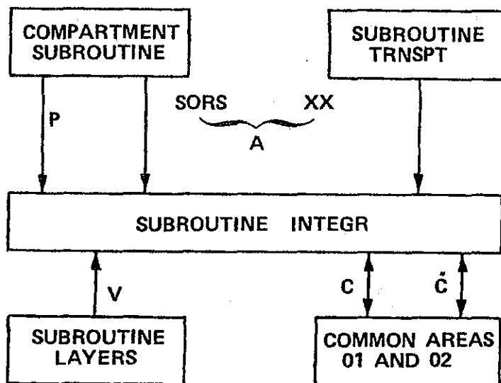
Figure 42. Mechanics of integration
