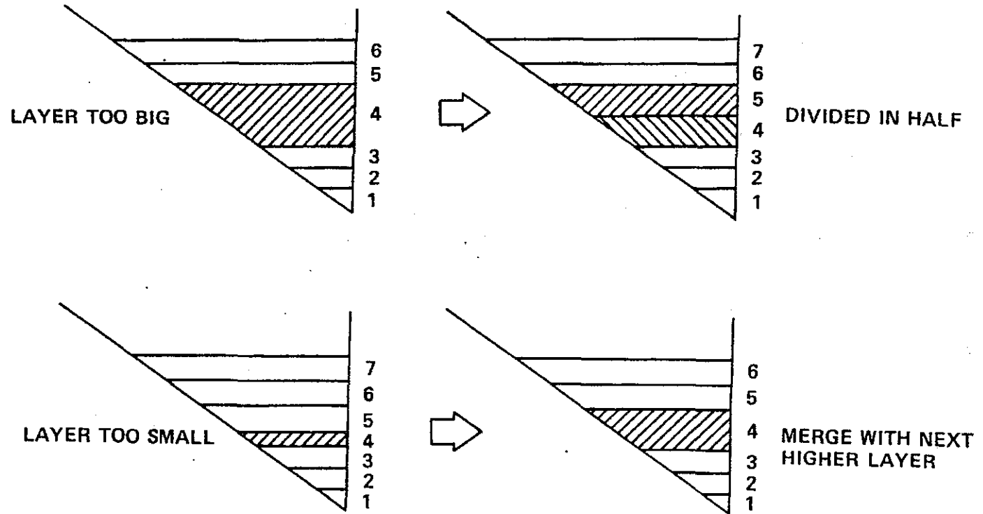
Figure 34. Resizing layers
