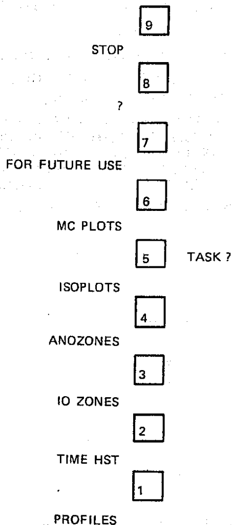
Figure 84. Graphics tasks
