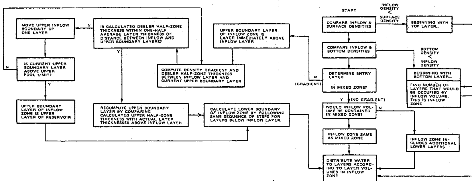
Figure 21. Subroutine FLOWIN
