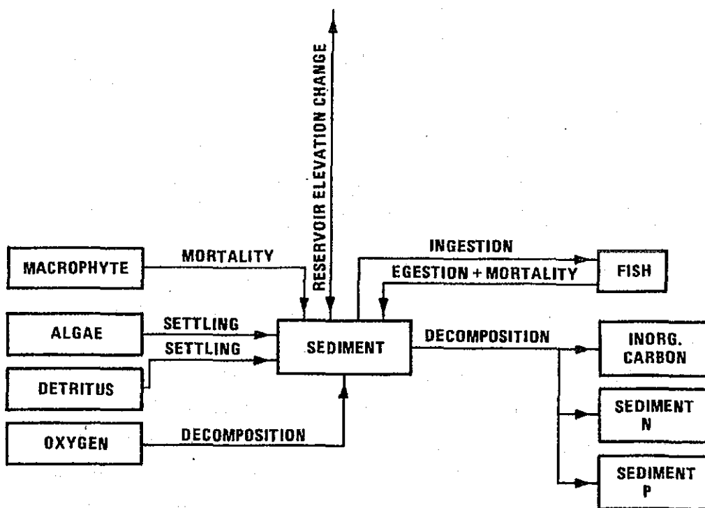
Figure 50. Fluxes for the sediment compartment
