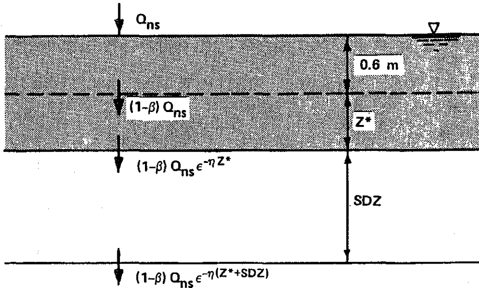
Figure 38. Solar radiation fluxes with depth
