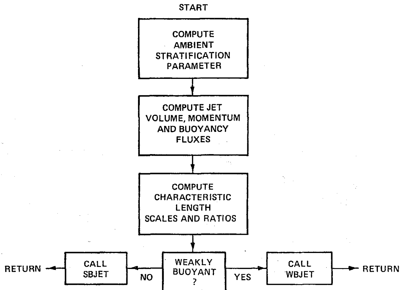
Figure 25. Flowchart for subroutine ENTRN
