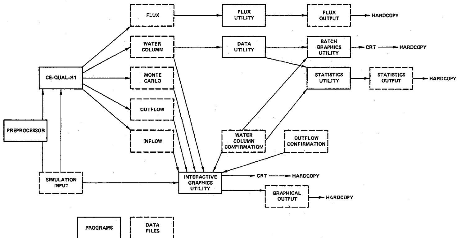
Figure 8. The relationship of computer programs and data files for CE-QUAL-R1
