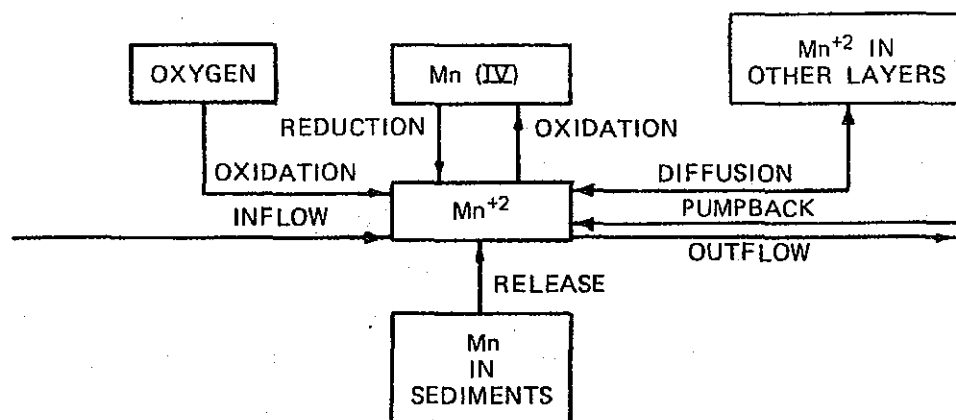
Figure 60. Fluxes for the reduced manganese compartment
