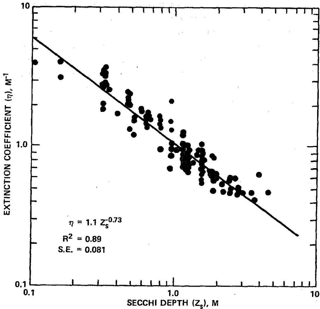
Figure 79. Relationship between the extinction coefficient and the Secchi disk depth (Williams et al. 1981)
