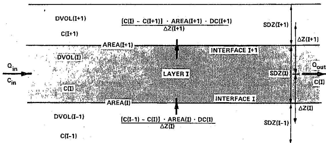
Figure 39. Elements of concentration-dependent transport
