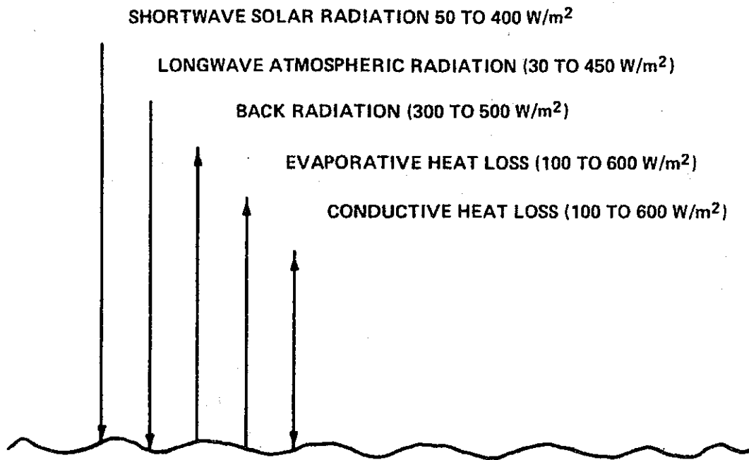
Figure 14. Principal components of the heat budget at the air-water interface (after Edinger, Brady, and Geyer 1974)
