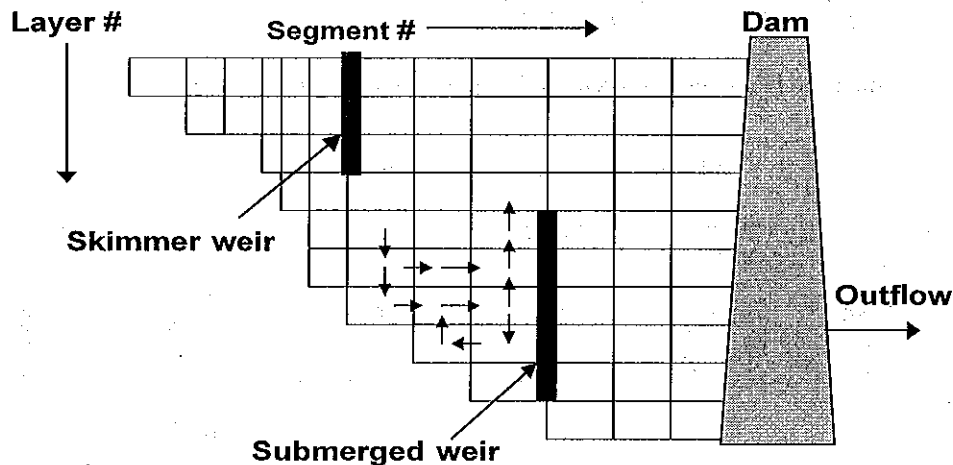
Figure A-42. Schematic representation of internal weirs.
