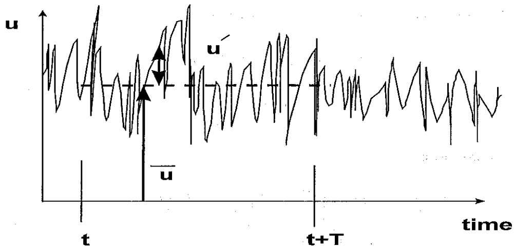
Figure A-17. Velocity variability with time.
