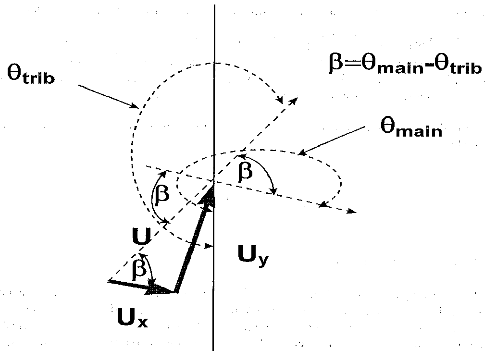
Figure A-16. Schematic of x and y velocity components.
