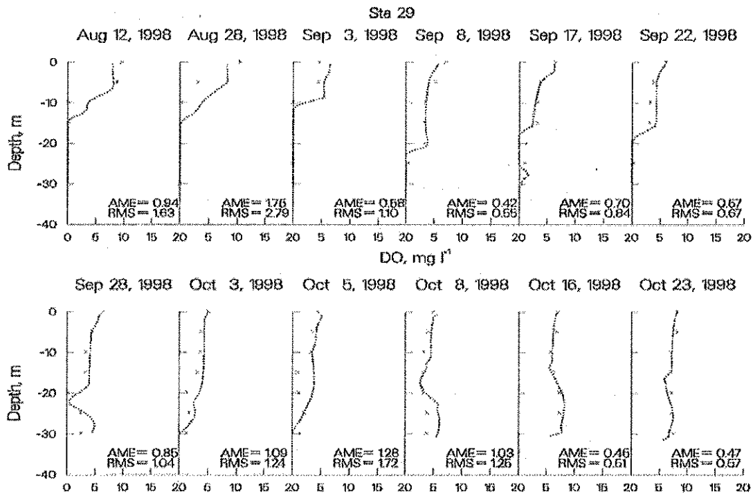
Figure 27. Shepaug Reservoir computed vs. observed DO.
