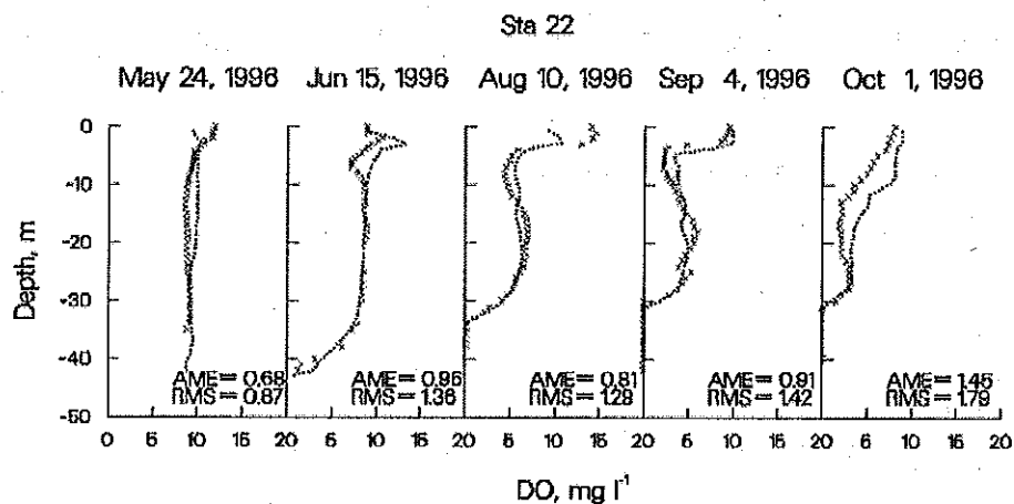
Figure 25. Rimov Reservoir computed vs. observed DO.
