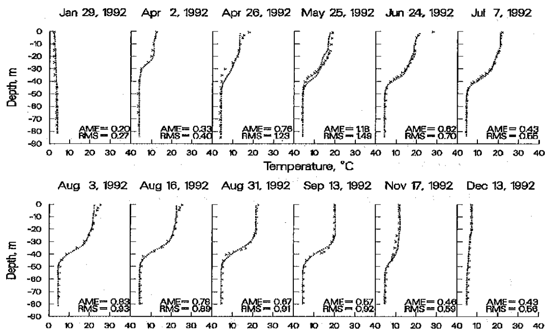
Figure 12. 1992 Brownlee Reservoir computed versus observed temperatures.
