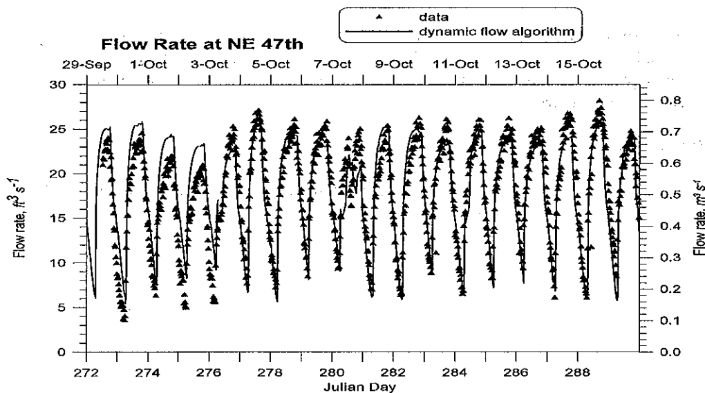
Figure A-41. Computed versus observed flow using dynamic culvert model.
