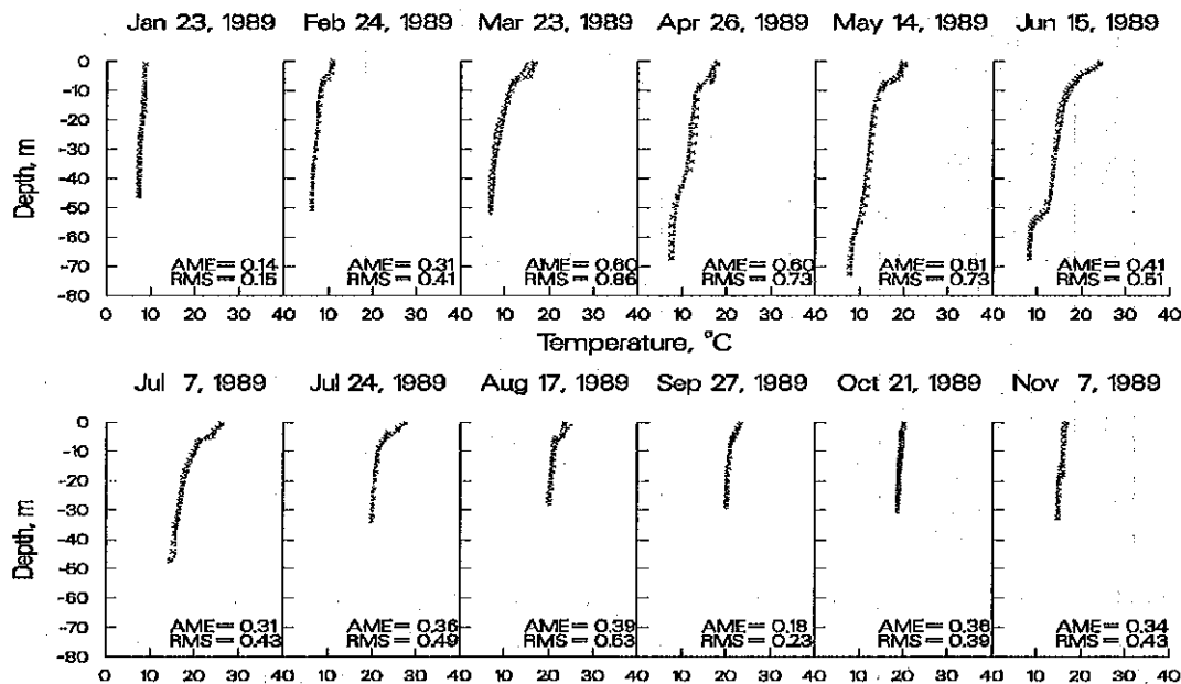
Figure 4. 1989 Pineflat Reservoir computed versus observed temperatures.
