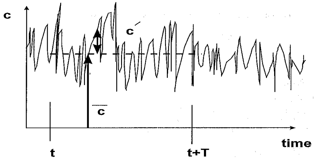
Figure A-18. Concentration variability with time.
