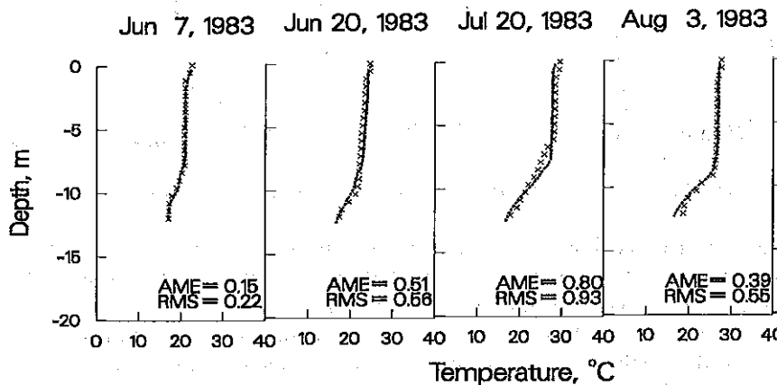
Figure 7. 1983 Bluestone Reservoir computed versus observed temperatures.
