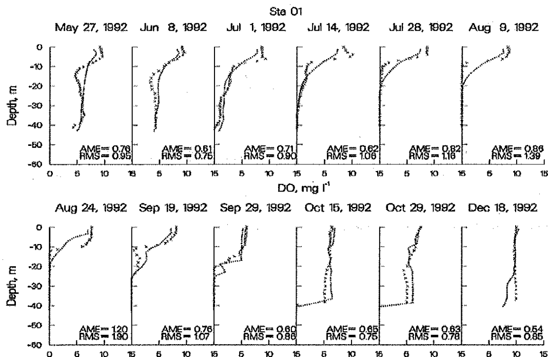
Figure 15. Allatoona Reservoir computed vs. observed DO.
