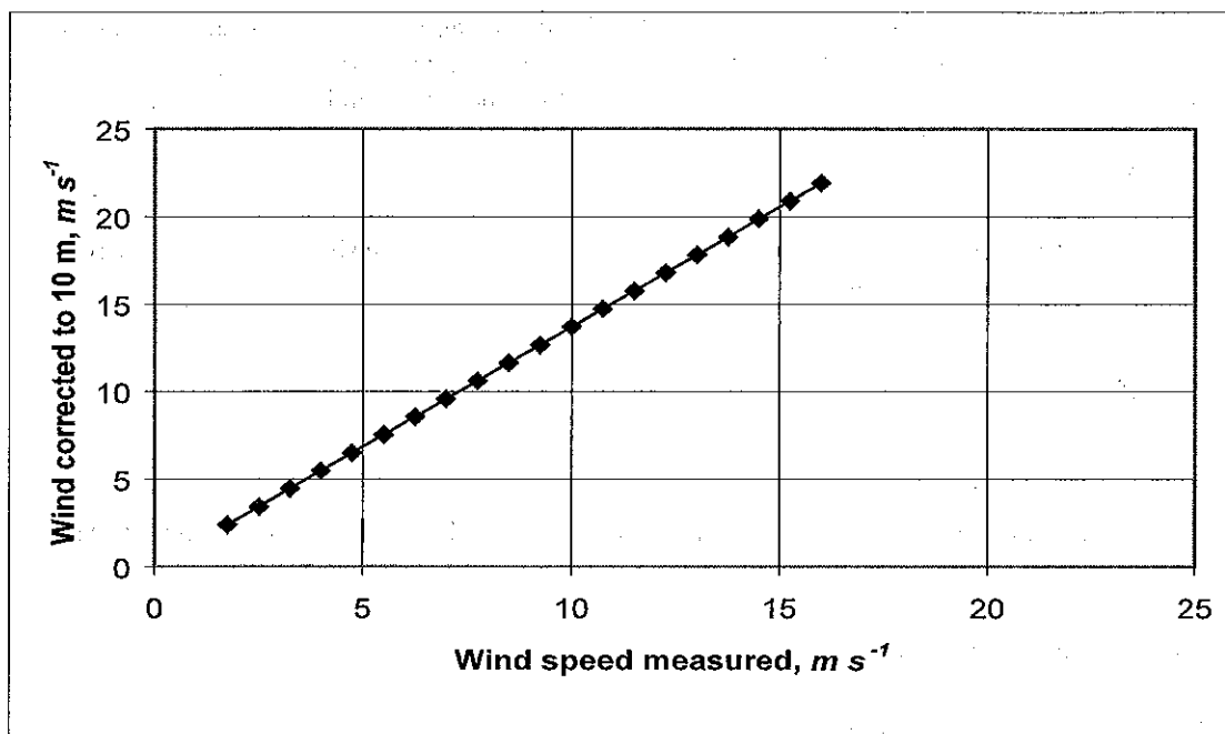
Figure B-24. Wind corrected to 10 m based on wind measured on land.
