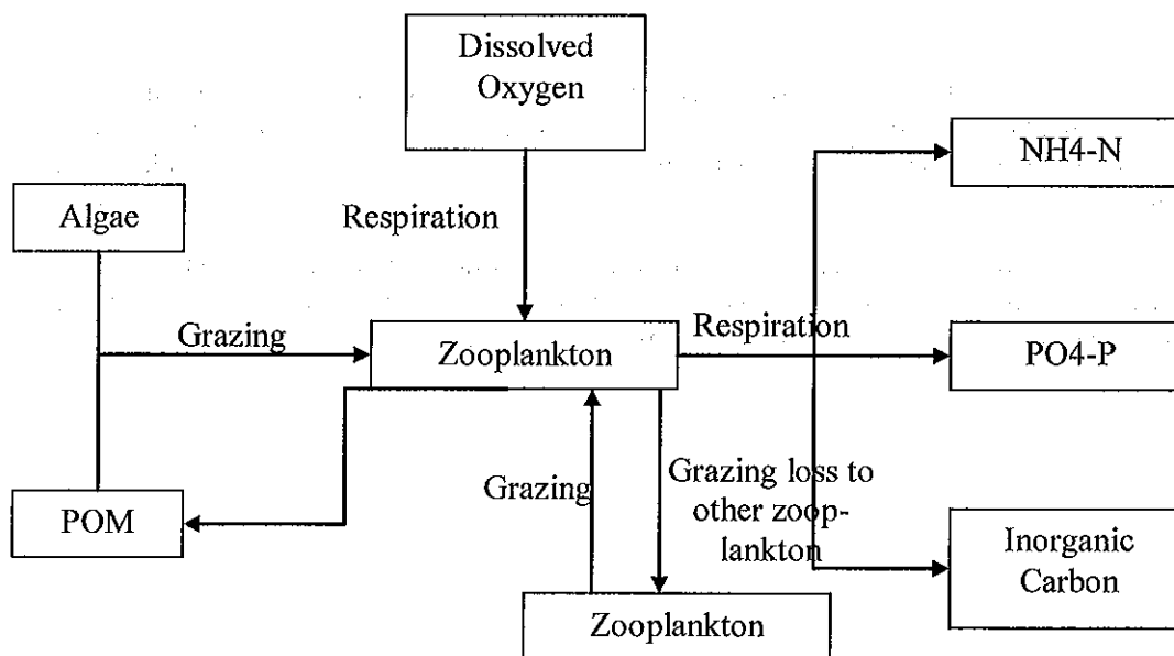
Figure 12. Zooplankton source/sinks.
