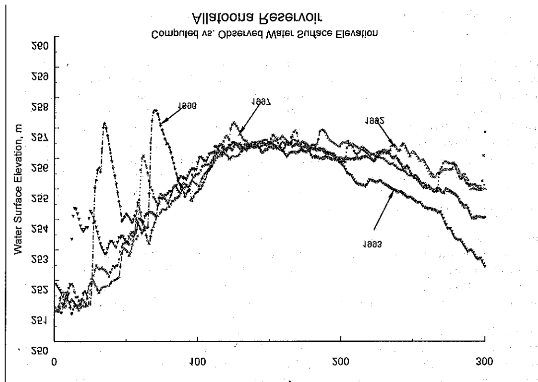
Figure 3. Allatoona Reservoir computed (lines) vs. observed (symbols) water surface elevations for 1992, 1993, 1996, and 1997.
