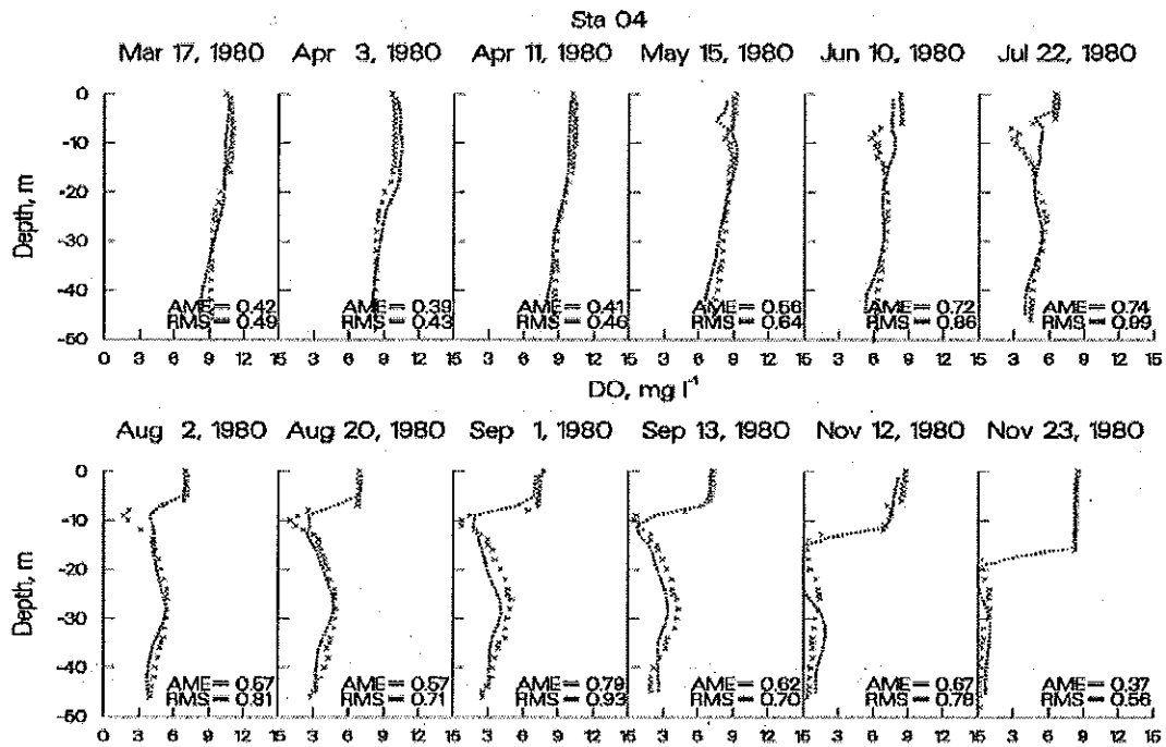
Figure 18. DeGray Reservoir computed vs. observed DO.
