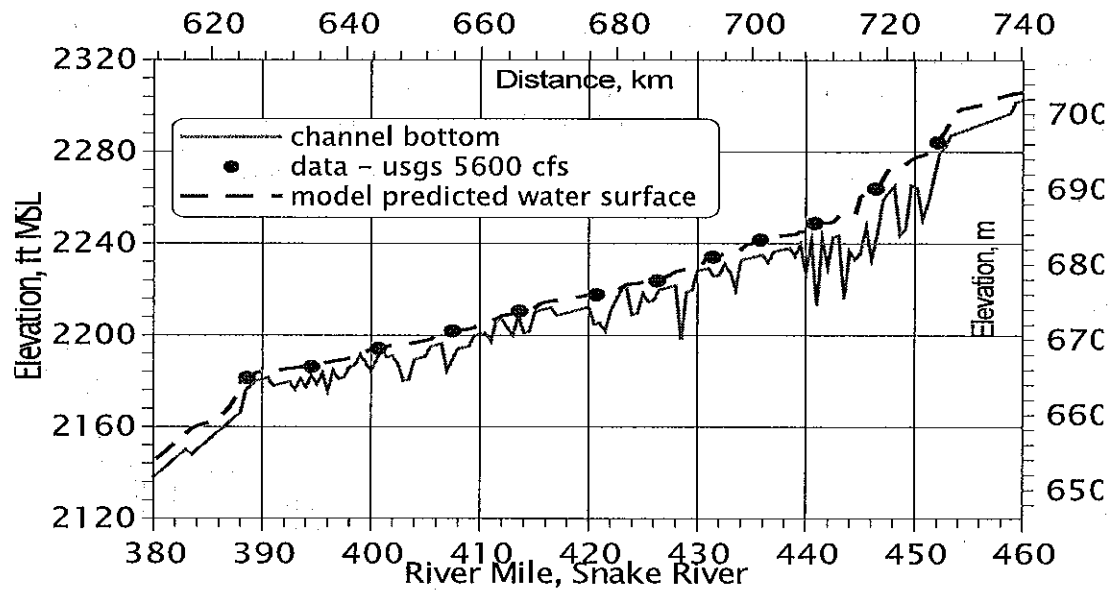
Figure 54. Snake River water level comparison between CE-QUAL-W2 V3 and USGS field data.
