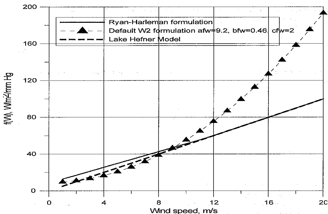
Figure A-49. Comparison of the wind speed formulation for Ryan-Harleman and W2 default (for T_{air}=15^{\circ}C , T_{dew}=-5^{\circ}C , T_{surface}=25^{\circ}C ).
