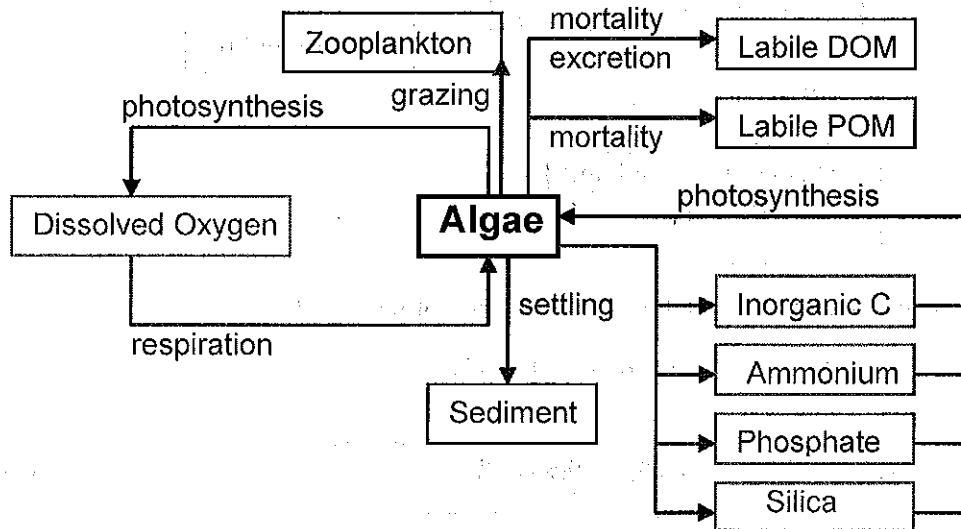
Figure B-9. Internal flux between algae and other compartments.
