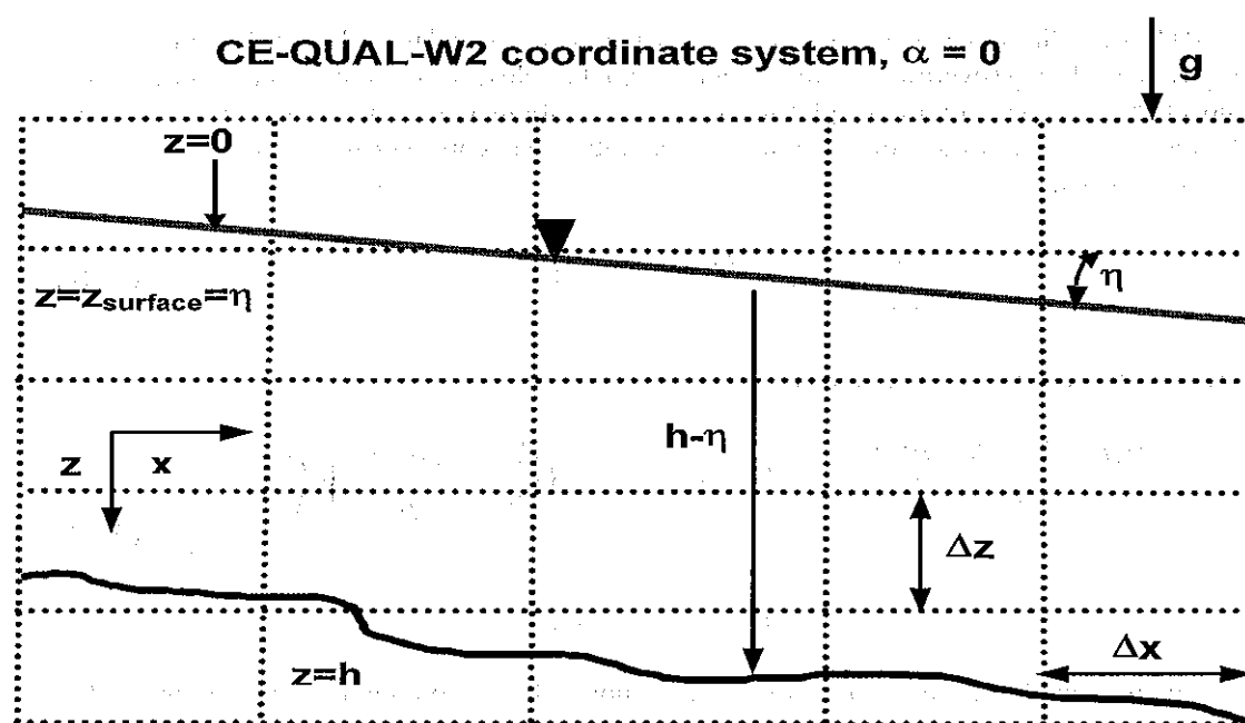
Figure A-10. Coordinate system without channel slope.
