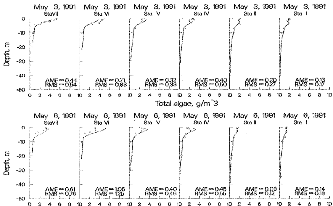
Figure 42. Rimov Reservoir computed vs. observed phytoplankton with wind rotated 90°.
