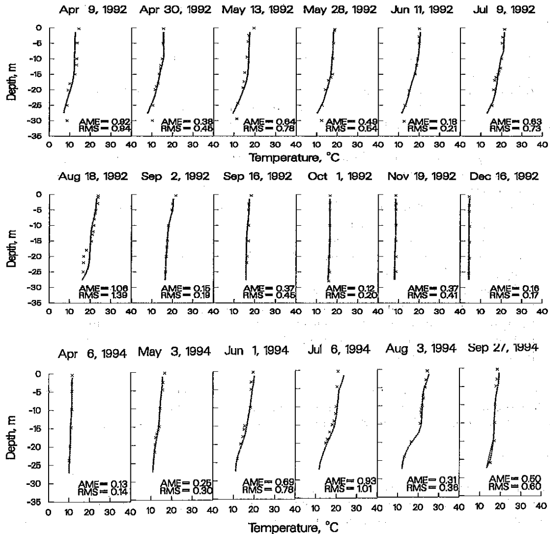
Figure 14. C.J. Strike Reservoir computed versus observed temperatures.
