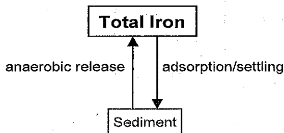
Figure B-18. Internal flux between total iron and other compartments.
