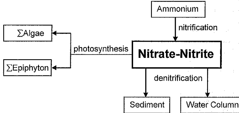
Figure B-15. Internal flux between nitrate + nitrite and other compartments.
