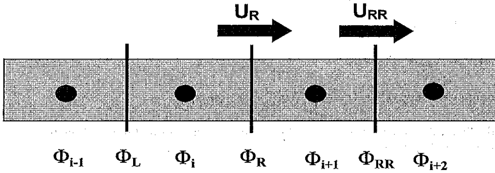
Figure A-26. Definition sketch for variable velocity.
