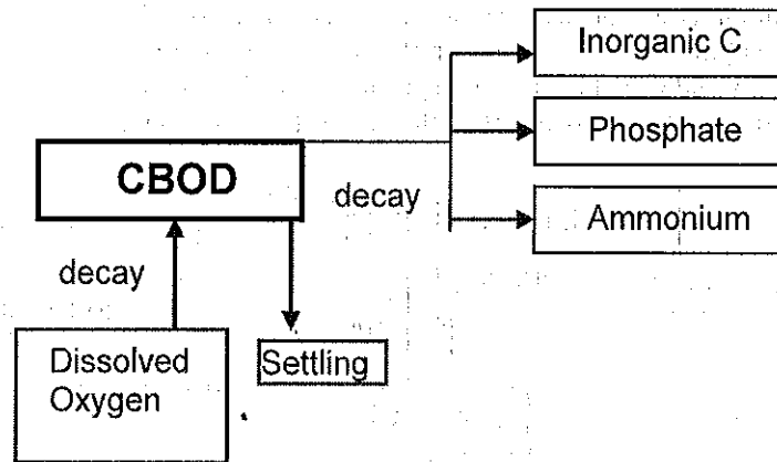
Figure B-8. Internal flux between CBOD and other compartments.
