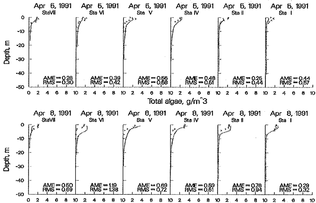
Figure 32. Rimov Reservoir computed vs. observed phytoplankton biomass.
