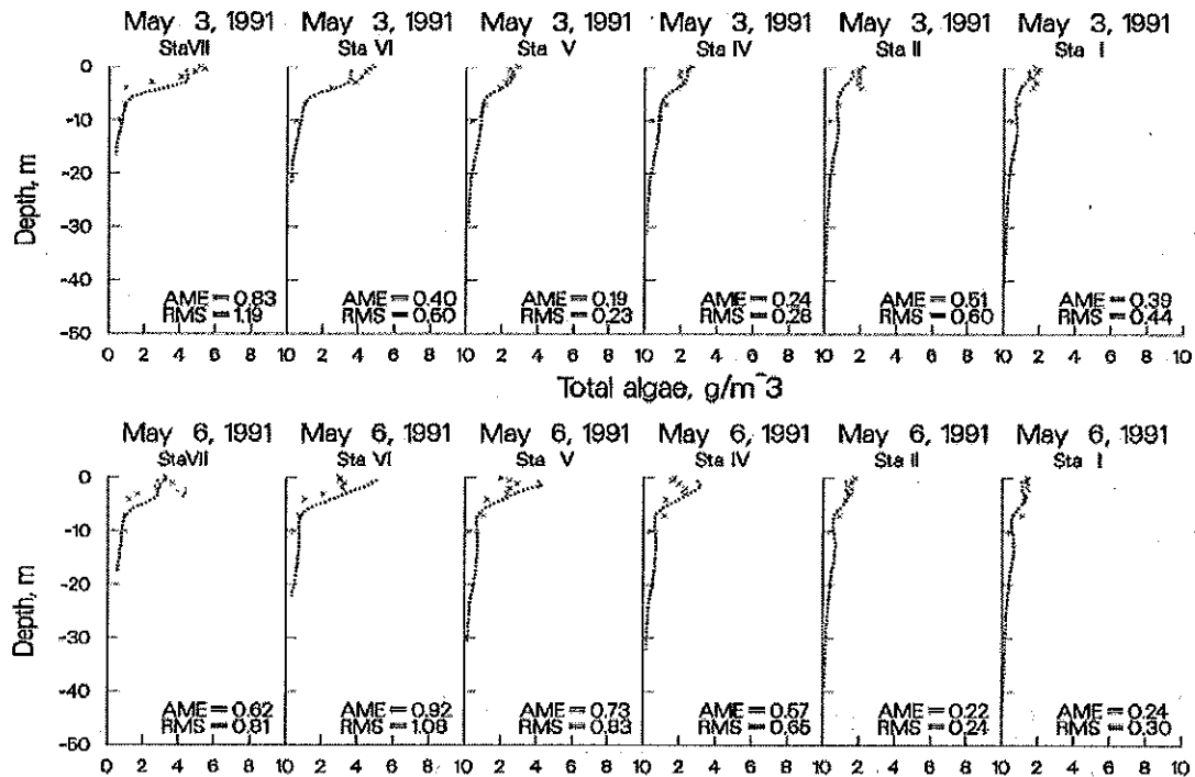
Figure 36. Rimov Reservoir computed vs. observed phytoplankton biomass.
