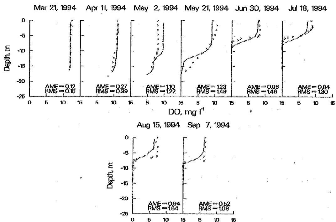
Figure 24. Monroe Reservoir computed vs. observed DO.
