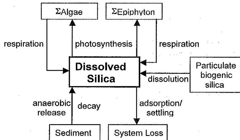
Figure B-16. Internal flux between dissolved silica and other compartments.
