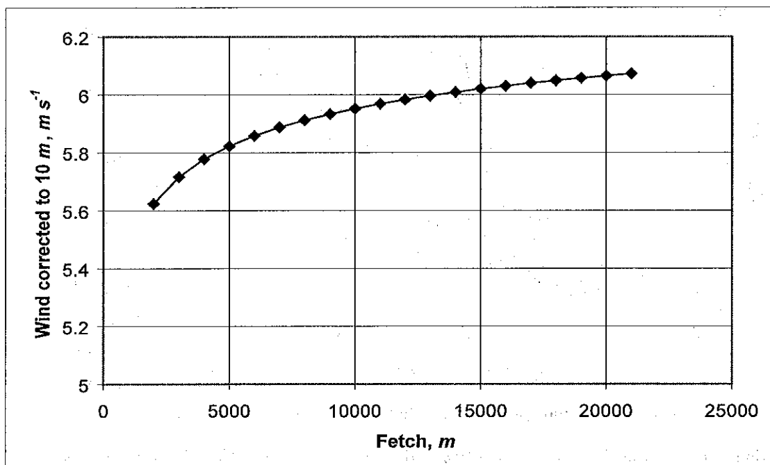
Figure B-23. Wind speed of 5 m s^{-1} corrected to 10 m as a function of fetch.
