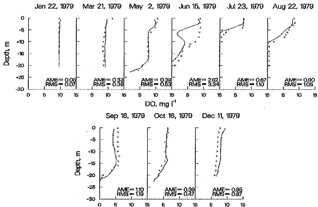
Figure 29. West Point Reservoir computed vs. observed DO.
