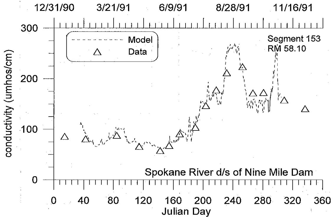
Figure 64. Spokane River computed versus observed conductivity below Nine Mile Dam.
