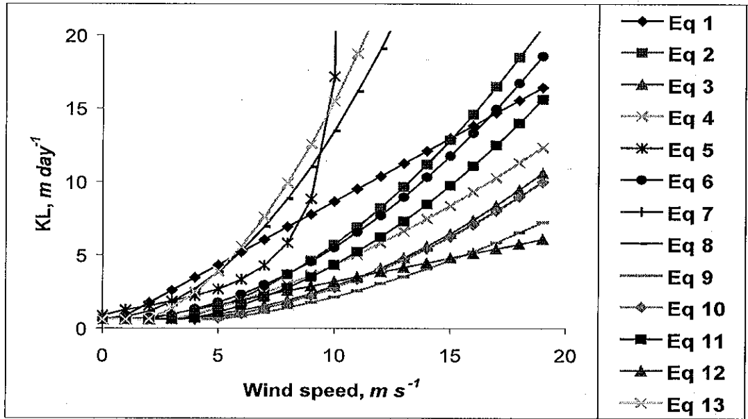
Figure B-21. Variation of wind speed and KL for lake/reservoir equations.
