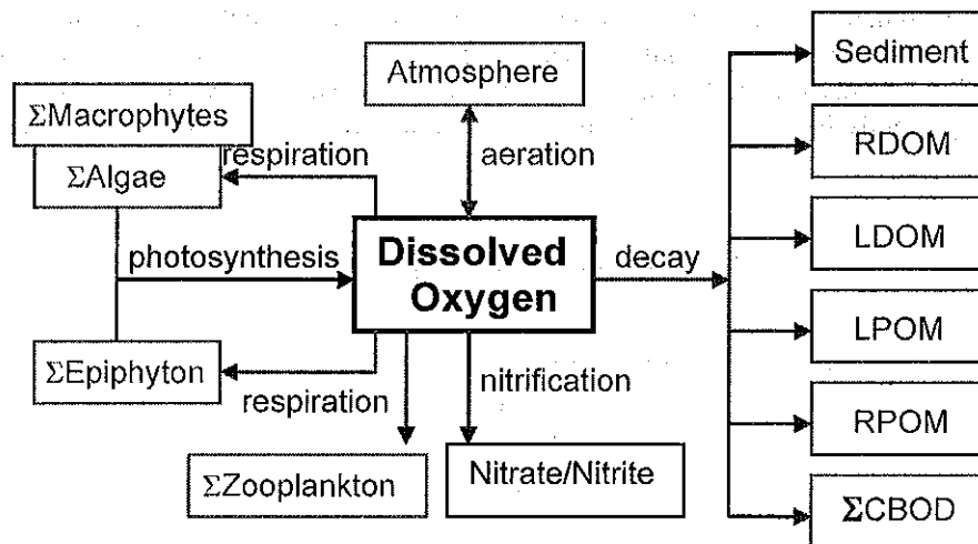
Figure B-19. Internal flux between dissolved oxygen and other compartments.
