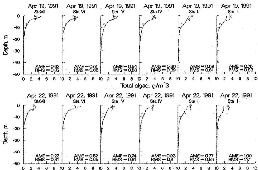
Figure 34. Rimov Reservoir computed vs. observed phytoplankton biomass.
