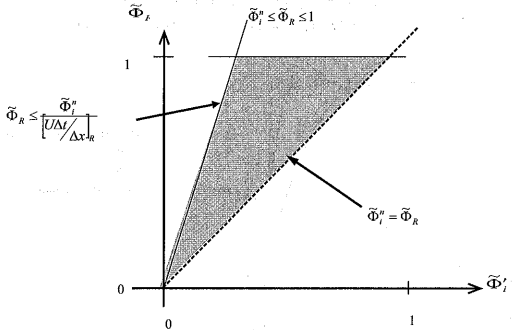
Figure A-24. Definition sketch for monotonic solution domain.
