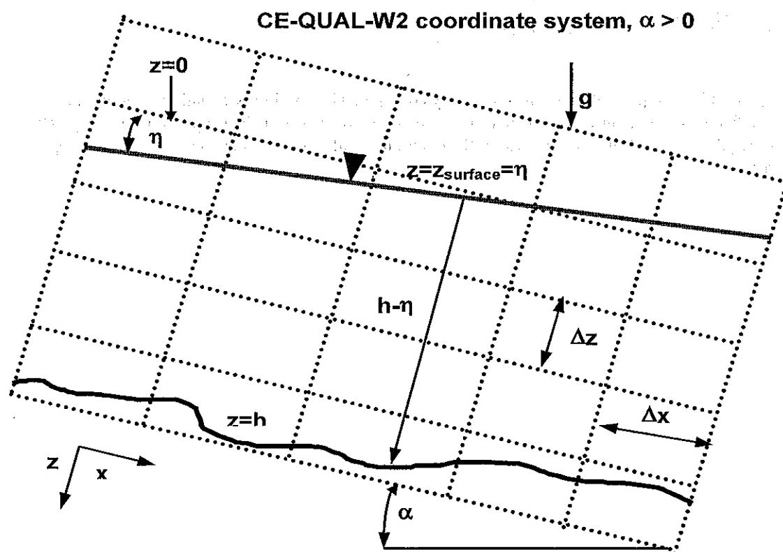
Figure A-11. Coordinate system with channel slope.
