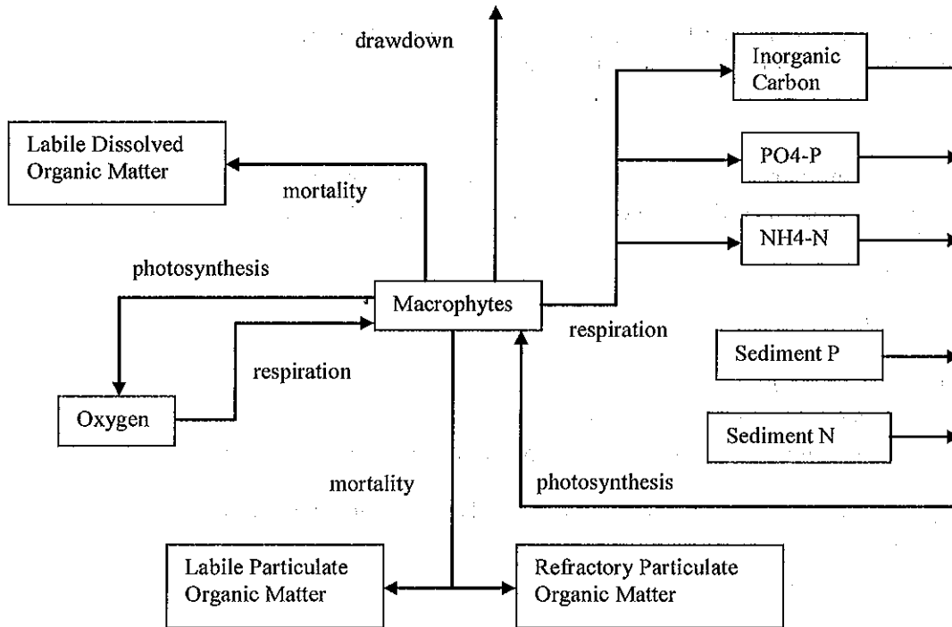
Figure 11. Nutrient fluxes for the macrophyte compartment in CE-QUAL-W2.
