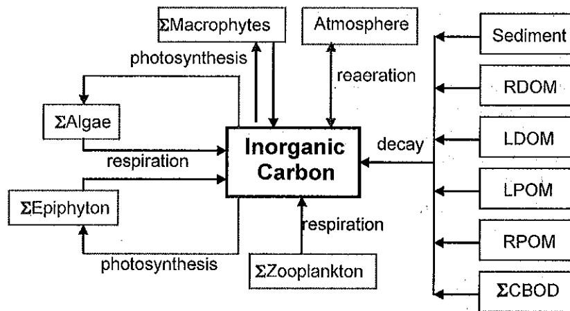
Figure B-28. Internal flux between inorganic carbon and other compartments.
