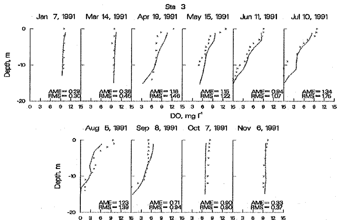
Figure 28. Weiss Reservoir computed vs. observed DO.
