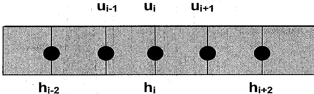
Figure A-40. Linkage schematic of model segments with a culvert.
