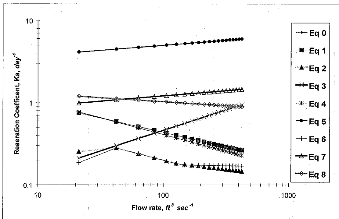
Figure B-20. Reaeration coefficient as a function of flow rate.
