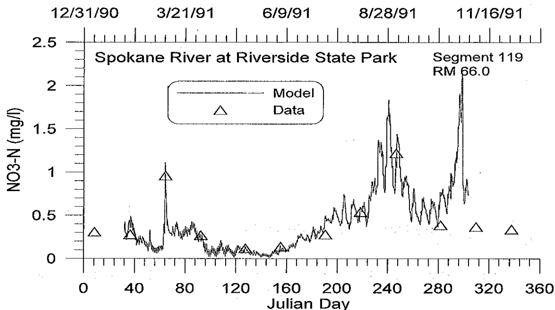
Figure 73. Spokane River computed versus observed nitrate-nitrite at Riverside State Park.
