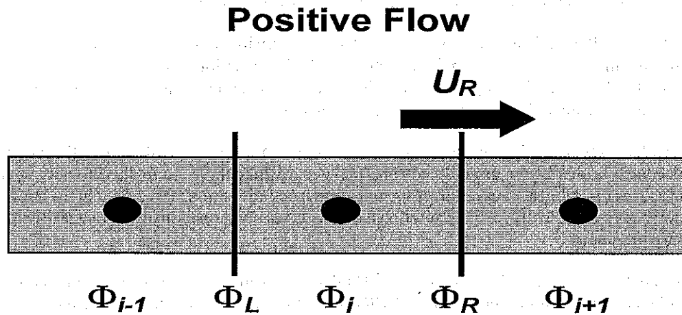
Figure A-22. ULTIMATE schematization for positive flow.
