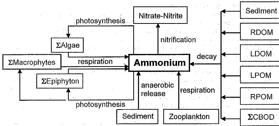
Figure B-14. Internal flux between ammonium and other compartments.
