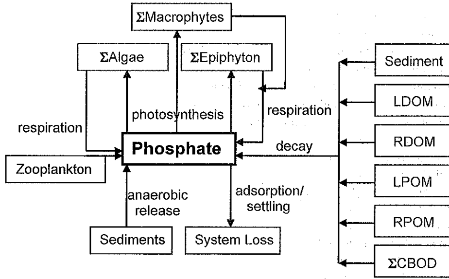
Figure B-13. Internal flux between phosphorus and other compartments.
