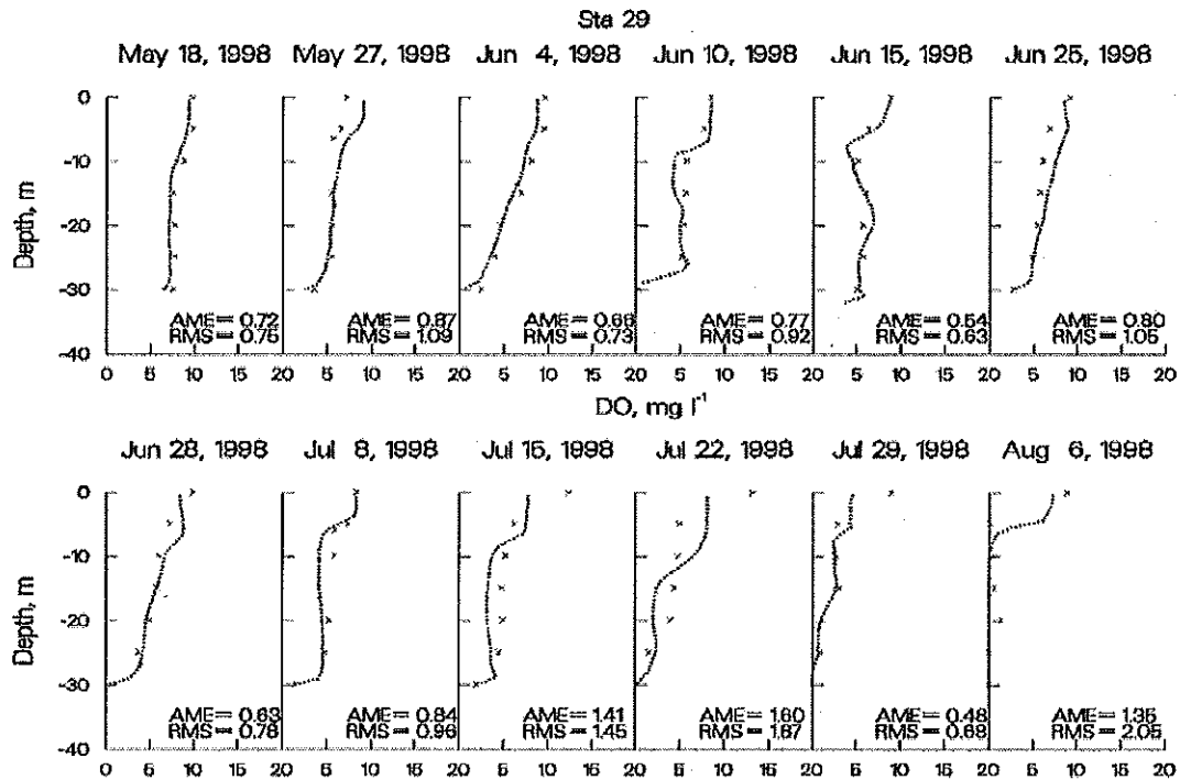
Figure 26. Shepaug Reservoir computed vs. observed DO.
