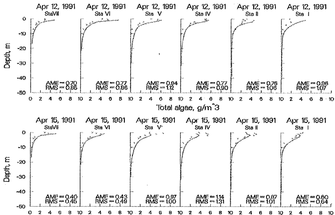
Figure 33. Rimov Reservoir computed vs. observed phytoplankton biomass.
