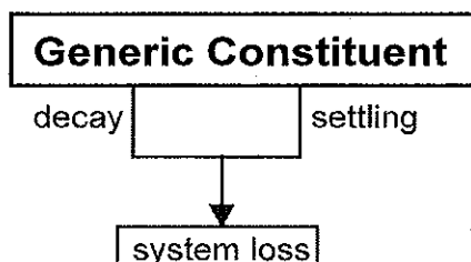
Figure B-1. Internal flux for generic constituent compartment.
