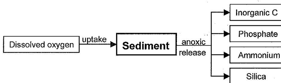
Figure B-26. Internal flux between 0-order sediment compartment and other compartments.
