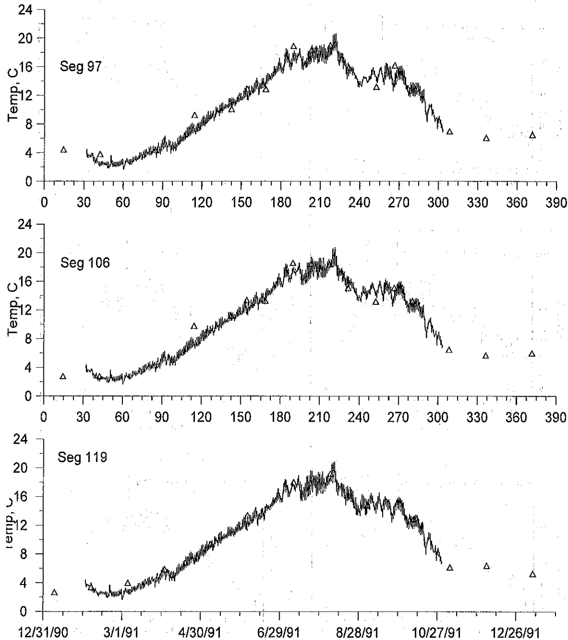
Figure 63. Computed versus observed temperatures for the Spokane River at Stateline Bridge (upstream boundary), City of Spokane, Fort Wright Bridge, and Riverside State Park.
