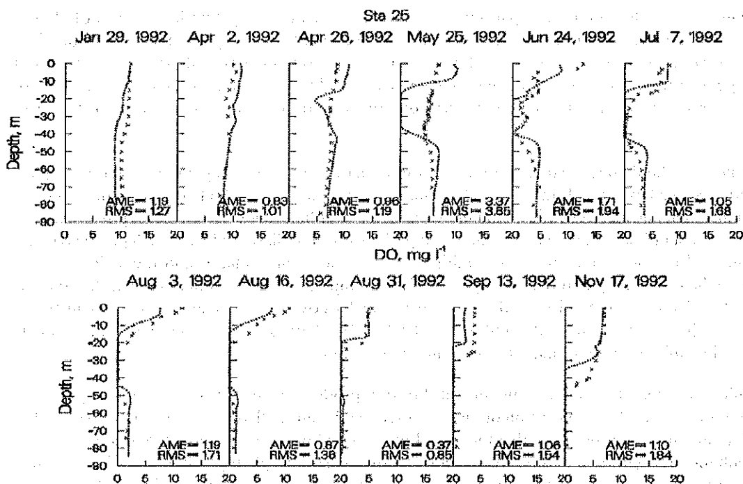
Figure 16. Brownlee Reservoir computed vs. observed DO.
