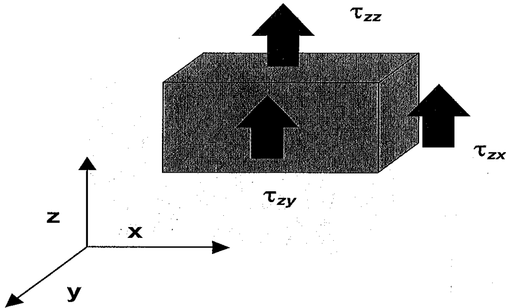
Figure A-5. Sketch of turbulent shear stresses in z-direction.
