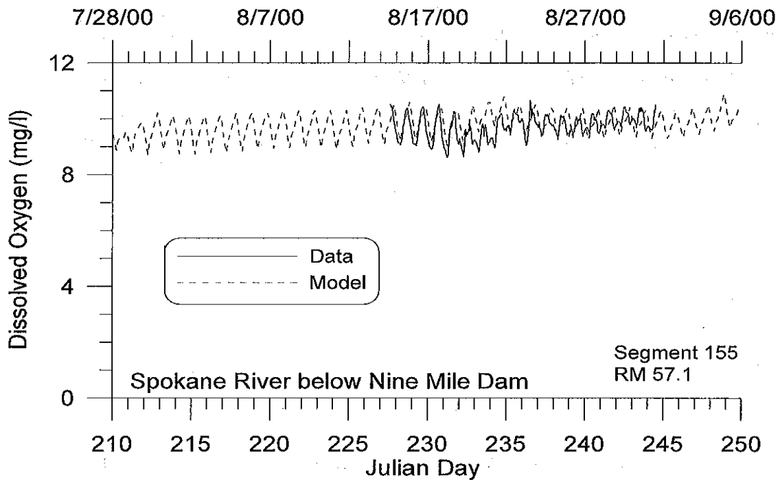
Figure 71. Spokane River computed versus observed dissolved oxygen below Nine Mile Dam.
