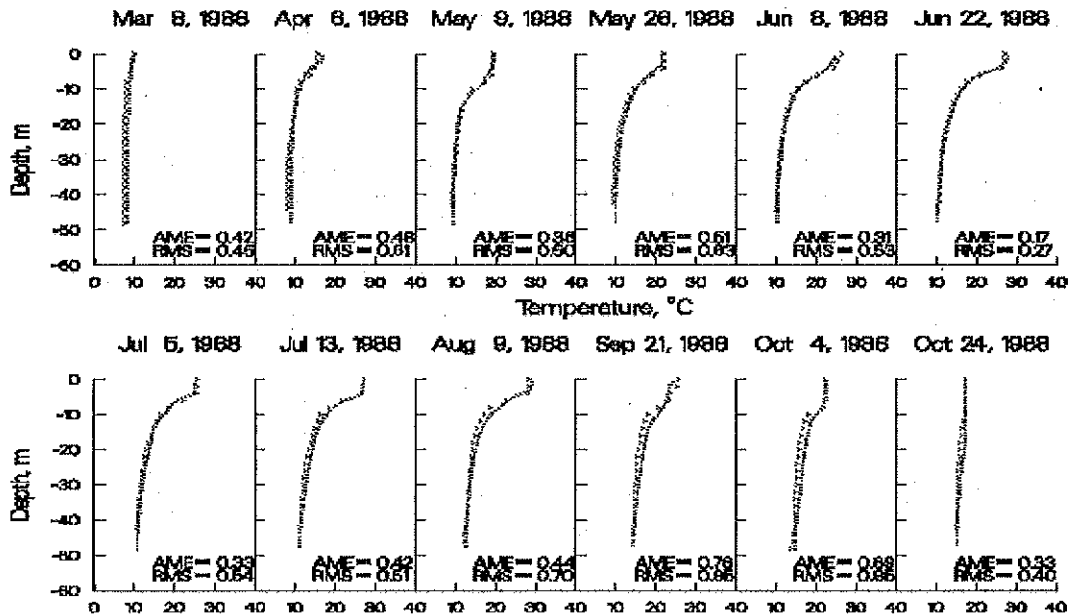
Figure 8. 1988 Richard B. Russell computed versus observed temperatures.
