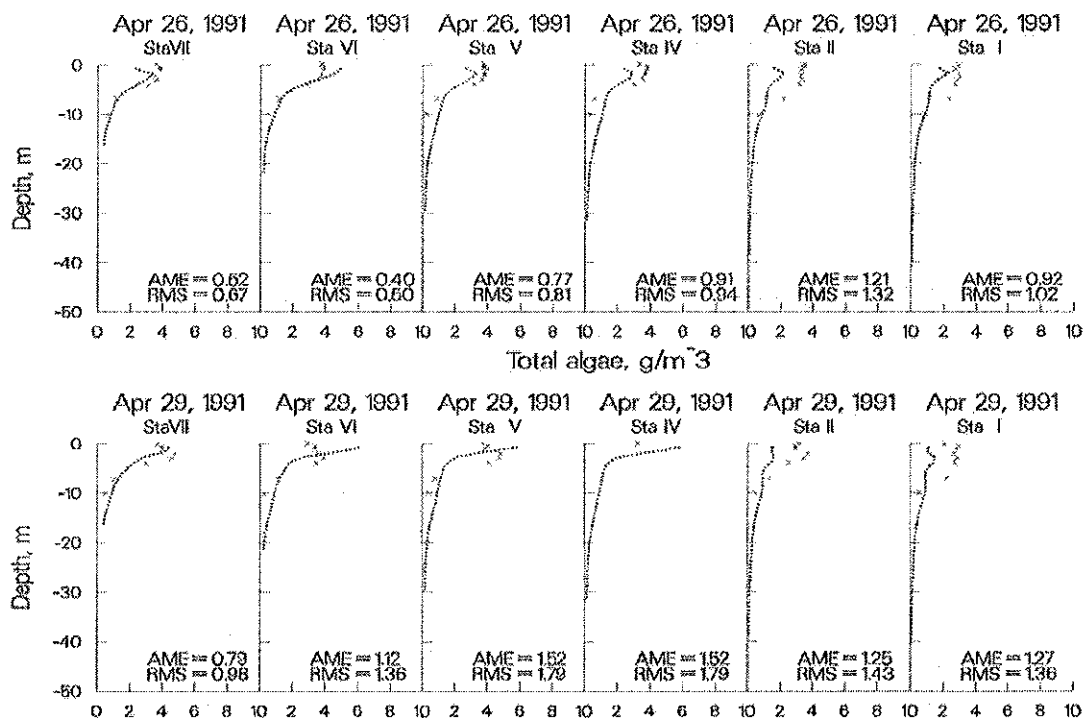
Figure 35. Rimov Reservoir computed vs. observed phytoplankton biomass.
