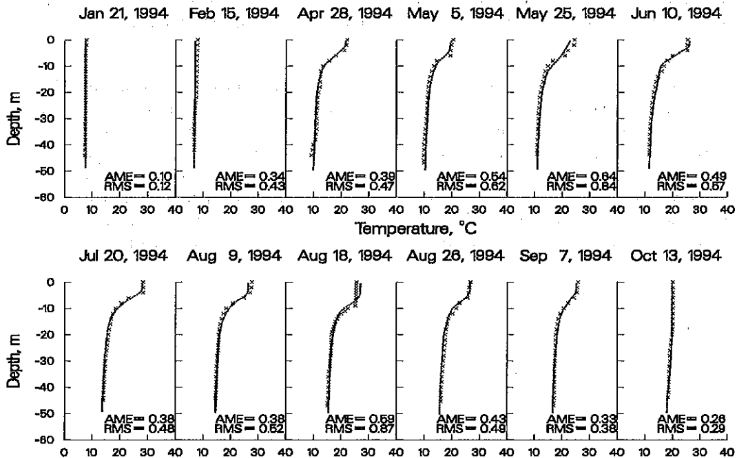
Figure 9. 1994 Richard B. Russell computed versus observed temperatures.
