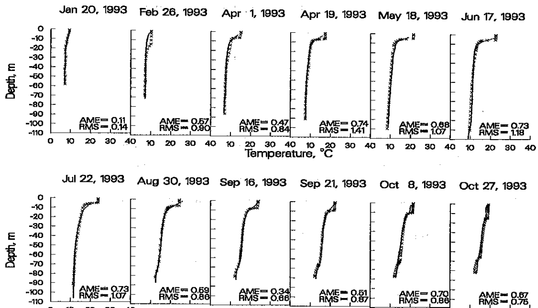
Figure 5. 1993 Pineflat Reservoir computed versus observed temperatures.
