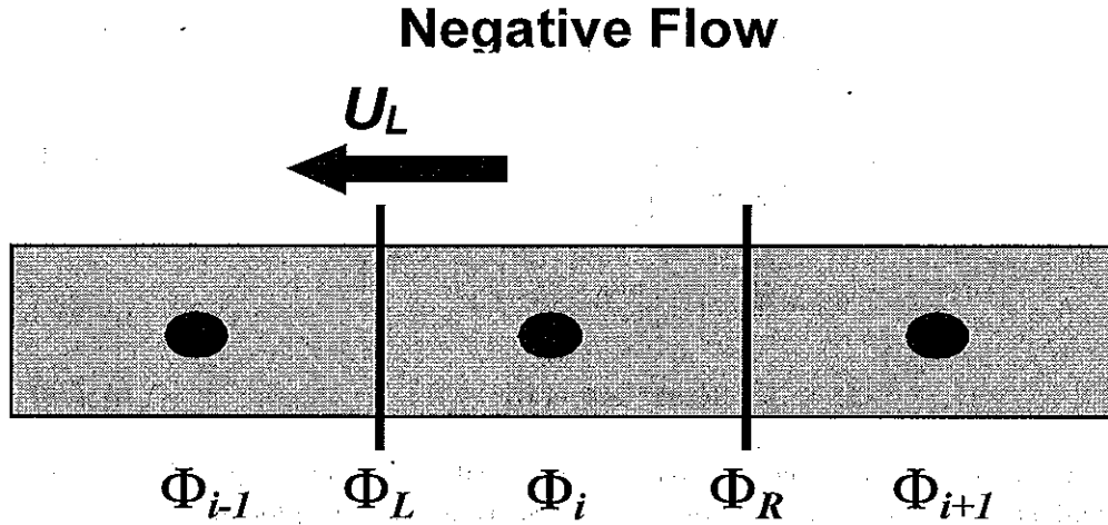
Figure A-23. ULTIMATE schematization for negative flow.
