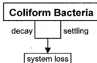
Figure B-2. Internal flux for coliform bacteria.
