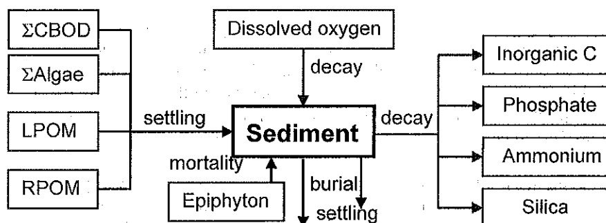
Figure B-27. Internal flux between 1 st -order sediment compartment and other compartments.
