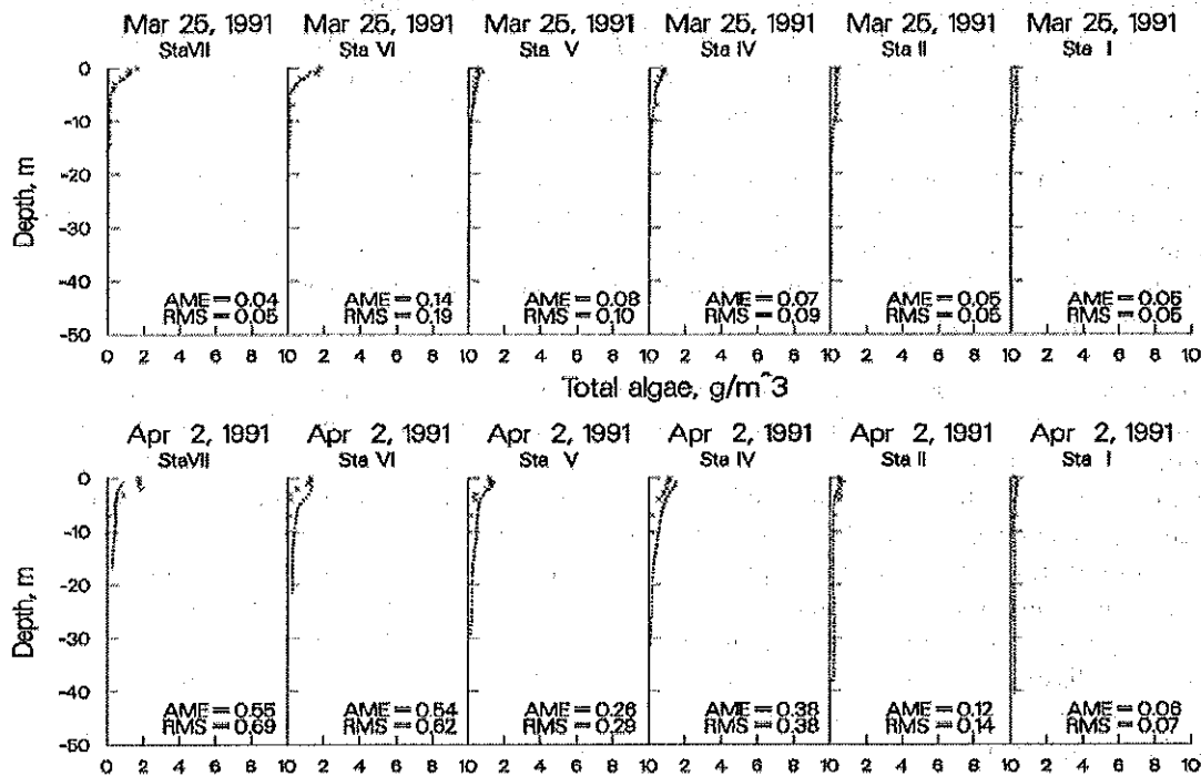
Figure 31. Rimov Reservoir computed vs. observed phytoplankton biomass.
