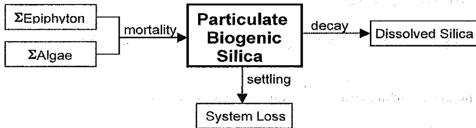
Figure B-17. Internal flux between particulate biogenic silica and other compartments
