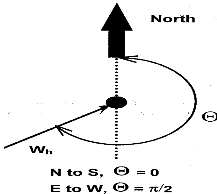
Figure A-29. Wind orientation.
