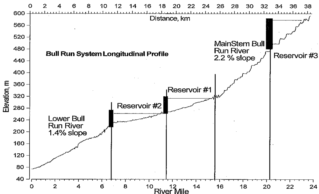
Figure 57. Channel slope for the Bull Run system.
