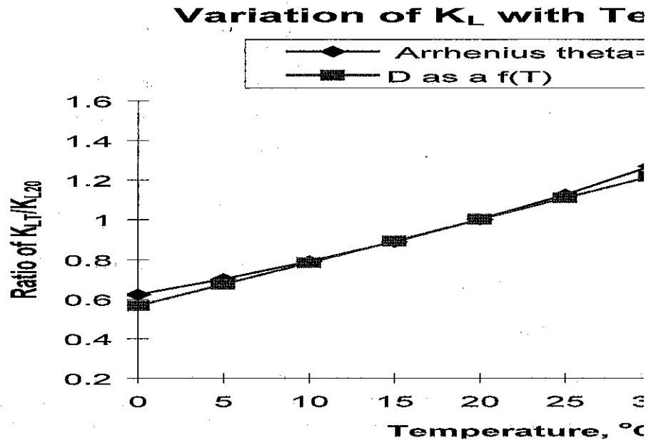
Figure B-25. Variation of K_{LT}/K_{L20} as a function of temperature.
