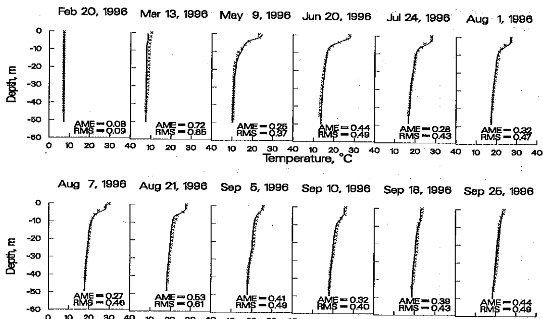
Figure 10. 1996 Richard B. Russell computed versus observed temperatures.
