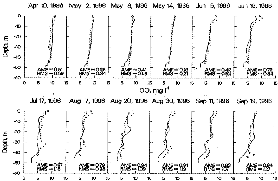
Figure 21. 1996 Richard B. Russell computed vs. observed DO.
