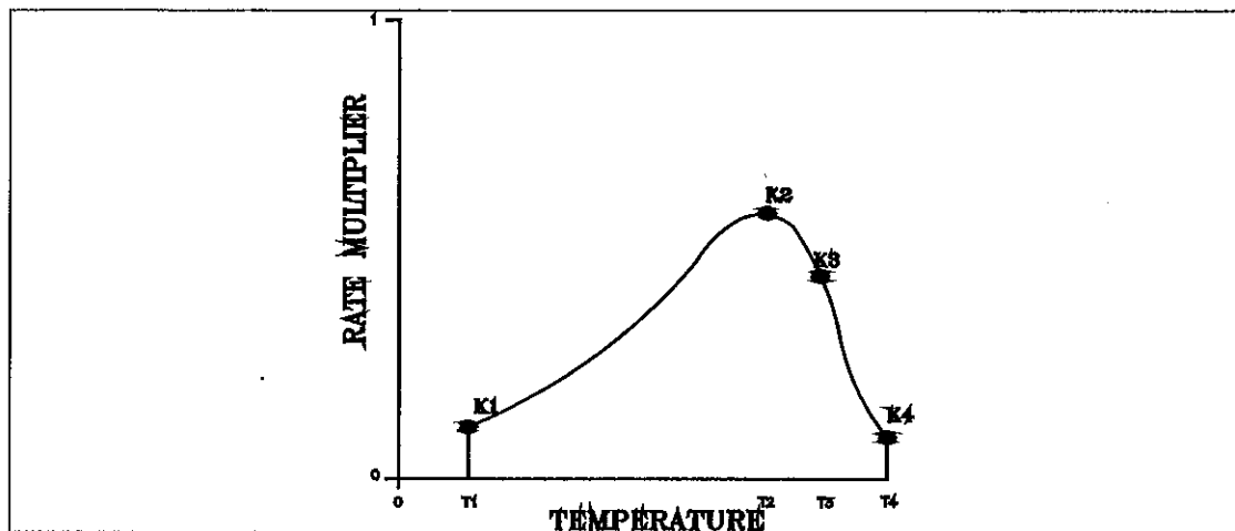
Figure B-29. Temperature rate multiplier function.
