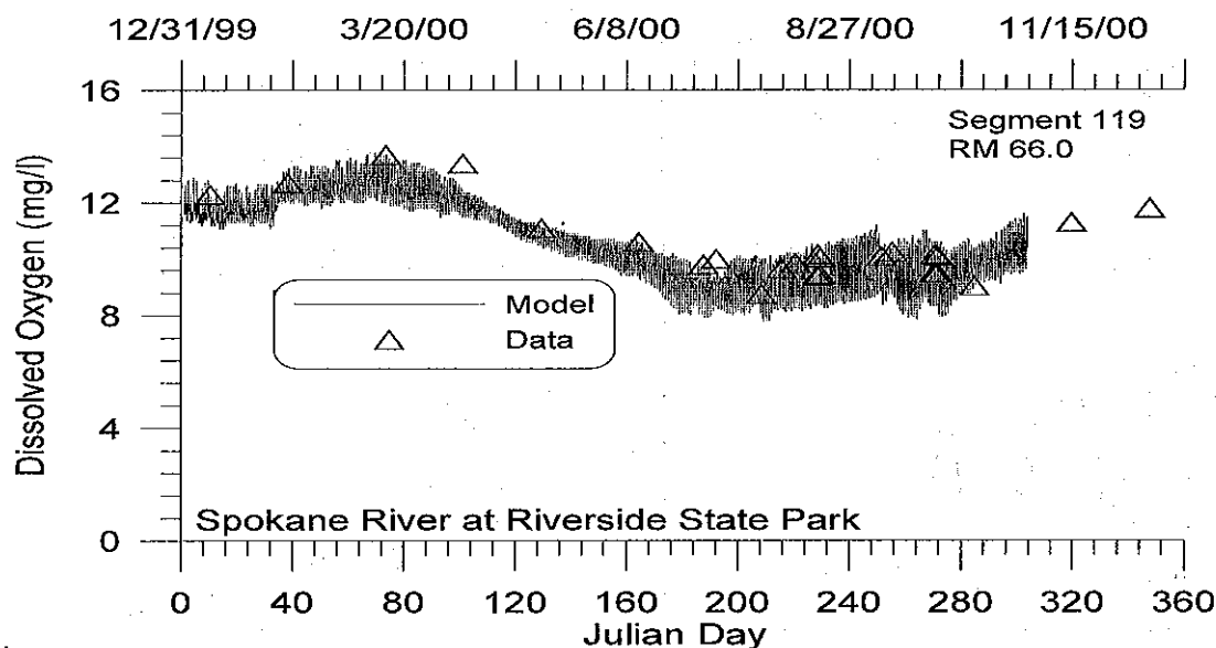
Figure 70. Spokane River computed versus observed dissolved oxygen at Riverside State Park.
