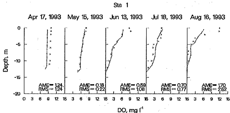
Figure 22. Neely Henry Reservoir computed vs. observed DO.
