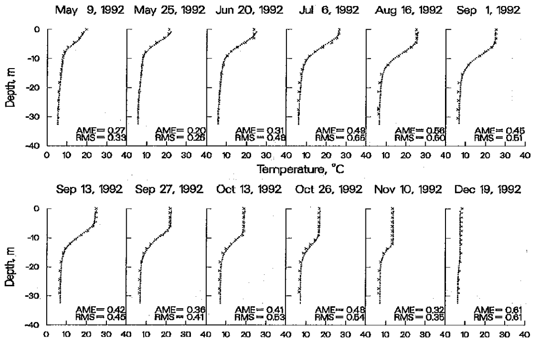
Figure 11. Paintsville Reservoir computed versus observed temperatures.
