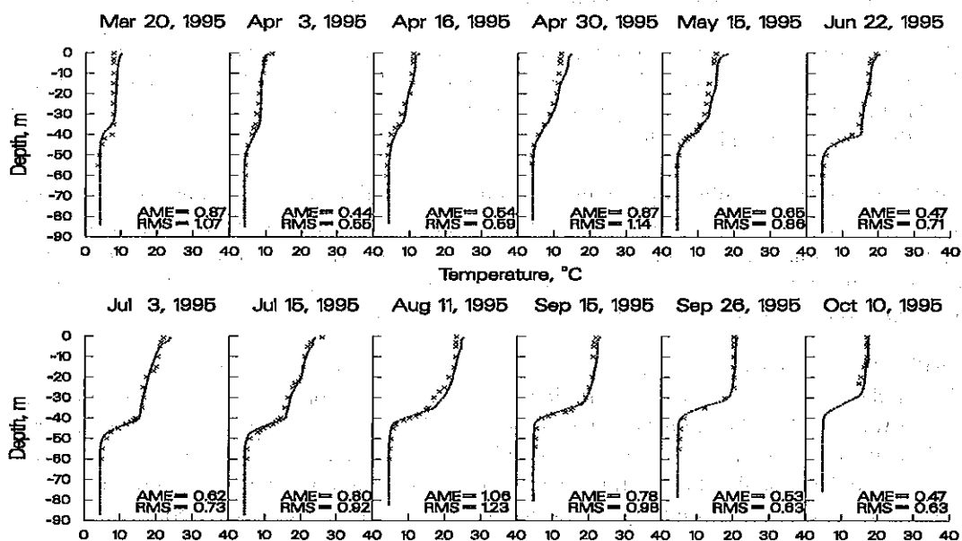
Figure 13. 1995 Brownlee Reservoir computed versus observed temperatures.
