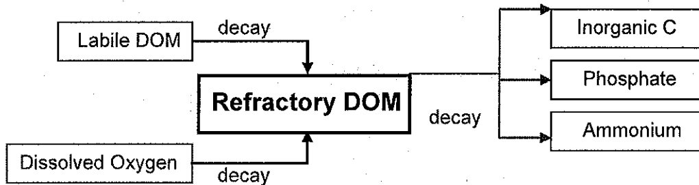
Figure B-5. Internal flux between refractory DOM and other compartments.
