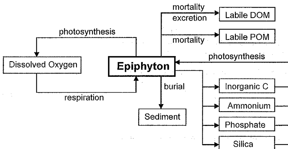
Figure B-10. Internal flux between epiphyton and other compartments.
