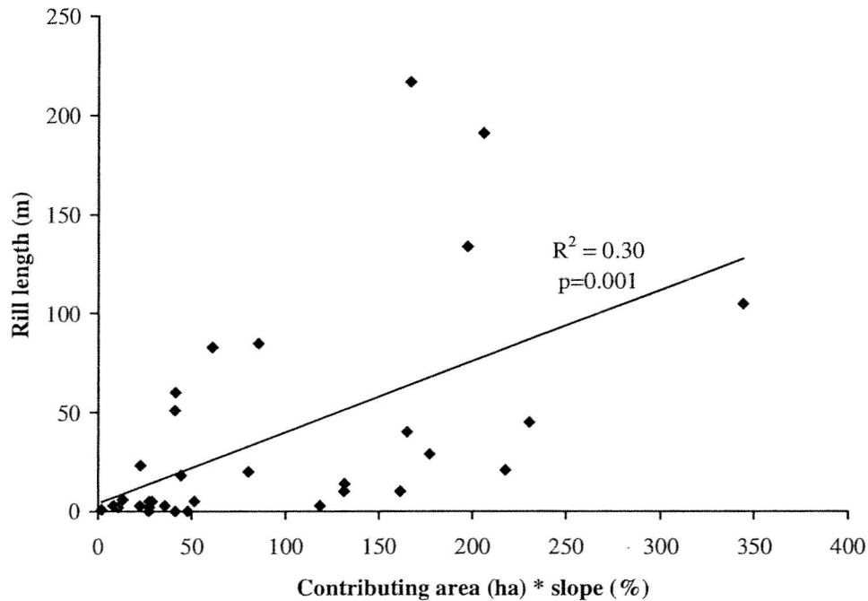
Figure 15. Rill length in summer 2004 versus contributing area times slope.
