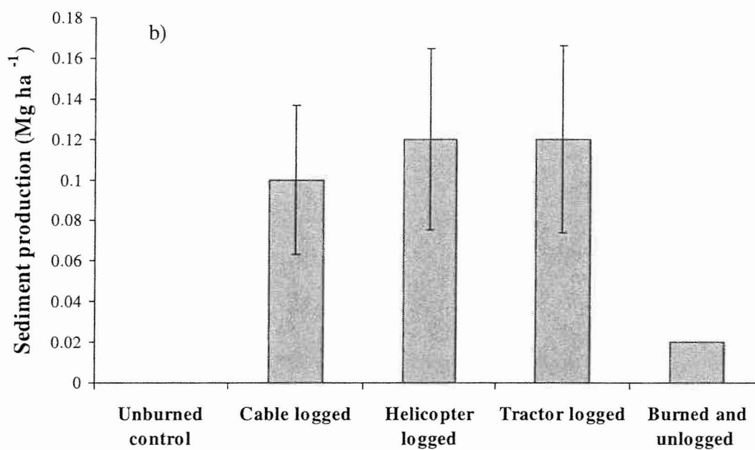
Figure 13. Sediment production rates by treatment for: a) 2002-2003 wet season, and b) 2003-2004 wet season. Bars represent one standard error.
