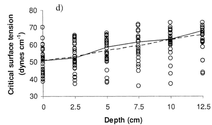
Figure 11. Critical surface tension (CST) values by depth for: a) unburned sites (mean of 2002-2004; n=5 ); b) burned sites in 2002 ( n=32 ); c) burned sites in 2003 ( n=32 ); and d) burned sites in 2004 ( n=32 ). Each circle represents the average value at a site. The mean values are plotted as dashed lines and median values are plotted as solid lines. A decrease in CST indicates stronger water repellency.
