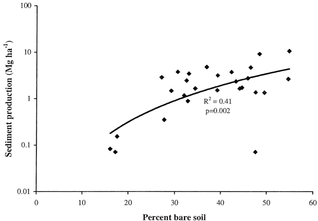
Figure 16. Sediment production versus percent bare soil for the 2002-2003 wet season.
