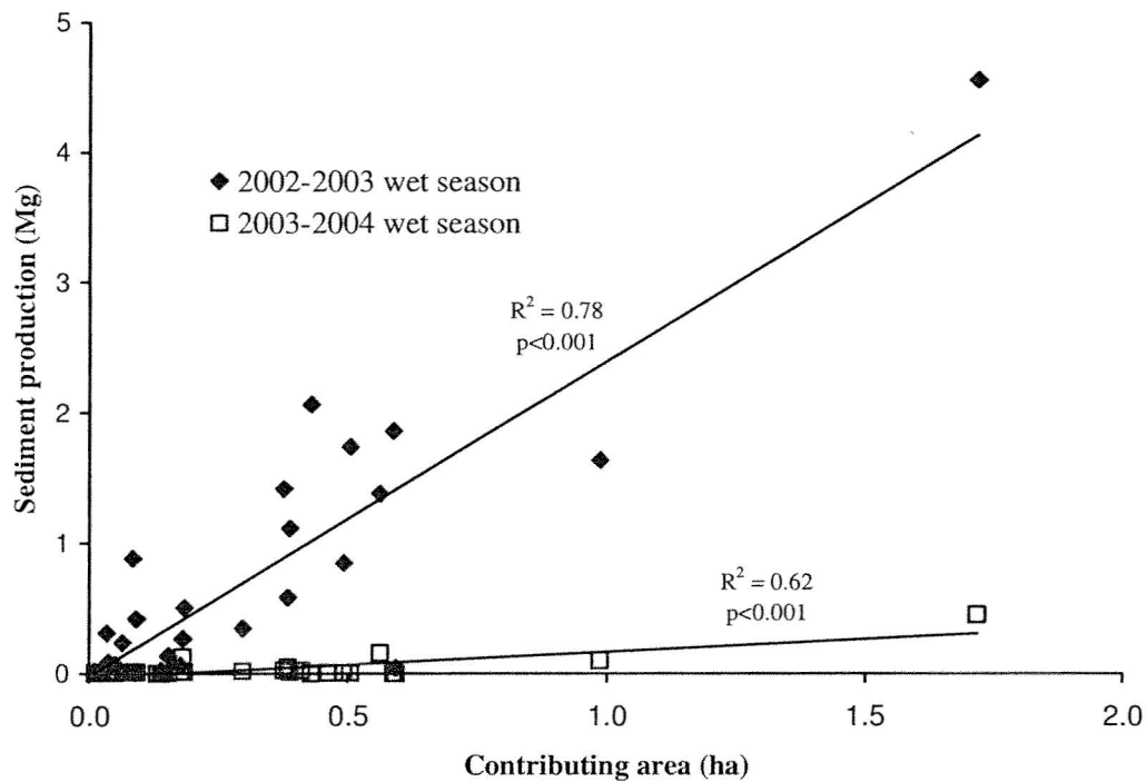
Figure 12. Sediment production versus contributing area for the 2002-2003 and 2003-2004 wet seasons.
