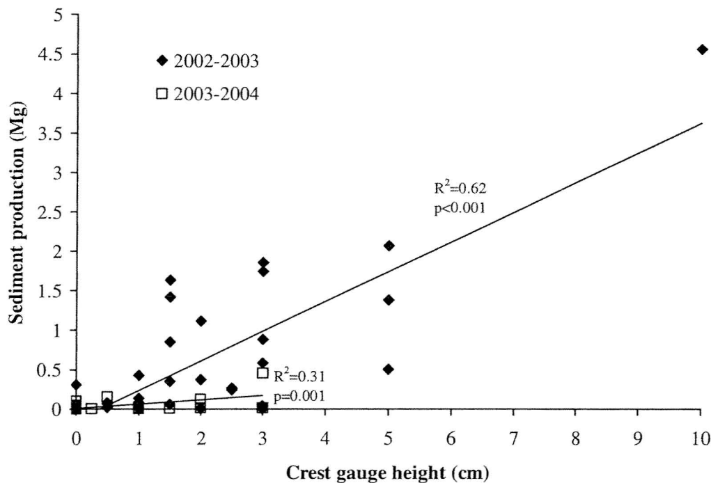
Figure 14. Sediment production versus crest gauge height for the 2002-2003 and 2003-2004 wet seasons.
