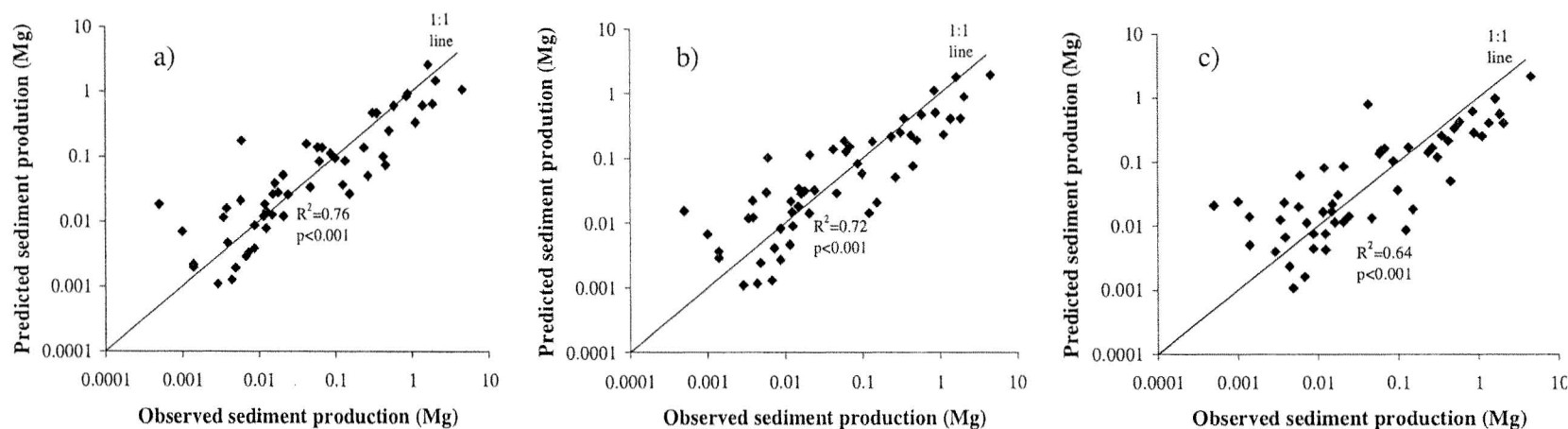
Figure 17. Predicted versus observed sediment production for: a) complete model; b) 4-parameter model; and c) 3-parameter model.
