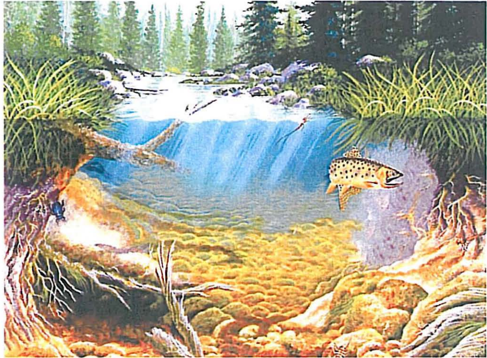
Figure 22 —The combination of greatest water velocity and highest rooting strength and concentration in healthy riparian systems creates undercut banks, which in turn provide a cooling effect in the water column as well as other special habitat features beneficial to many aquatic organisms.
