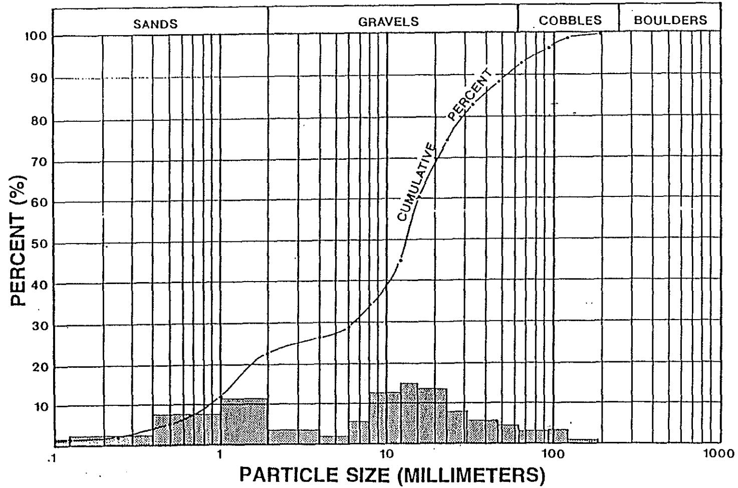
Figure 7. Channel material sizes showing cumulative and percent distributions.
