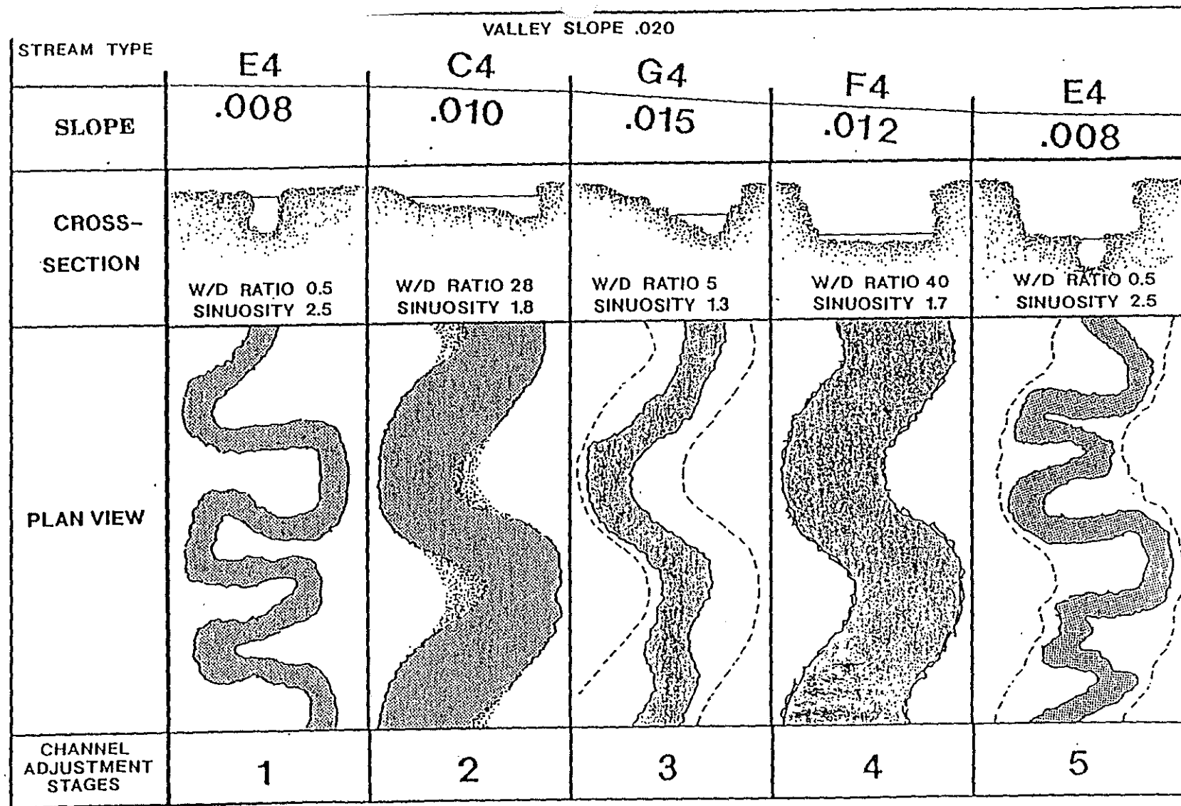
Figure 9. Evolutionary stages of channel adjustment.
