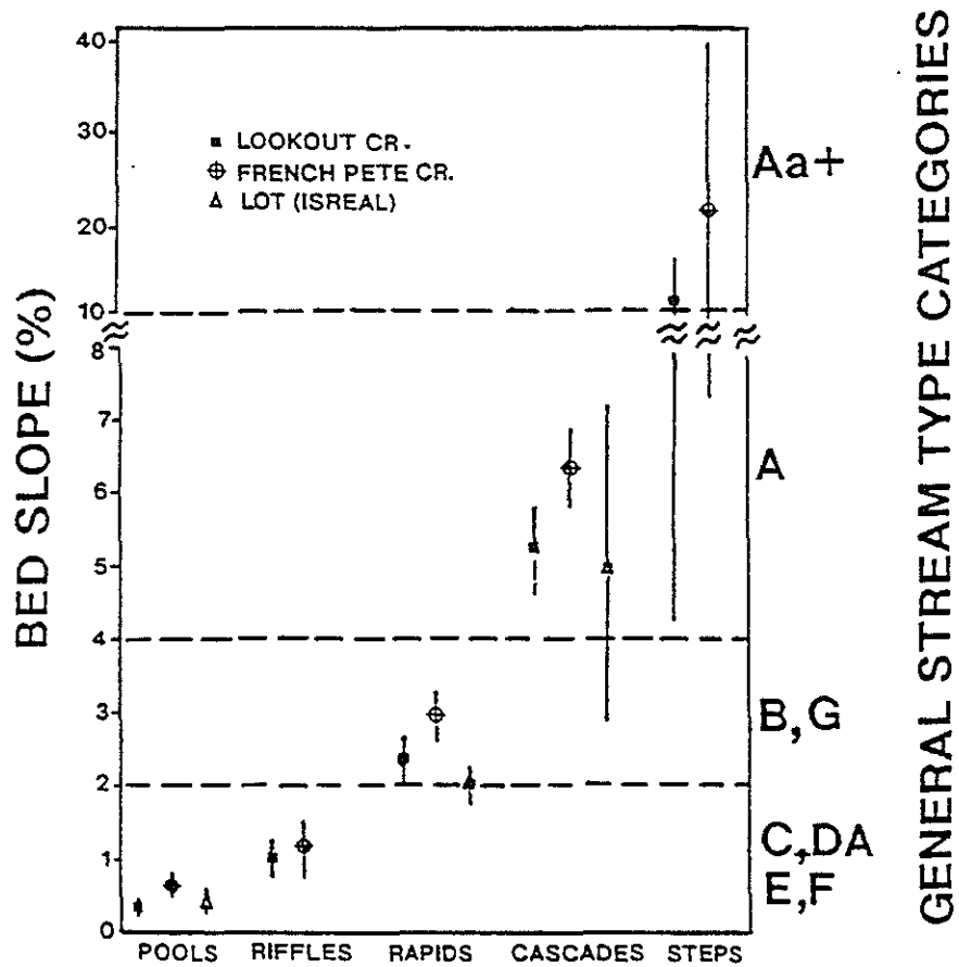
Figure 2. Relationship of bed slope to bed forms (from Grant et al., 1990) for various stream types.
