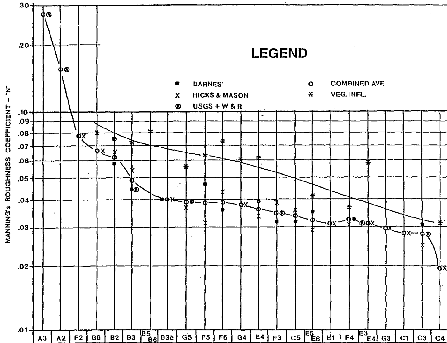
Figure 10. Bankfull stage roughness coefficients ("N" values) by stream type for 140 streams from the United States and New Zealand.
